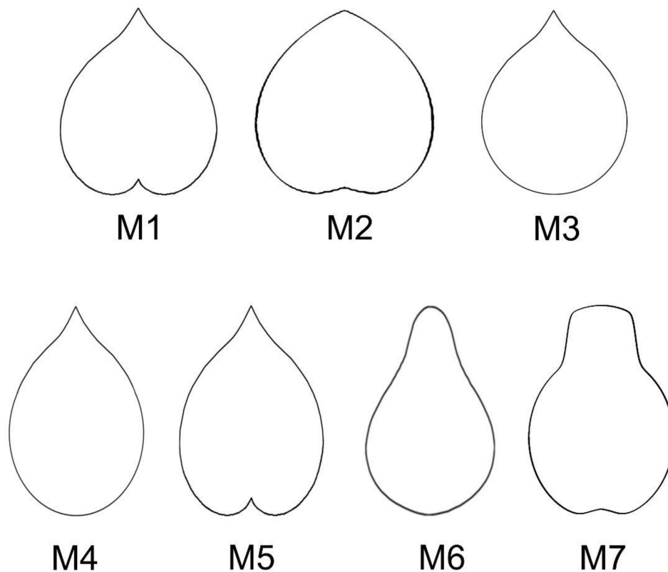
Figure 2. Geometric models for the quantification of shape in seeds of the Vitaceae: (M1) The fourth heart curve of Weisstein [31]. (M2) A rounded heart curve modified from M1. (M3) The water drop, obtained from M1, adapting the basis in the heart curve to a circumference overlapping the maximum width of the curve. (M4) Obtained by scaling M3 in the y-axis by a factor of 123/100. (M5) Obtained by scaling M1 in the y-axis by a factor of 123/100. (M6) Fibonacci’s pear, obtained by scaling the pear curve of Weisstein [30] with r = 2 in the y-axis by a factor equal to the Golden Ratio \Phi . (M7) Derived from an ellipse.
