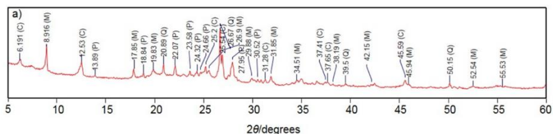
Figure 2: XRPD analysis of raw clayey diatomite (Q: quartz, M: muscovite, C: chlorite, P: plagioclase).
