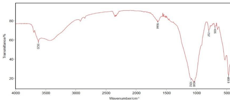
Figure 3: IR spectrum of raw clayey diatomite.
