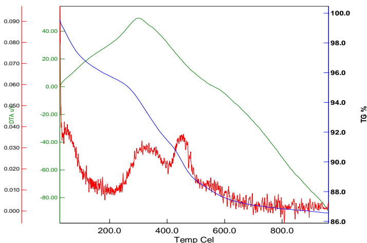
Figure 6: DTA/TGA of raw clayey diatomite.
