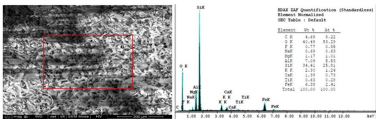
Figure 5: SEM-EDX spectrum of raw clayey diatomite.
