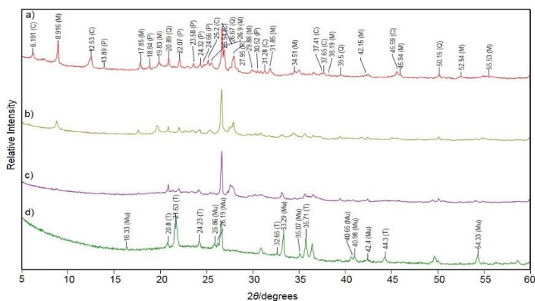
Figure 7: XRPD analysis of raw clayey diatomite (a), and thermally treated sample for a period of 1 hour at 800°C for a period of 1 hour, (b) at 1000°C for a period of 1 hour, (c) and at 1200°C for a period of 1 hour (d).
