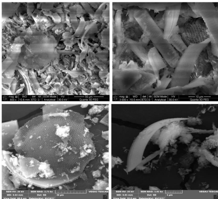
Figure 4: SEM pictures of raw clayey diatomite composed of various microreliefs of biogenetic origin with various forms (globular or tubes) with many pores ranging from 350 – 650 nm.
