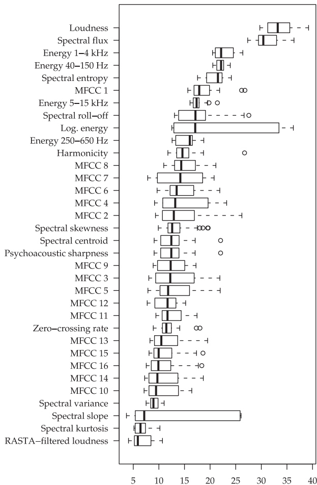
Figure 1. Audio LLD relevance: Absolute values of t-statistics (non-violent vs. violent) for groups of LLDs, across functionals applied to two second non-overlapping segments. 26/45 functionals selected by highest t-statistic per LLD group. doi:10.1371/journal.pone.0078506.g001
