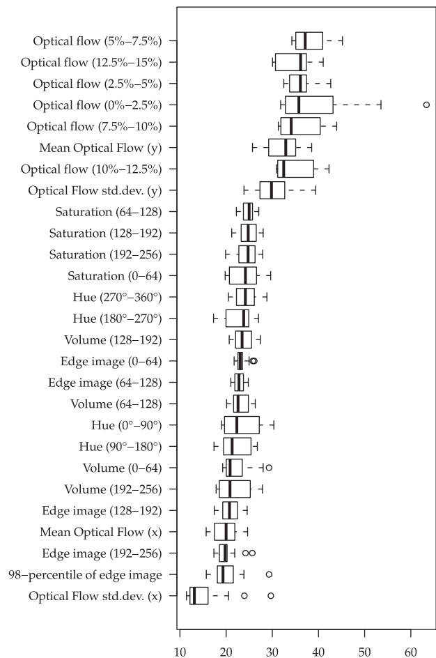
Figure 2. Video LLD relevance: Absolute values of t-statistics (non-violent vs. violent) for groups of LLDs, across functionals applied to two second non-overlapping segments. 26/45 functionals selected by highest t-statistic per LLD group. doi:10.1371/journal.pone.0078506.g002
