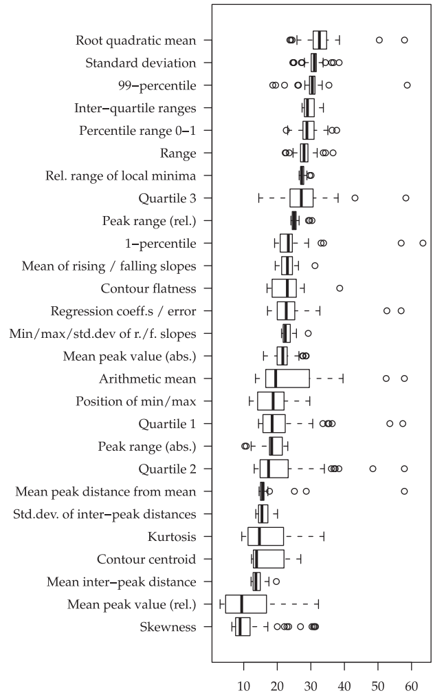
Figure 4. Functional Relevance for video: Absolute values of t-statistics (non-violent vs. violent) for groups of functionals applied to two second non-overlapping segments, across audio/video LLDs. 18/37 (audio) and 48/97 (video) LLDs selected by highest t-statistic per functional group. doi:10.1371/journal.pone.0078506.g004
