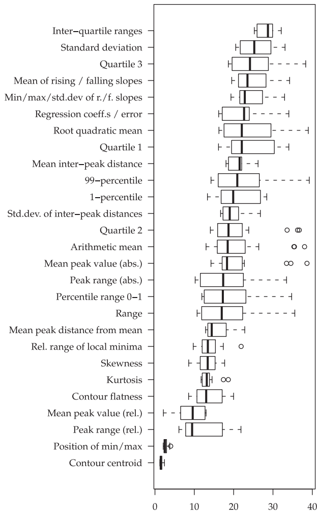
Figure 3. Functional Relevance for audio: Absolute values of t-statistics (non-violent vs. violent) for groups of functionals applied to two second non-overlapping segments, across audio/video LLDs. 18/37 (audio) and 48/97 (video) LLDs selected by highest t-statistic per functional group. doi:10.1371/journal.pone.0078506.g003
