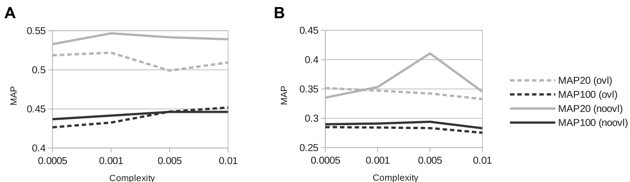
Figure 5. Segmentation and classifier training: Influence of SVM complexity and overlapping (ovl, 50%) vs. non-overlapping (noovl) shot sub-windows on (shot level) mean average precision (MAP), measured on the development set of the MediaEval 2012 Affect Task Data Set. Sub-window size 2 seconds. A: audio, B: video. doi:10.1371/journal.pone.0078506.g005
