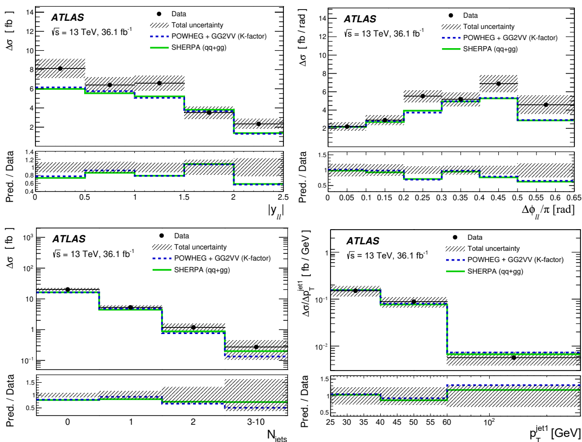
Figure 7. The measured differential cross-sections for |y_{\ell\ell}| (top left), \Delta\phi_{\ell\ell} (top right), N_{\text{jets}} (bottom left), and p_{\text{T}}^{\text{jet}1} (bottom right) in the fiducial region. The hashed bands in light grey give the total uncertainty. Also shown are the predictions as obtained from SHERPA (solid line) and POWHEG+GG2VV (dashed line) with higher-order K -factors, as described in section 3. The last bin in the distributions of N_{\text{jets}} and p_{\text{T}}^{\text{jet}1} is shown using a different x -axis scale for better visualisation.
