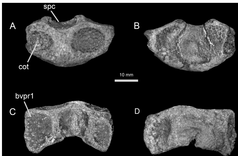
FIG. 5. AMNH FF 22425, Late Cretaceous, Ramanessin Brook, NJ; isolated first vertebra referred to Cretasquatina : A , anterior view; B , posterior view; C , dorsal view; D , ventral view. The centrum is visible posteriorly but does not emerge onto the anterior surface of the element. Large paired concavities of the cranial-vertebral articulation are present anteriorly. Note also the large size of cartilage tesserae covering surfaces of the arcualia and cotyli (compare with figs. 3, 4).
