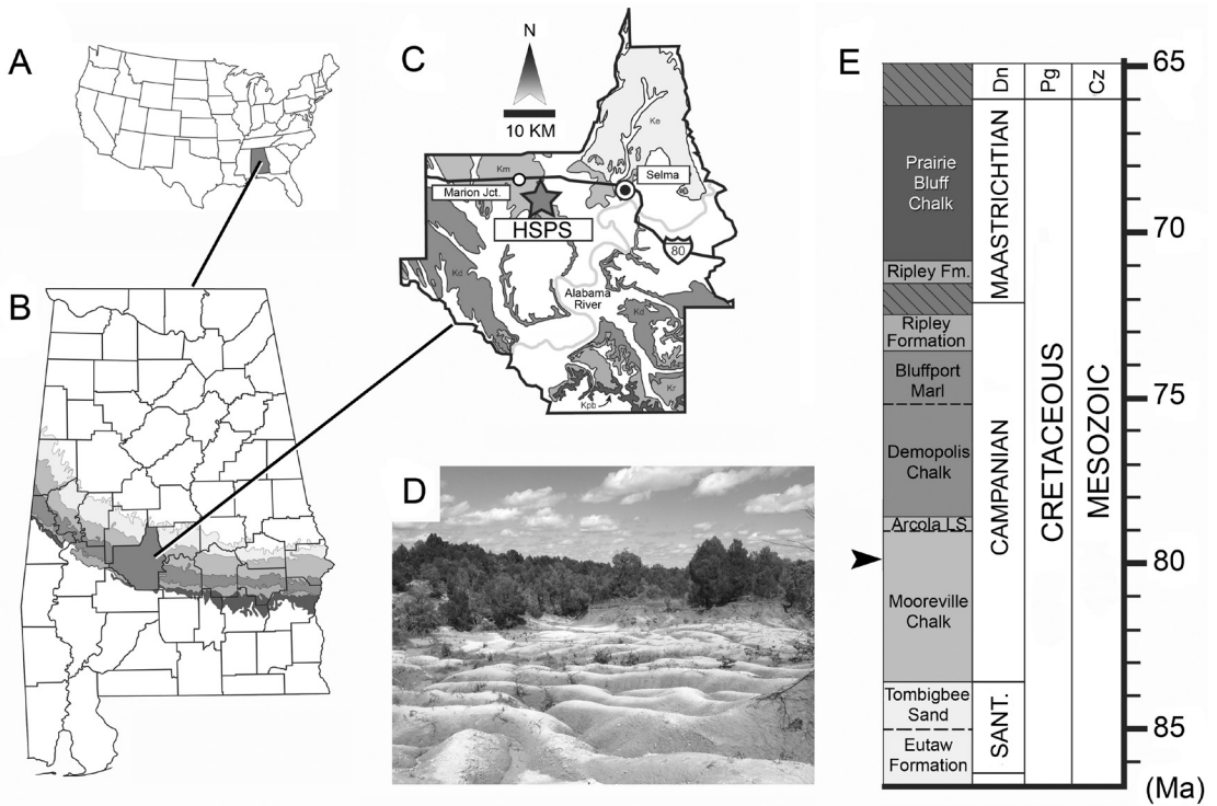
FIG. 1. Locality and stratigraphic information. A , location of Alabama within continental United States (no scale); B , location of Dallas County within Alabama (no scale); C , location (starred) of Harrell Station Paleontological Station (HSPS); D , general view of the HSPS site; E , Upper Cretaceous geologic section for western Alabama showing the approximate exposure level at HSPS (arrow).
