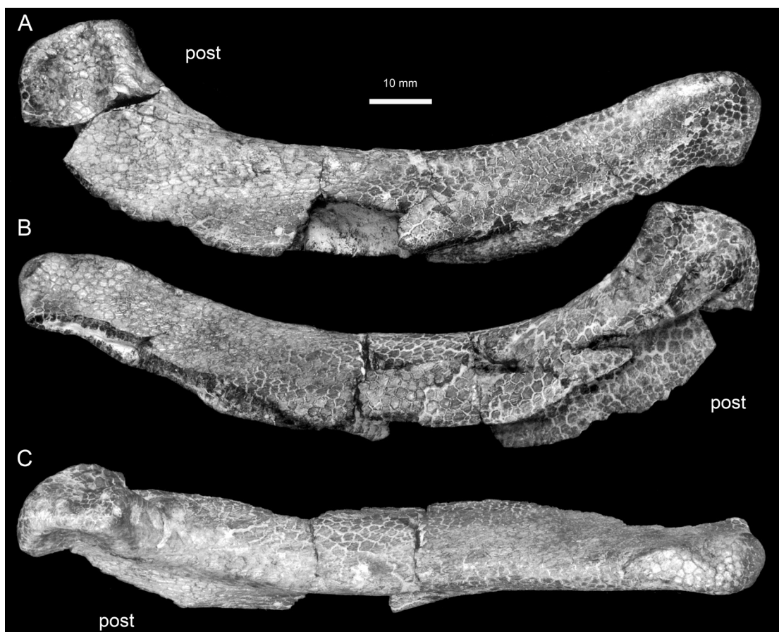
FIG. 10. ALMNH 2792-B, three views of ceratohyal referred here to Cretasquatina americana . Anterior to right in A and C, to left in B. Again, note the extremely coarse texture of tesserae.
