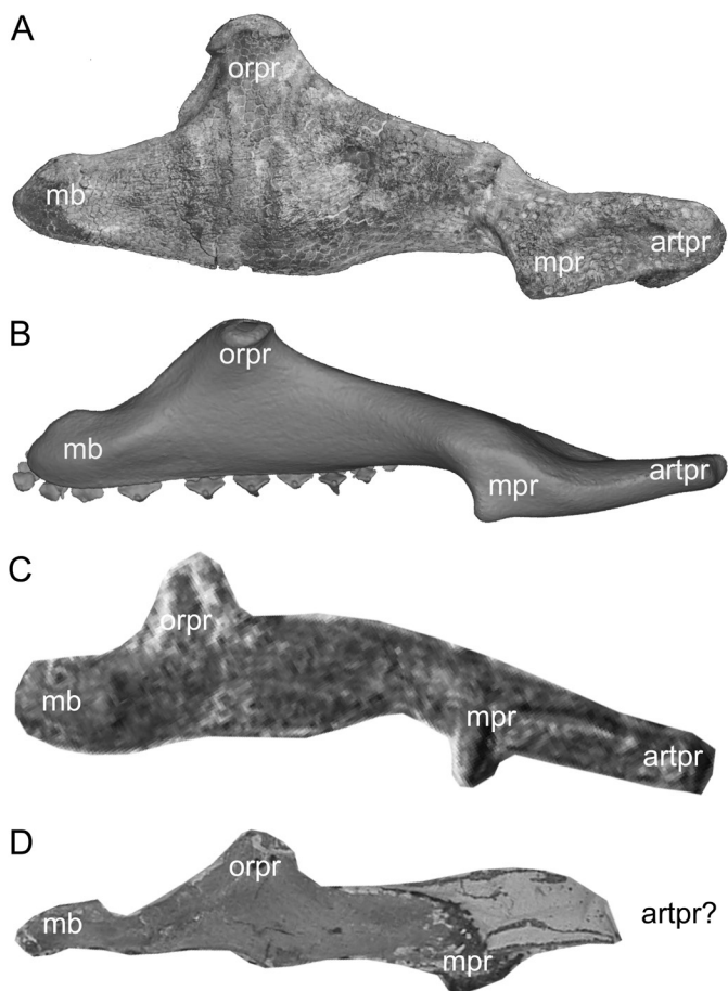
FIG. 12. Comparison of palatoquadrate proportions in four different squatinids, all in lateral view, anterior to left. See text for discussion. A , ALMNH 2792-A (see fig. 6), referred here to Cretasquatina americana ; B , modern Squatina nebulosa , AMNH 258172 (see fig. 9); C , Pseudorhina acanthoderma (adapted after Vaz and Carvalho, 2013; fig.6); D , Cretascyllium cranei (adapted from a photograph of the holotype specimen, Booth Museum BNB 007329/007330, courtesy of C.J. Underwood).
