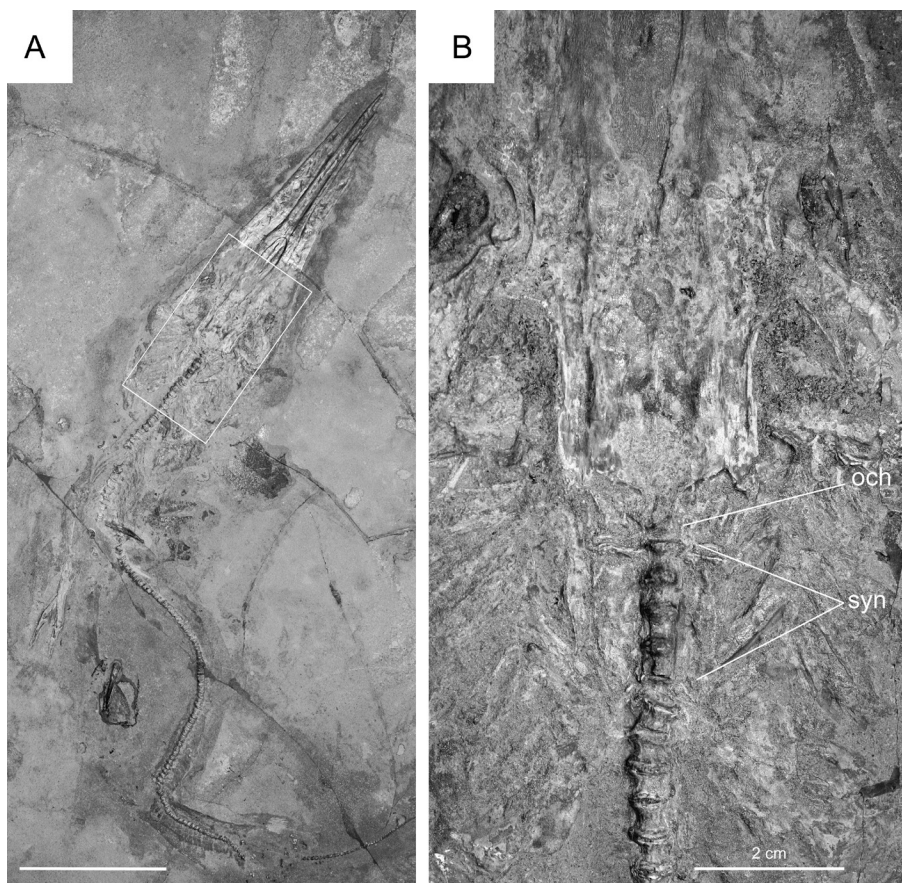
FIG. 14. An undescribed Early Jurassic batomorph skeleton from Holzmaden (SMNS 52666): A , general view of the specimen in dorsal view; white rectangle indicates region shown in B (scale bar = 10 cm); B , detail of cranio-vertebral articulation, showing the existence of an occipital hemicentrum and a short synarcual with four unreduced anterior vertebral centra. In all modern batoids, the occipital hemicentrum and the anterior-most centra within the synarcual are absent and the cranio-vertebral joint is formed entirely by fused dorsal and ventral arcualia of the vertebral column (synarcual cartilage). Thus, reduction or absence of the anterior spool in the first free centrum of squatiniforms is probably independent of the condition in batomorphs.
