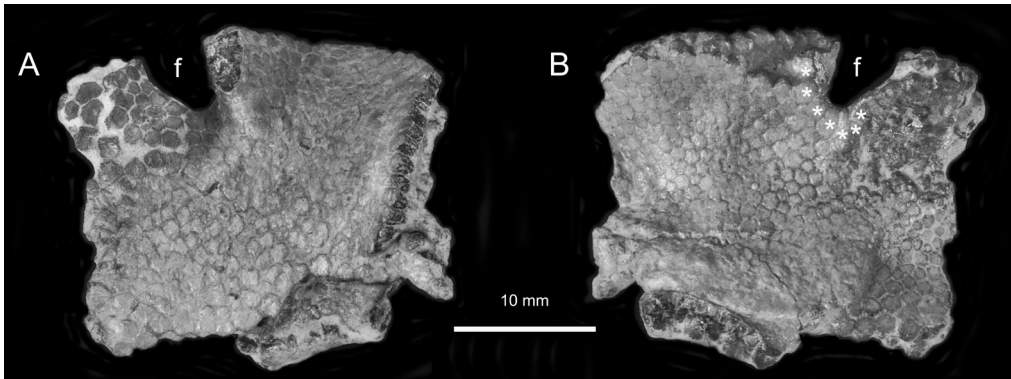
FIG. 11. ALMNH 2792-D, fragment of braincase, possibly part of the postorbital process. Small white stars in B mark a series of voussoir tesserae lining the outer margin of a foramen.
