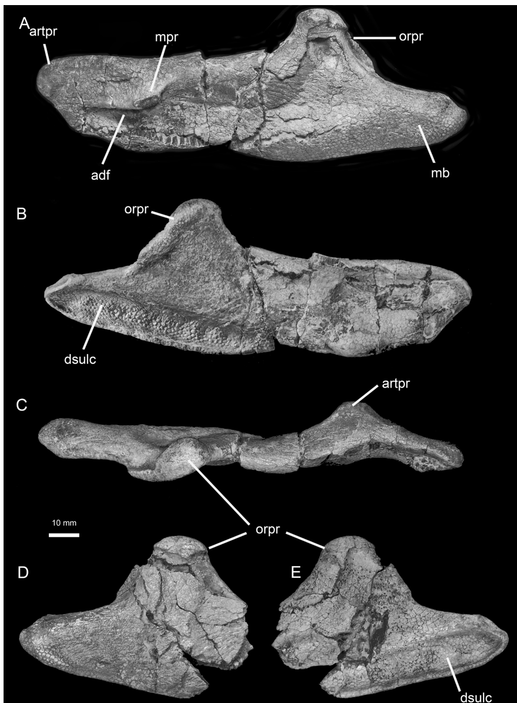
FIG. 8. Additional palatoquadrate referred here to Cretasquatina americana : A–C, ALMNH 1040-A, almost complete right palatoquadrate approximately 143 mm long. A , lateral view, anterior to right; B , mesial view, anterior to left; C , dorsal view, anterior to left; D , E , ALMNH 1040-B, anterior part of left palatoquadrate matching 1040-A in size and representing its antimere (the two were collected together).
