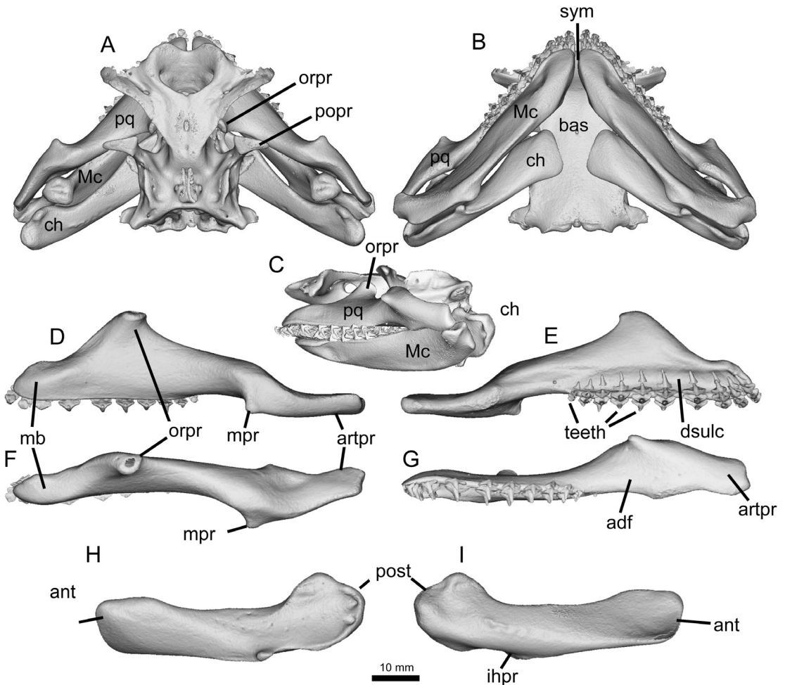
FIG. 9. Head skeleton of modern Squatina nebulosa , AMNH 258172 (juvenile female 405 mm TL), images from scanned specimen segmented by C. Crawford: A , cranium, jaws and ceratohyals in dorsal view, anterior to top; B , same in ventral view; C , same in lateral view, left side, anterior to left; D , left palatoquadrate in lateral view, anterior to left; E , same in mesial view, anterior to right; F , same in dorsal view, anterior to left; G , same in ventral view, anterior to left; H , left ceratohyal in lateral view; I , same in mesial view.
