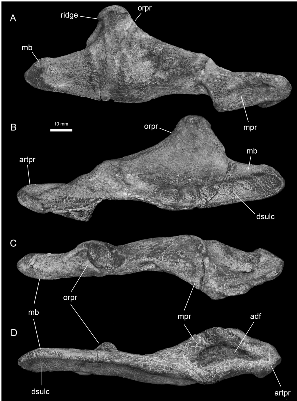
FIG. 7. ALMNH 2792-A, almost complete left palatoquadrate, referred here to Cretasquatina americana : A , lateral view, anterior to left; B , mesial view, anterior to right; C , dorsal view, anterior to left; D , ventral view, anterior to left. Note extremely large cartilage tesserae (some with zigzag intertesseral contacts), especially in the center of the lateral surface of the palatoquadrate main bar in A .
