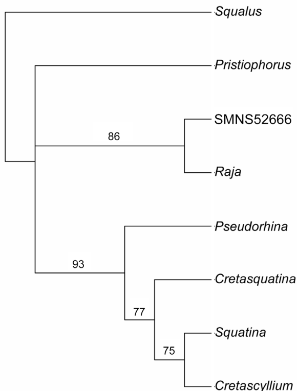
FIG. 13. Strict consensus of two equally parsimonious trees, inferred from PAUP*. Numbers at nodes are bootstrap support values. Cretasquatina is inferred to lie on the squatinid stem above Pseudorhina . Cretascyllium is resolved in this analysis as the closest extinct taxon to modern Squatina .
