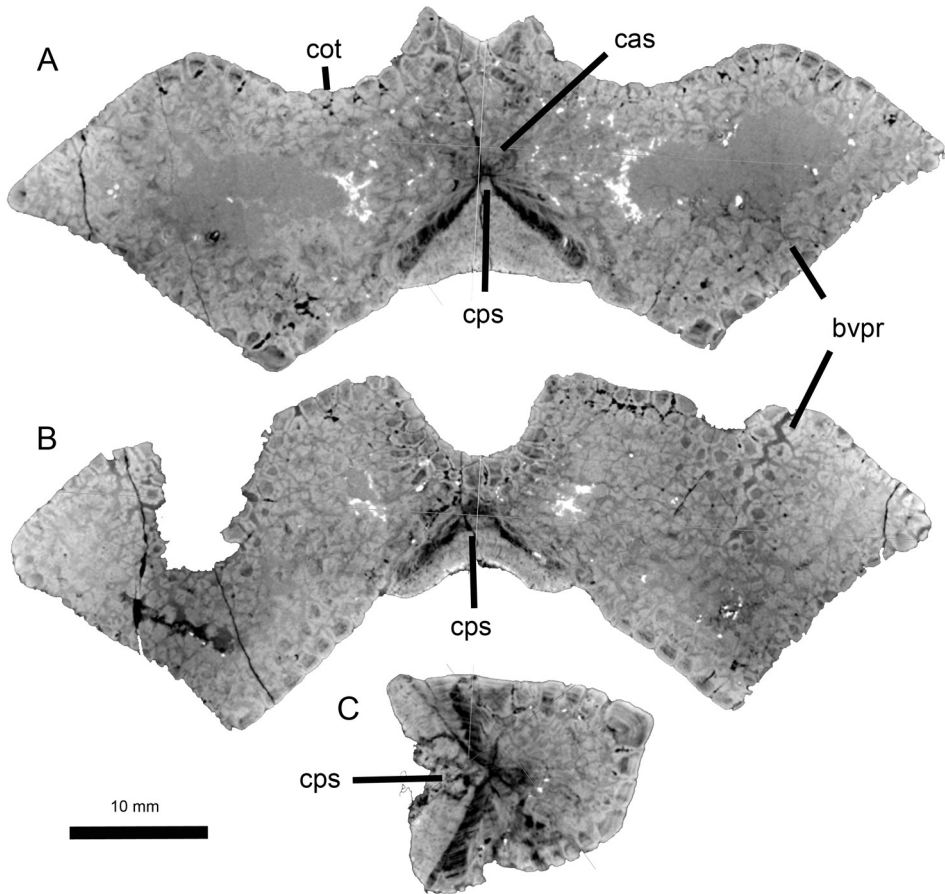
FIG. 4. Cretasquatina americana . Holotype, ALMNH 2792-C, computerized tomography images of slices through first vertebra: A , horizontal section through middle of centrum just above median process; B , slightly higher horizontal section clipping anterior part of spinal canal; C , midsagittal section through vertebral centrum. Note the extremely large size of individual tesserae, especially rows of “voussoir” tesserae along margins between adjacent surfaces.
