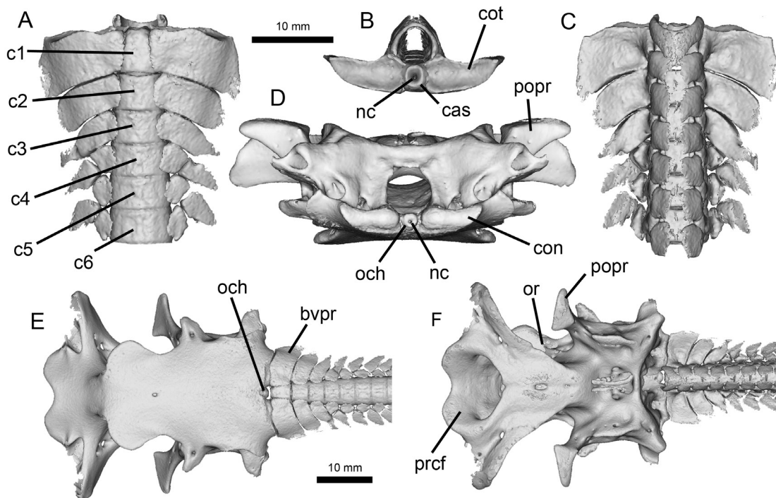
FIG. 6. Squatina nebulosa , AMNH 258172. Views of the cranium and anterior part of vertebral column, imaged from tomographic scan by C. Crawford: A , ventral view of first six vertebral centra and associated basiventrals, anterior to top; B , anterior view of first vertebral element; C , dorsal view of A ; D , posterior view of cranium; E , ventral view of cranium and vertebral centra (anterior to left); F , dorsal view of same. Upper scale bar for A – D ; lower scale bar for E and F only.
