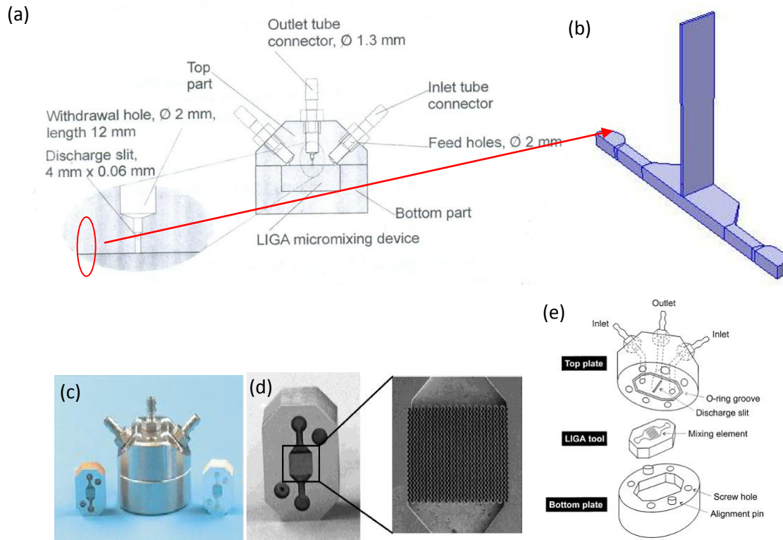
Figure 1: Standard Slit Interdigital Micro Mixer [12] (a) The schematic presentation of the assembly in the micro mixing system,-(Institut fur Mikrotechnik Mainz GmbH) (b) The model structure of SSIMM in COMSOL Multiphysics (c) The photograph of SSIMM (d) The mixing element (e) Explosion drawing of the SSIMM
