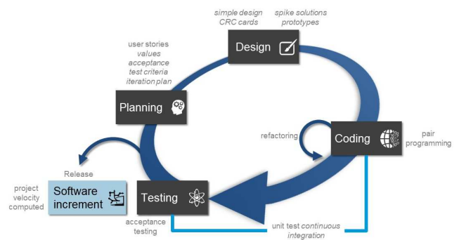
Fig. 5 XP Workflow
