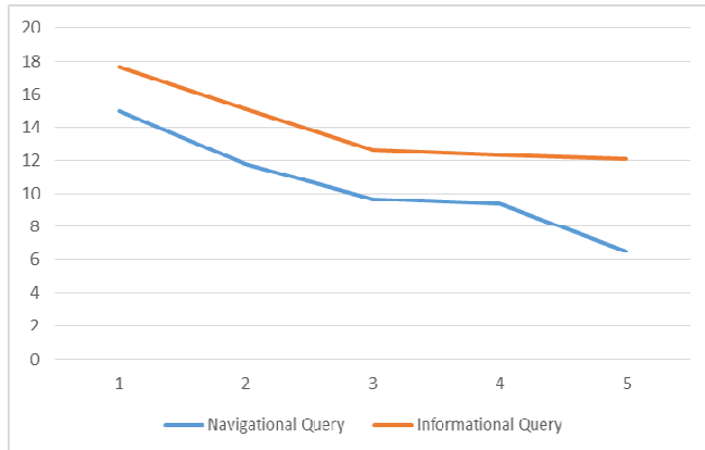
Fig. 1 Average document length of Navigational and Information Queries obtained from the Okapi BM25 mathematic model
