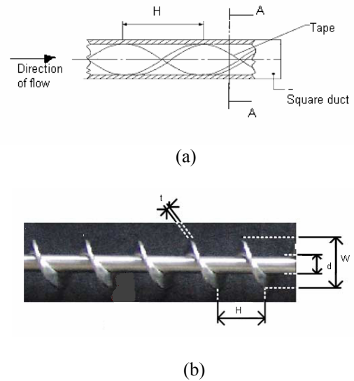
Fig. 1 Schematic diagram of different inserts, (a) for twisted tape, (b) for Screw tape insert
