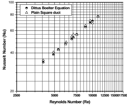
Fig. 4 Data verification of Nusselt number of plain duct
