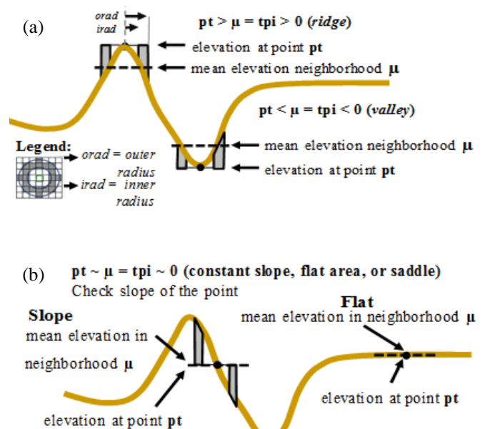
Fig. 3 Illustration for calculating topographic position index[15]
