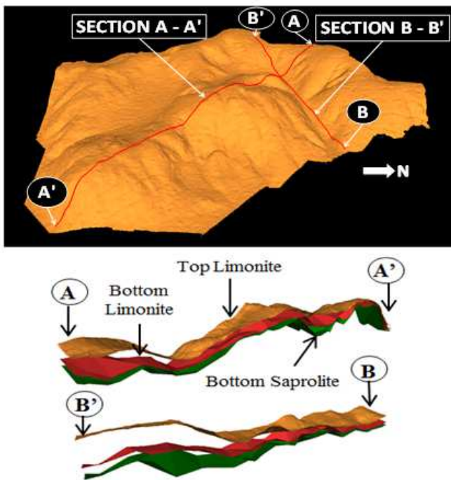
Fig. 8 Spatial distribution of interpolated layer thickness from the borehole dataset which represented surface topographic condition (exaggeration z=2 )
