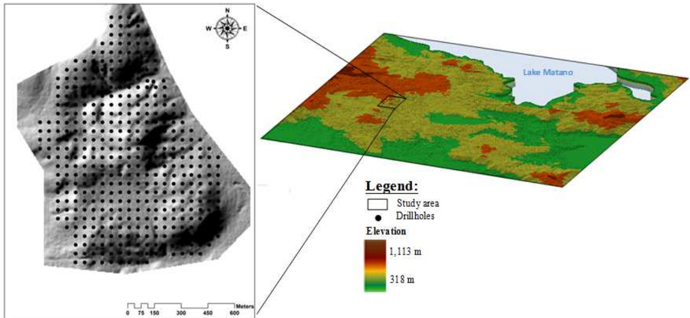
Fig. 5 Topography of ultramafic terrain in Sorowako including study area which supported by 50m drill spacing
