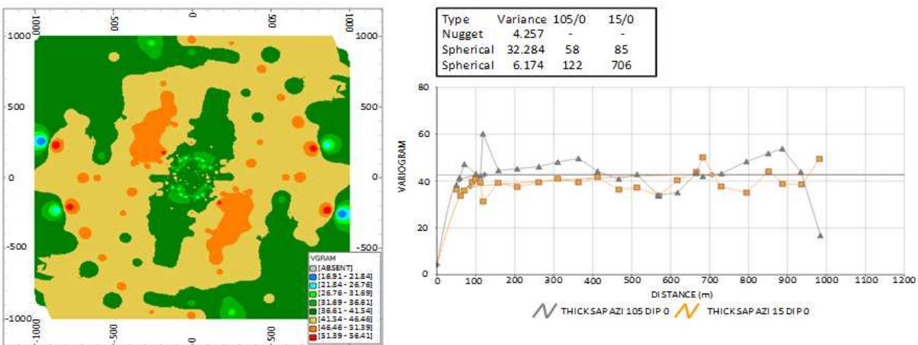
Fig. 13 Variogram map of saprolite thickness and semivariogram model along two directions
