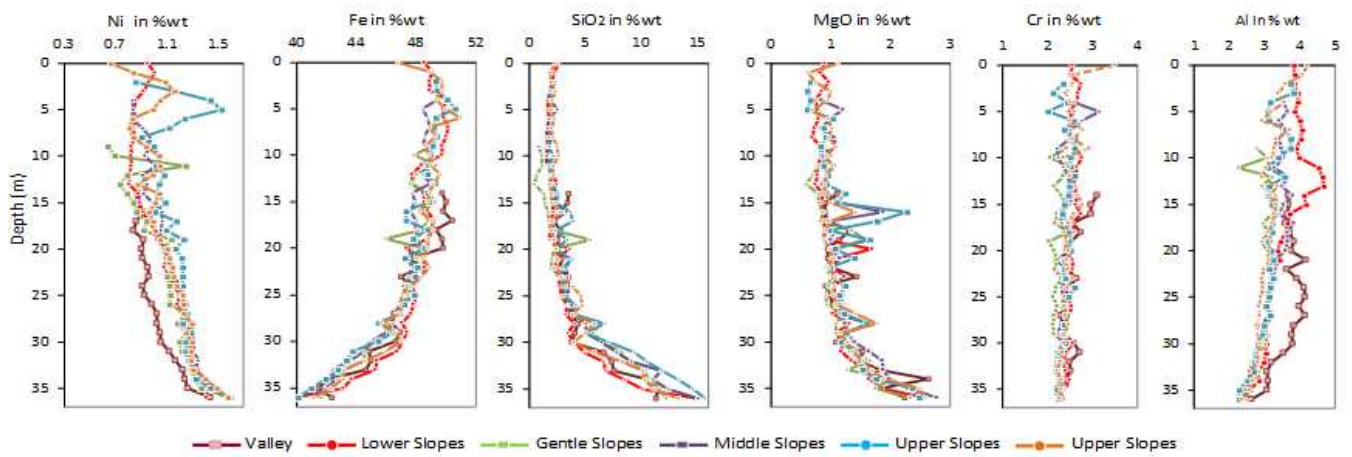
Fig. 14 Composition of Ni, Fe, SiO 2 , MgO, Cr and Al on limonite profile for each slope position category
