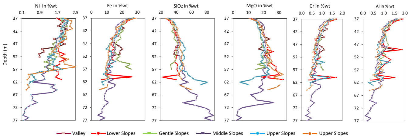
Fig. 15 Composition of Ni, Fe, SiO 2 , MgO, Cr and Al on saprolite profile for each slope position category
