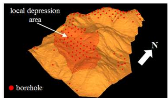
Fig. 11 Detail 3D surface model with the thick limonite distribution, showing local depression area (exaggeration z=2 )
