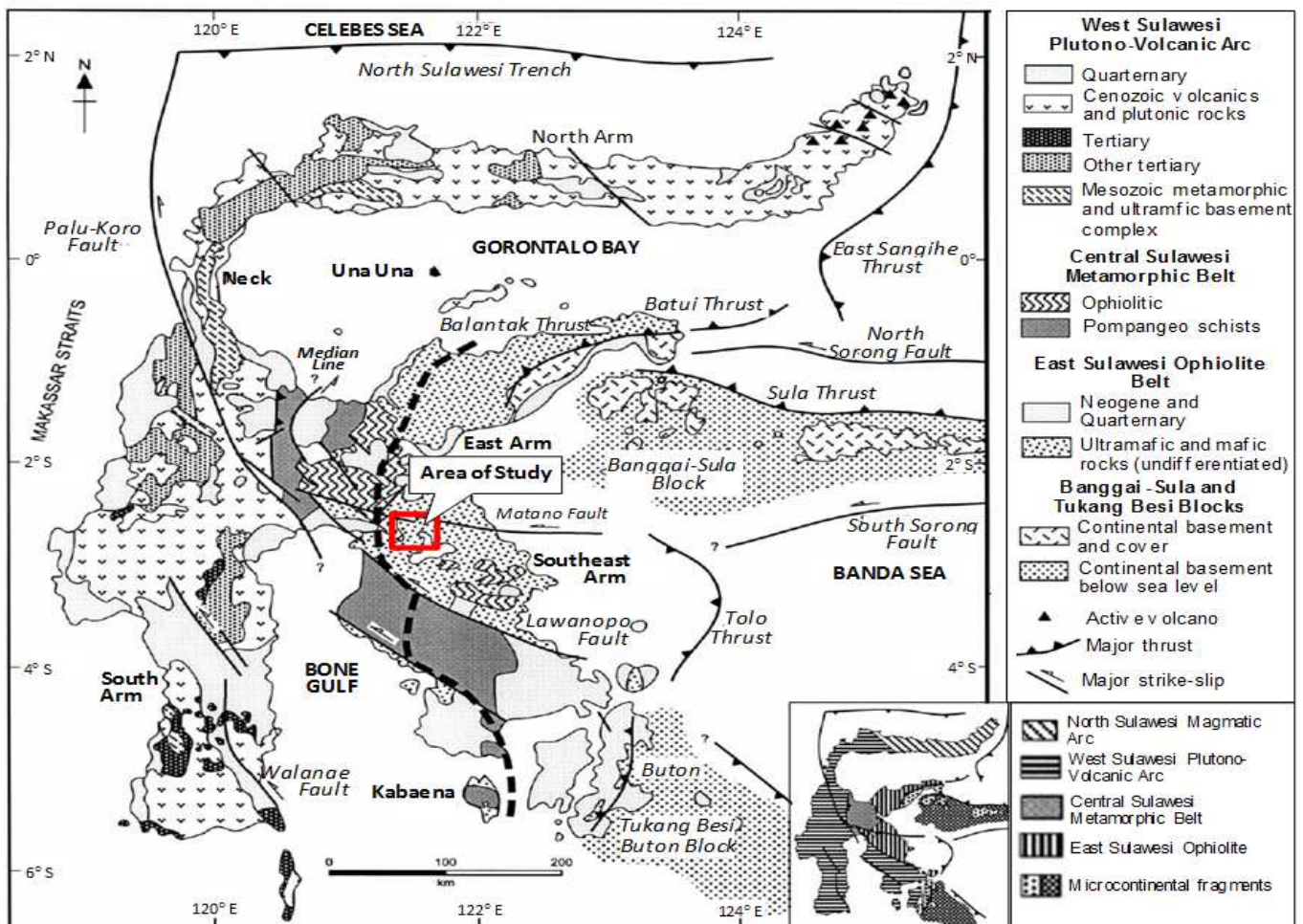
Fig. 1 Regional geology map of Sulawesi with the principle tectonic provinces –inset [9].
