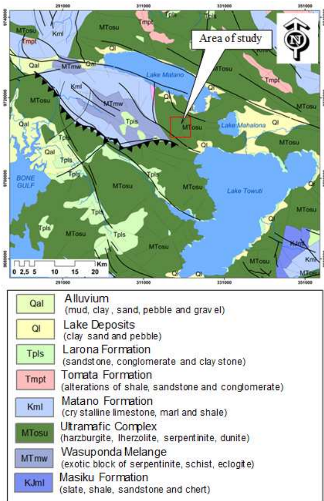
Fig. 2 Local geology of Sorowako and its vicinity[11].
