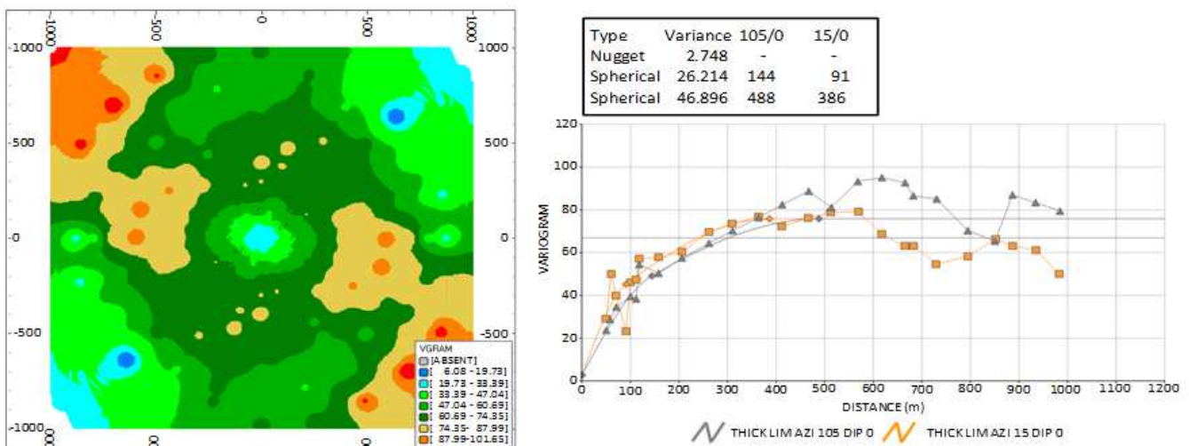
Fig. 12 Variogram map of limonite thickness and semivariogram model along two directions
