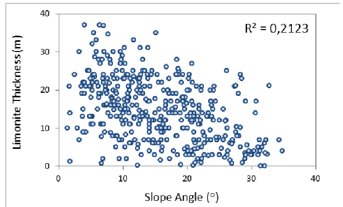
Fig. 9 Scatterplots show the relationship between topographic slope angle and limonite thickness
