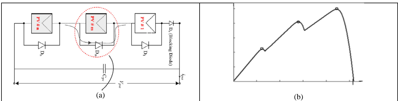
Fig. 5 (a) PV Array of Three PV Modules in a Series Configuration, (b) P - V Characteristic of PV Array
