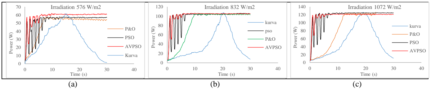
Fig. 10 Experimental Result of Each Method; a) at low irradiation; b) at medium irradiation; c) at high irradiation
