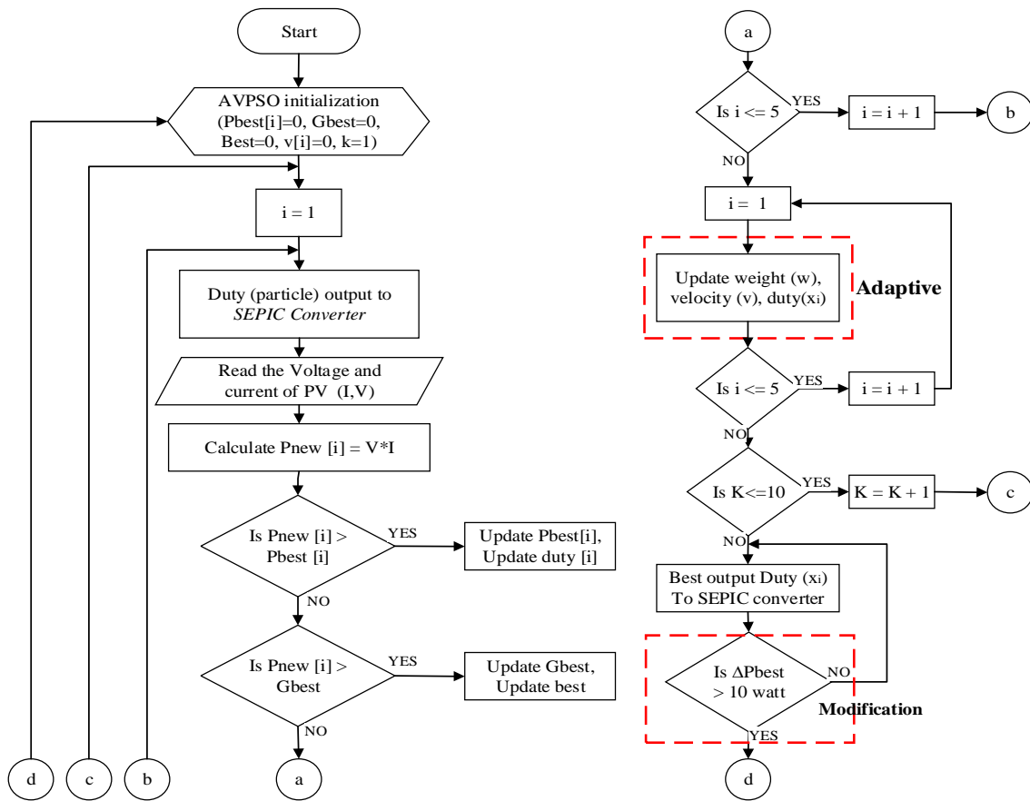
Fig. 7 Flowchart of the Proposed AVPSO Algorithm
