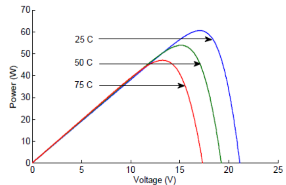
Fig. 3 P-V curves at Several Temperature Levels
