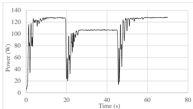
Fig. 15. Power Tracking Curve when There is a Change Power Value
