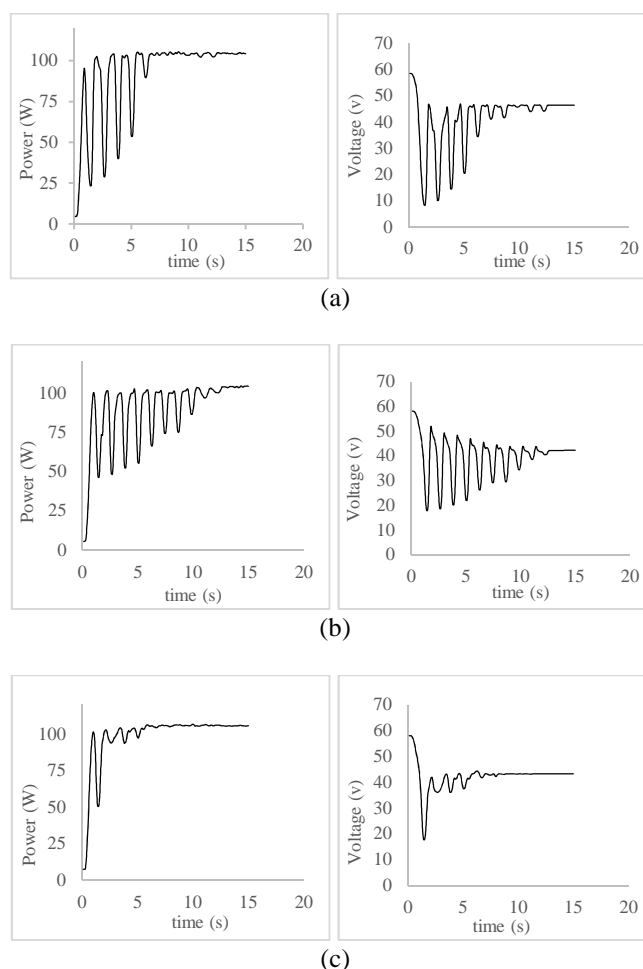
Fig. 13 Power and Voltage Tracking Curves of Several Methods (a) Conventional PSO; (b) Modified PSO; (c) Proposed AVPSO
