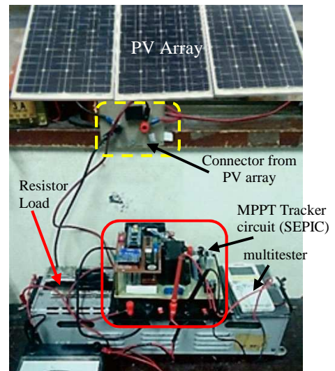
Fig. 9 Hardware Experiment Configuration
