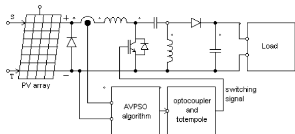
Fig. 6 Block Diagram of the prototype Based MPPT Scheme
