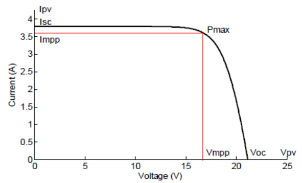
Fig. 1 I-V curve of PV Module
