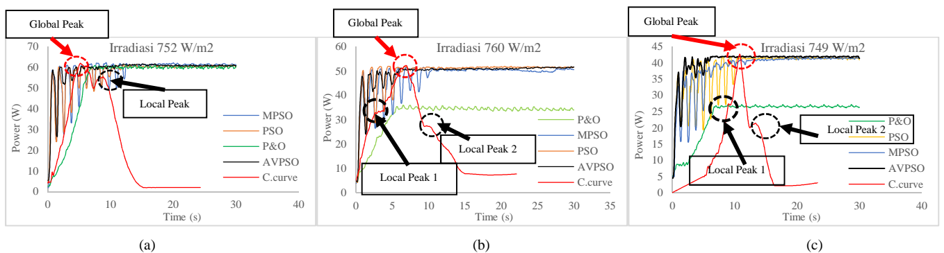
Fig. 12 Comparison the Experimental Result of each MPPT Method Under NUIC(a) the result at pattern 1;(b) the result at pattern 2;(c) the result at pattern 3
