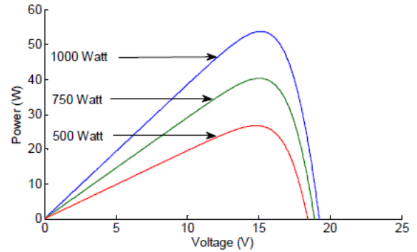
Fig. 2 P-V Curves at Several Irradiance Levels
