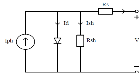
Fig. 4 Equivalent Circuit of PV Module
