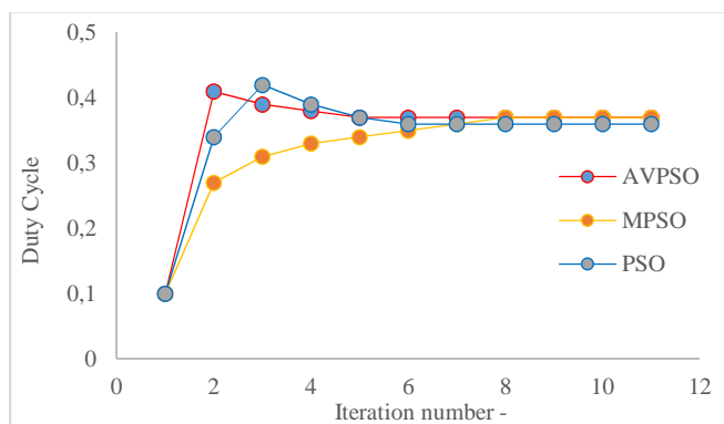
Fig. 14 Movement of Particles in Each Iteration
