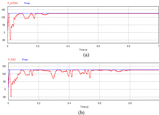
Fig. 8 Power Waveform (a) the AVPSO Algorithm, (b) Original PSO
