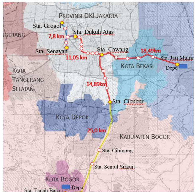
Fig. 2 Layout of LRT Jabodebek
