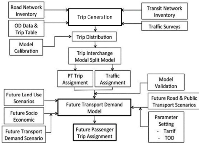
Fig. 4 Flowchart of the four-stage method (FSM)
