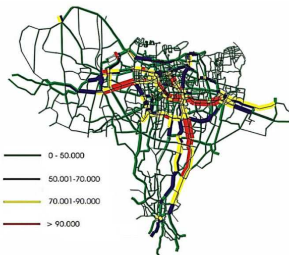
Fig. 14 The forecasted travel demand model for the Greater Jakarta area in post-construction stage (2020)
