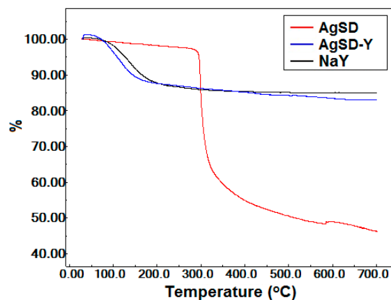
Figure 5. Curve of AgSD, AgSD-Y and NaY samples.
