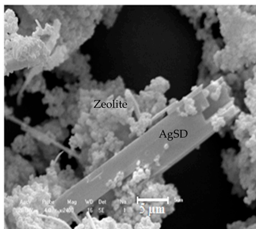
Figure 2. SEM micrograph of AgSD-Y zeolite (magnification of 2400×).
