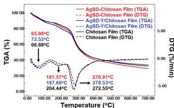
Figure 10. curve for the Chitosan film and AgSD/Chitosan film and AgSD-Y/Chitosan film.
