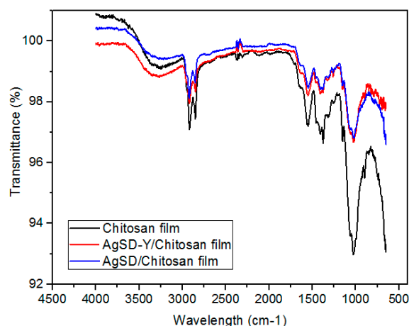
Figure 11. Infrared spectrum of the chitosan film, AgSD-Y/Chitosan film and AgSD/Chitosan film.
