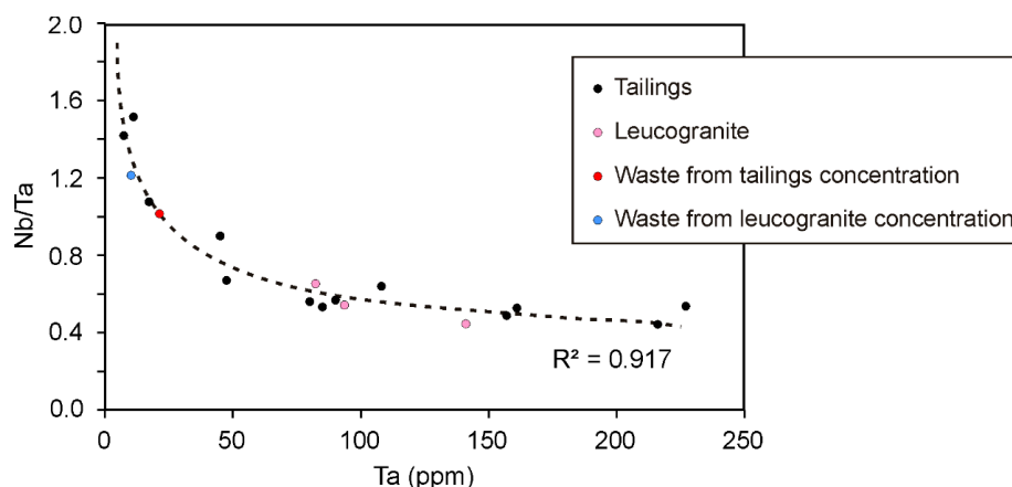
Figure 5. Nb/Ta ratio vs. the Ta content from Penouta materials.
