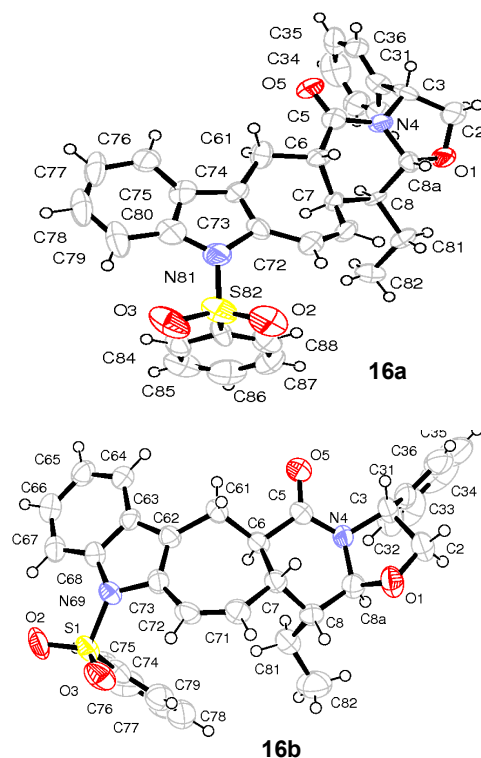
FIGURE 2. X-ray crystal structure of pentacycles 16a and 16b .
