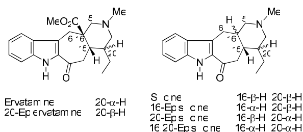
FIGURE 1. Representative alkaloids of the ervatamine-silicine group.
