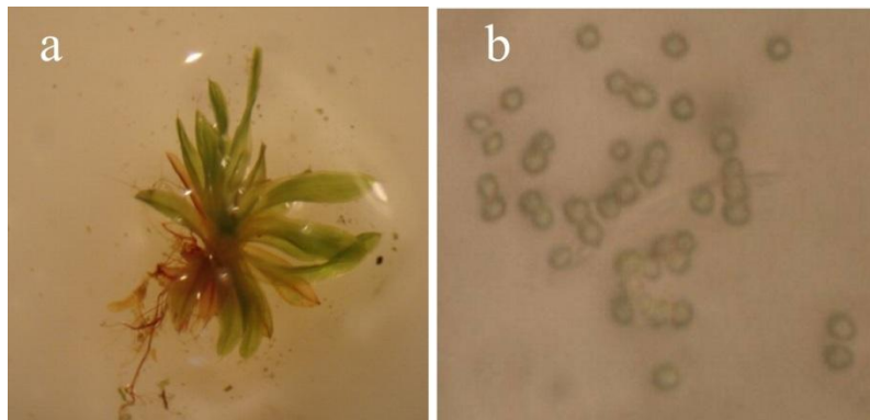
Figure 2: OM image of the green biofilm samples. a) Hennediella sp.; b) Synechocystis sp.
