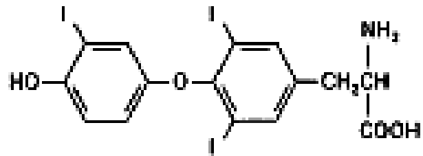
3, 5, 3'-triiodothyronine (T3)
