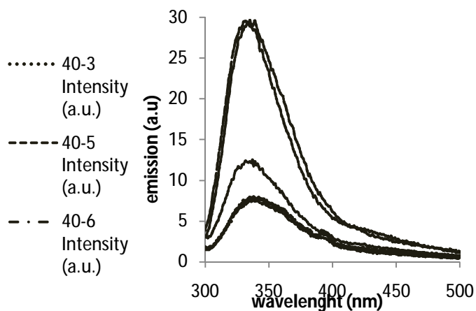
Fig. 4. Fluorescence spectra of 40 µg gramicidin at the presence of copper ions (40ga-cu), absence of copper ions (40ga) and when formulated with 3 (40-3), 5 (40-5) and 6 (40-6) mg/ml of polymer at the presence of copper ions.
