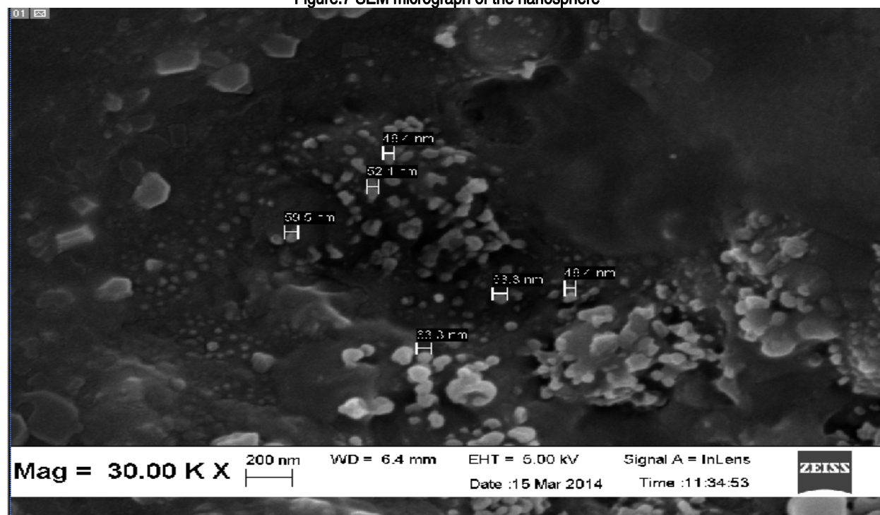
Figure:7 SEM micrograph of the nanosphere
