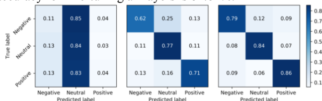
(a) Baseline (b) Finetune fc layers (c) Finetune all layers Fig. 7. The confusion matrix on DEAP.
