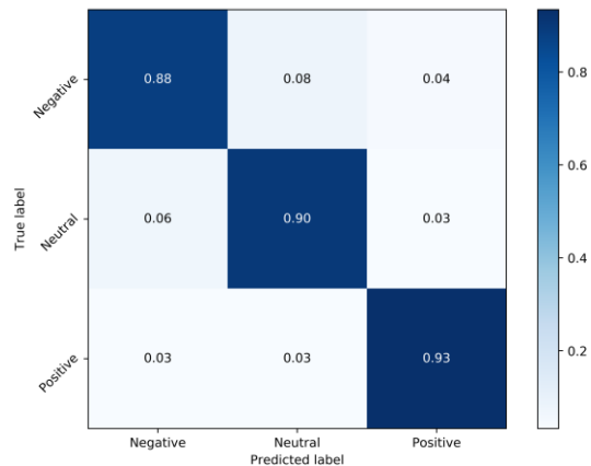
Fig. 5. Confusion matrix on SEED.
