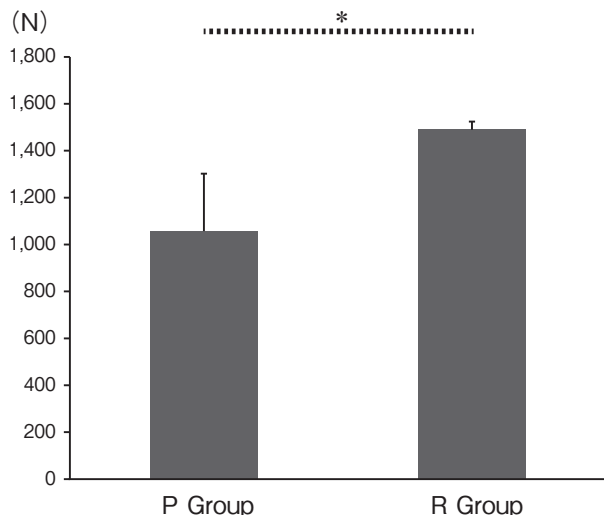
Fig. 3 The mean maximum load. The mean maximum was significantly higher in the R group. P group: Conventional posterior plate fixation. R group: Posterior fixation using spinal instrumentation. *: p -value < 0.05
