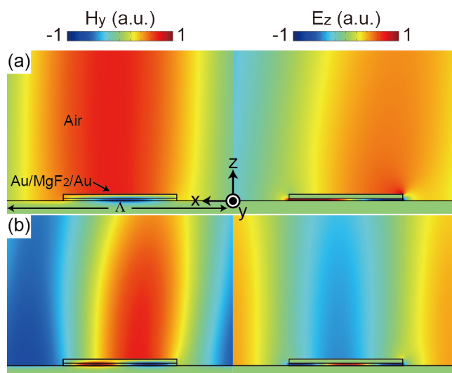
Figure S1 | Mode profiles of SPPs. Corresponding H y and E z distributions of the minor absorption dips at \theta = 80^\circ in Fig. 2(b): (a) at 1690 cm -1 and (b) at 3370 cm -1 .
