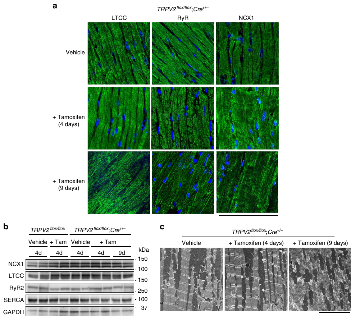
Figure 7 | Expression of \text{Ca}^{2+} handling protein by isolated cardiomyocytes and electron micrographs of myofibrils in TRPV2-deficient hearts.
