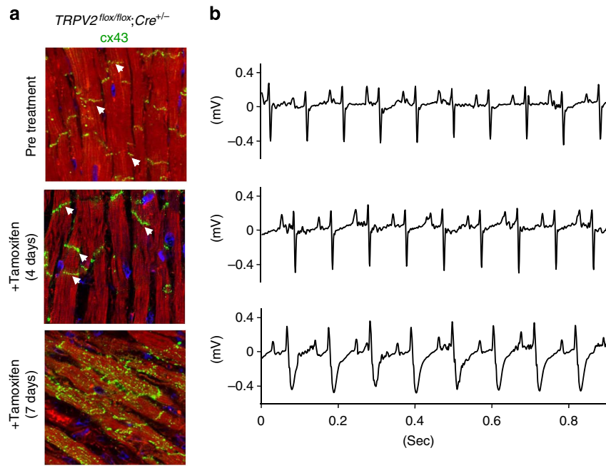
Figure 5 | Cardiac conduction defects after TRPV2 elimination. (a) Change in connexin 43 localization in TRPV2^{flox/flox};Cre^{+/-} hearts after tamoxifen treatment. Scale bar, 100 \mu m. (b) Intraventricular conduction delay after TRPV2 depletion. Electrocardiographs (comparable with lead II) obtained by telemetry.
