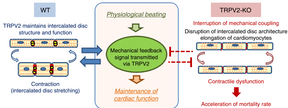
Figure 10 | Role of TRPV2 within the working heart. In wild-type mice, TRPV2 protein (yellow) is located in the intercalated discs (red), which is cyclically stretched and accompanied by cardiac contractions within the working heart. The mechanical feedback signal transmitted via TRPV2 is crucial for the maintenance of cardiomyocytes. TRPV2 ablation leads to the disruption of the intercalated disc architecture (red), and disorganization of sarcomere myofibril proteins at the intercalated discs (orange). These TRPV2-KO myocytes show contractile dysfunction. Therefore, the mortality rate of TRPV2-KO mice is accelerated. Thus, the mechanical feedback signal within the working heart integrates myocyte structure and function, with TRPV2 playing a pivotal role.
