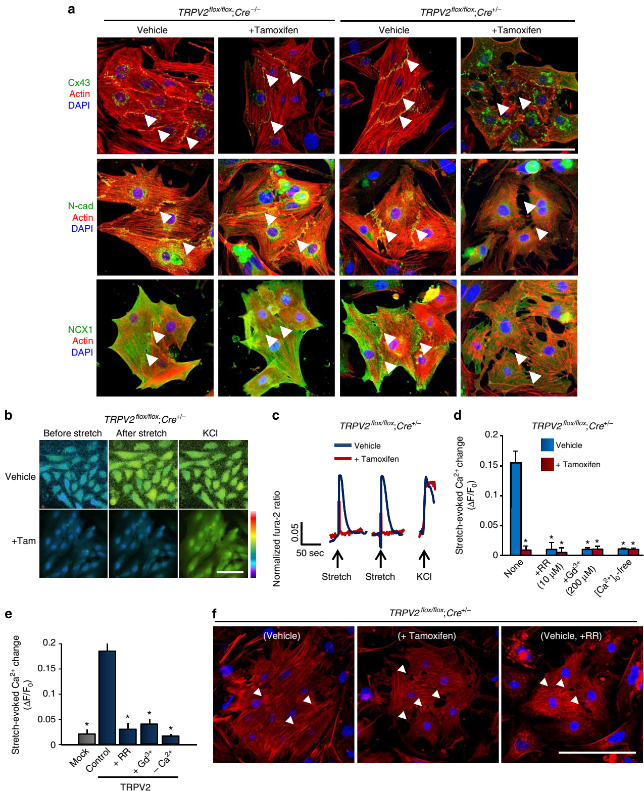
Figure 8 | Impairment of maturation into functional syncytia with synchronously beating cardiomyocytes in TRPV2-deficient newborn mice. (a) Isolated cardiomyocytes from TRPV2 flox/flox ; Cre -/- or TRPV2 flox/flox ; Cre +/- newborn mice. Triple staining with anti-connexin 43 antibody (green), phalloidin (red) and DAPI (blue) in cardiomyocytes (upper panels). Triple staining with anti-N-cadherin antibody (green), phalloidin (red) and DAPI (blue) in cardiomyocytes (middle panels). Triple staining with anti-NCX1 antibody (green), phalloidin (red) and DAPI (blue) in cardiomyocytes (lower panels). Scale bar, 100 μm. (b) Fura-2-imaging of stretch-induced intracellular Ca 2+ dynamics in neonatal cardiomyocytes. Scale bar, 100 μm. (c) Representative trace of stretch-induced intracellular Ca 2+ increase. (d) Effect of mechanosensitive channel inhibitors. Data are means ± s.e.m. *P < 0.01 versus vehicle control (n = 19–44). (e) Stretch-induced Ca 2+ changes in ectopically expressed TRPV2 in HEK293 cells. Data are means ± s.e.m. *P < 0.01 versus control. (n = 23–37) (f) Isolated cardiomyocytes from newborn mice cultured with 10 μM rubidium red. Scale bar, 100 μm. Arrowheads, cell-cell junctions.
