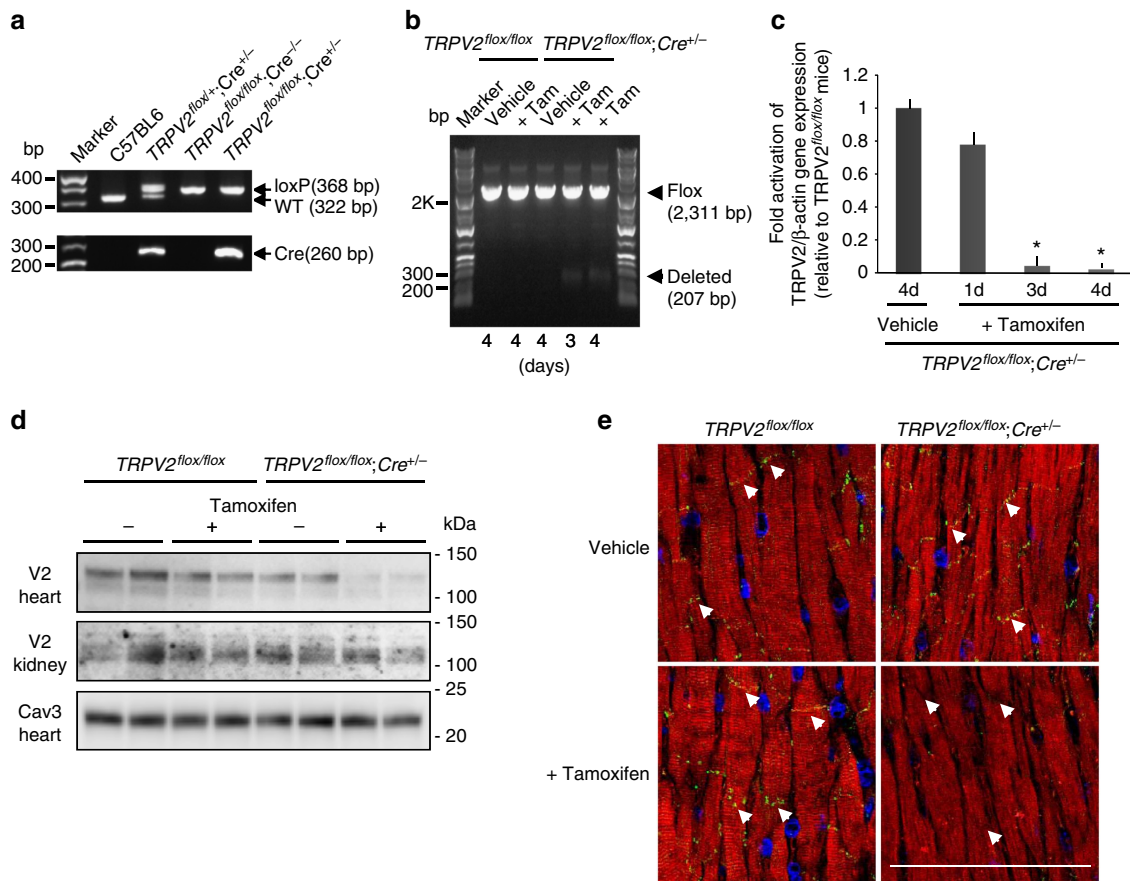
Figure 1 | Generation of temporally controlled cardiac-specific TRPV2-deficient mice. (a) Genotyping of TRPV2^{flox/flox}; MerCreMer^{+/-} mice using tail genomic DNA. (b) Confirmation of Cre recombination by PCR of cardiac genomic DNA. (c) TRPV2 messenger RNA expression confirmed by RT-PCR, using \beta -actin as an internal control gene ( n = 3 mice per group). Data are mean \pm s.e.m. *P < 0.05 versus non-treated age-matched TRPV2^{flox/flox}; MerCreMer^{-/-} ( TRPV2^{flox/flox} ) mice. (d) Expression of TRPV2 protein in heart and kidney from tamoxifen-treated and -untreated TRPV2^{flox/flox} or TRPV2^{flox/flox}; MerCreMer^{+/-} ( TRPV2^{flox/flox}; Cre^{+/-} ) mice, using caveolin 3 as an internal control for hearts. Membrane extracts (10 \mu g per lane) were subjected to immunoblotting. (See full blots with marker position in Supplementary Fig. 6). (e) Triple staining of left ventricle sections with anti-TRPV2 antibody (green), phalloidin (red) and DAPI (blue). Scale bar, 100 \mu m. Arrows, intercalated discs.
