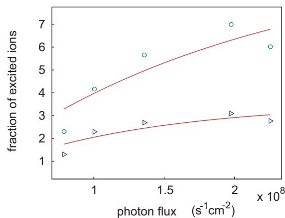
Figure 4.14: Minimum and maximum ratio of the tail to the peak area (blue triangles and green circles) fitted with the solution of the rate equation for the population of the excited state (red lines). The excitation cross section is a free fit parameter. The cross sections which are commensurate with the data are determined by the best fit.
