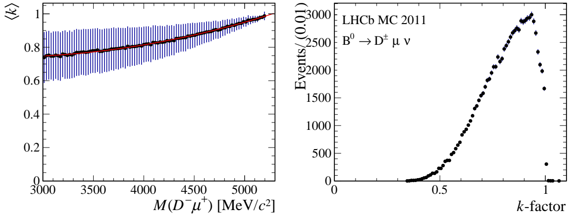
Figure 7.5: Left \langle k \rangle as function of the reconstructed B mass ( m(D^- \mu^+) ). Right k -factor distribution of all the B^0 \rightarrow D^- \mu^+ \nu_\mu X simulated events with 2011 conditions.
