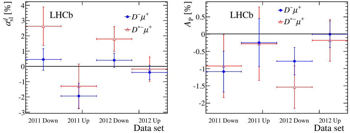
Figure 9.7: Left a_{sl}^d , Right A_P . Results on samples divided by year of acquisition and magnetic field polarity are compared. In blue the B^0 \rightarrow D^- \mu^+ \nu_\mu X results, in red the B^0 \rightarrow D^{*-} \mu^+ \nu_\mu X results. The statistical uncertainty on the single fit is added in quadrature to the uncertainty due to the statistical component of the uncertainty on the detection asymmetry measurements.
