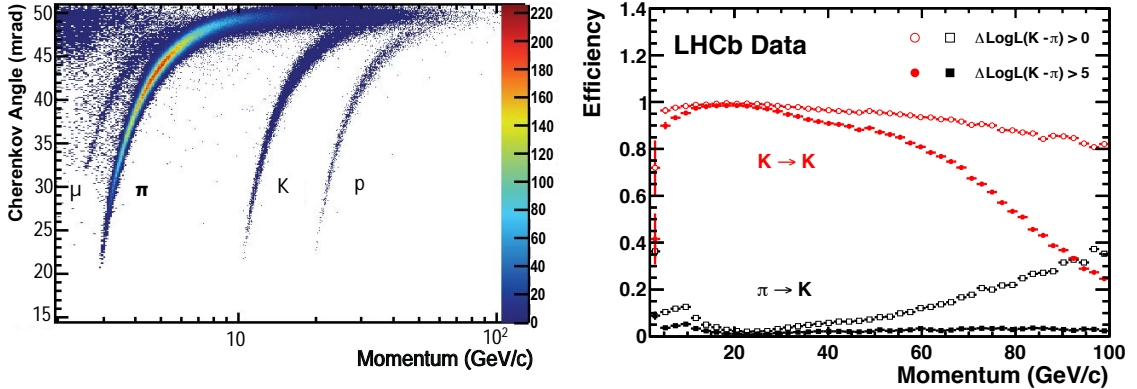
Figure 3.13: (left) Reconstructed Cherenkov angle \theta_{Ch} in function of momentum of the tracks transversing C_4F_{10} radiator. The Cherenkov bands for the different particles are visible. (right) Kaon identification efficiency and pion misidentification rate as function of the particle momentum, measured on data. The different marker indicate the different \Delta \log \mathcal{L}(K - \pi) used. More details about this quantities can be found in the reconstruction Sec. 3.3.2. Figs taken from reference [80], [59].
