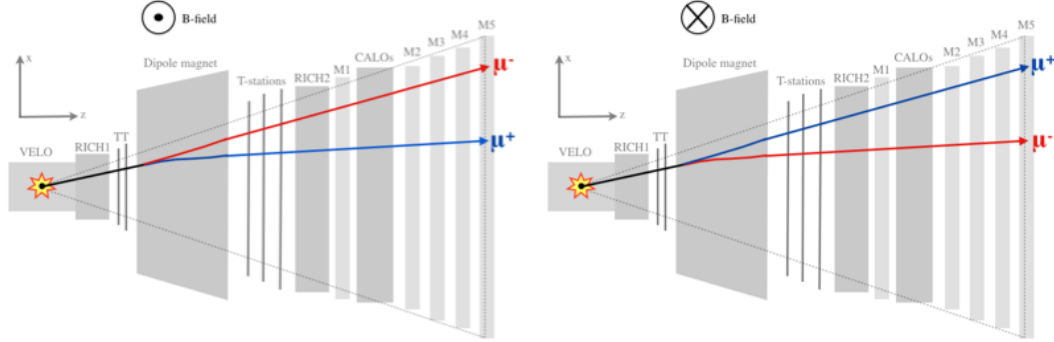
Figure 3.7: Illustrative example of trajectories of two muons with the same initial kinematics but opposite charges. The left and right figure correspond to the polarities up and down respectively of the LHCb dipole magnet. Figure taken from [73].
