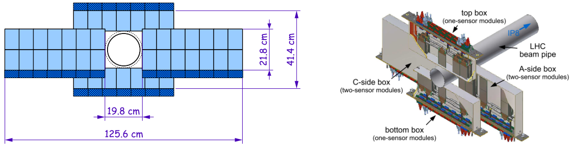
Figure 3.10: Layout of the IT. (Left) The silicon sensors are highlighted with light blue color, while the readout electronics is identified with dark blue color. (Right) The four IT boxes and the layers structure are shown. Figures taken from [75], [71]
