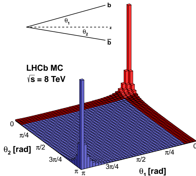
Figure 3.4: Polar angle distribution of b and \bar{b} collisions at \sqrt{s} = 8 \text{ TeV} . The beam line lies on the z -axis and the red region corresponds to the LHCb acceptance. The figure is taken from [66]
