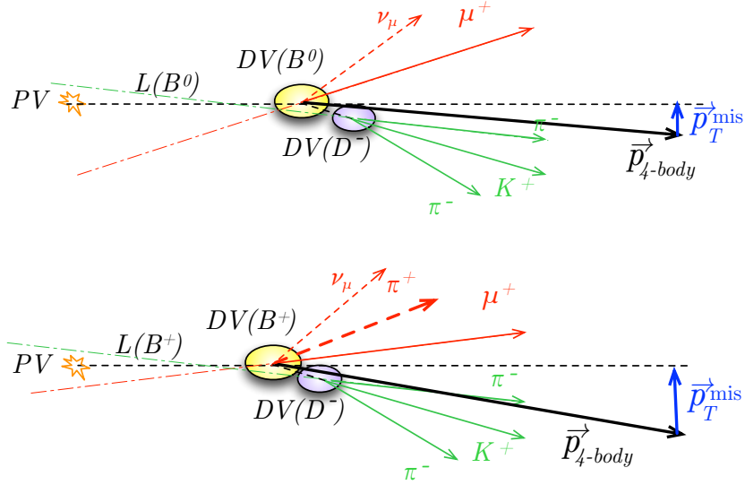
Figure 5.5: Sketch of signal and B^+ background decays reconstructed in D^- \mu^+ X sample. Solid lines are track reconstructed, dashed lines are not (except for the B flight direction indicated with the dashed black line). The definition of p_T^{\text{mis}} is highlighted. More tracks are missed in the reconstruction of a decay, larger |p_T^{\text{mis}}| values are expected and lower values are expected for the corrected mass (see Eq. 5.12). For these two examples the corrected mass distributions can be visualized from simulated events in Fig. 5.7.
