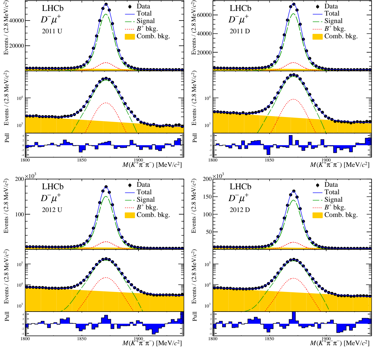
Figure B.1: Invariant mass distributions of the K^\mp \pi^\pm \pi^\pm combinations. The fit results are overlaid to the distribution of the dataset of each year and magnet polarity. The data distributions shown are obtained after applying the kinematical weights (see Sec. 6.5.1). For each subsample, the first two top rows show the invariant mass distributions using a linear and a logarithmic y-axis, respectively. The last row shows the so-called Pull values, i.e. the difference between the number of events observed in data for each bin of the histogram and the number of events predicted by the model in the same bin, divided by the uncertainty on the number of events.
