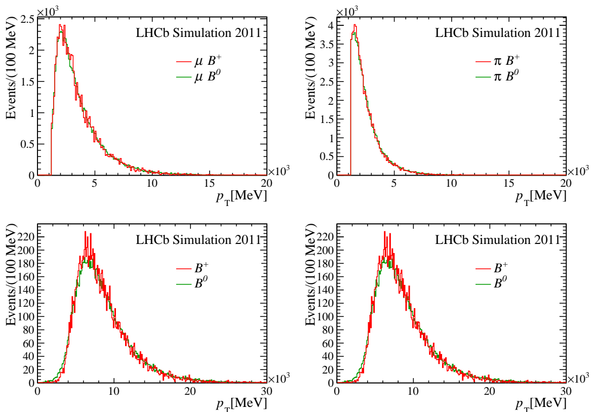
Figure 8.2: Muon and highest p_T pion transverse momenta spectra, reconstructed B meson momentum and p_T for B^0 \rightarrow D^- \mu^+ \nu_\mu X and B^+ \rightarrow D^+ \mu^- X^+ simulated events with 2011 conditions. The \mu\pi kinematical weights discussed in Sec 6.5.1 are not applied for these plots.
