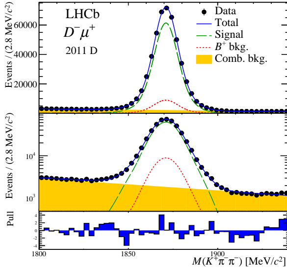
Figure 8.6: The invariant K^\mp \pi^\pm \pi^\pm mass distributions of the B^0 \rightarrow D^- \mu^+ \nu_\mu X magnet-down 2011 data sample, with fit models overlaid. The first two top rows show the invariant mass distributions using a linear and a logarithmic y-axis, respectively. The last row shows the so-called Pull values, i.e. the difference between the number of events observed in data for each bin of the histogram and the number of events predicted by the model in the same bin, divided by the uncertainty on the number of events of the bin.
