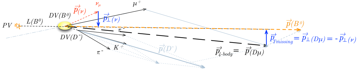
Figure 7.1: Sketch of signal semileptonic B^0 \rightarrow D^- \mu^+ \nu_\mu decay. The momenta of the reconstructed particles are indicated with solid black line, while the not reconstructed momentum is indicated with red dashed line. The black dashed three-momentum labeled as “ \vec{p}(D^- \mu^+) ” is the sum of the momenta of the reconstructed particles, also indicated as “reconstructed” B momentum. The orange dashed three-momentum corresponds to the “true” momentum of the B meson.
