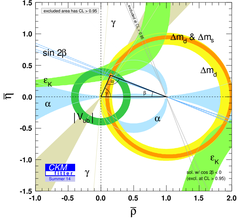
Figure 2.1: Unitarity Triangle: Constraints in the (\bar{\rho}, \bar{\eta}) plane [22].
