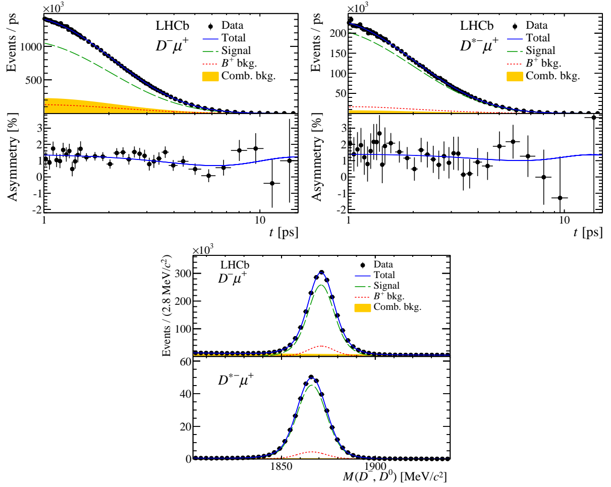
Figure 10.2: Top: B decay time distribution and charge asymmetry for D^- \mu^+ (left) and D^{*-} \mu^+ (right) samples. The datasets of each year and magnet polarity are combined and the fit results are overlaid. The number of bins for the charge asymmetry is reduced for illustration purposes. The non-zero charge asymmetry is due to the detection asymmetries (offset of the oscillating behavior) and B^0 production asymmetry (amplitude of the oscillating behavior). Bottom: Mass distributions of D^- candidates in the D^- \mu^+ sample and \overline{D}^0 candidates in the D^{*-} \mu^+ sample. The datasets of each year and magnet polarity are combined and the fit results are overlaid. All the data distributions shown are obtained after applying the kinematical weights (see Sec. 6.5.1).
