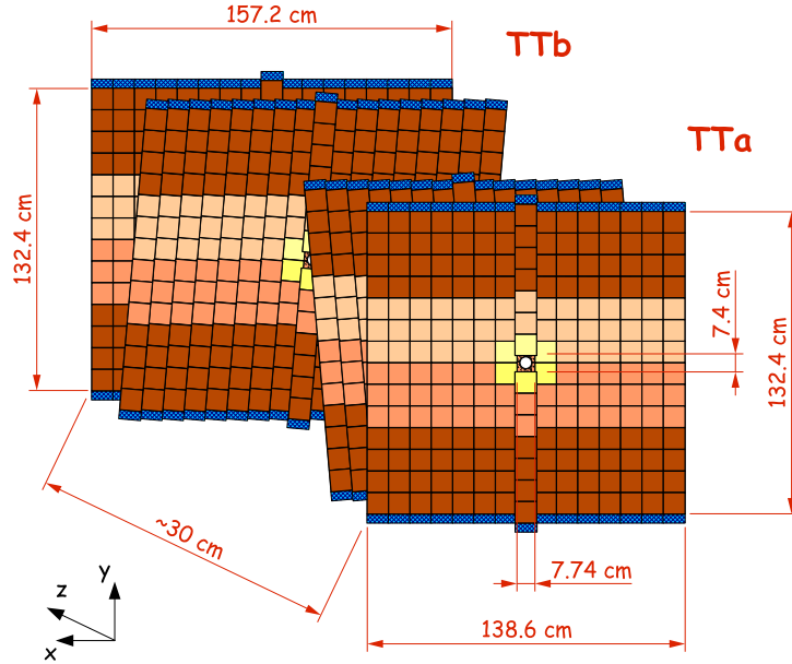
Figure 3.9: Layout of the four TT layers. Second and Third layers are tilted by \mp 5^{\text{deg}} . Different colors correspond to different readout sectors, the blue rim indicates the position of the readout electronics. Figure taken from [75].
