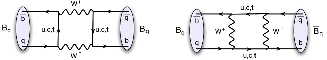
Figure 2.2: Dominant Feynman diagrams responsible for neutral B meson mixing in the SM.
