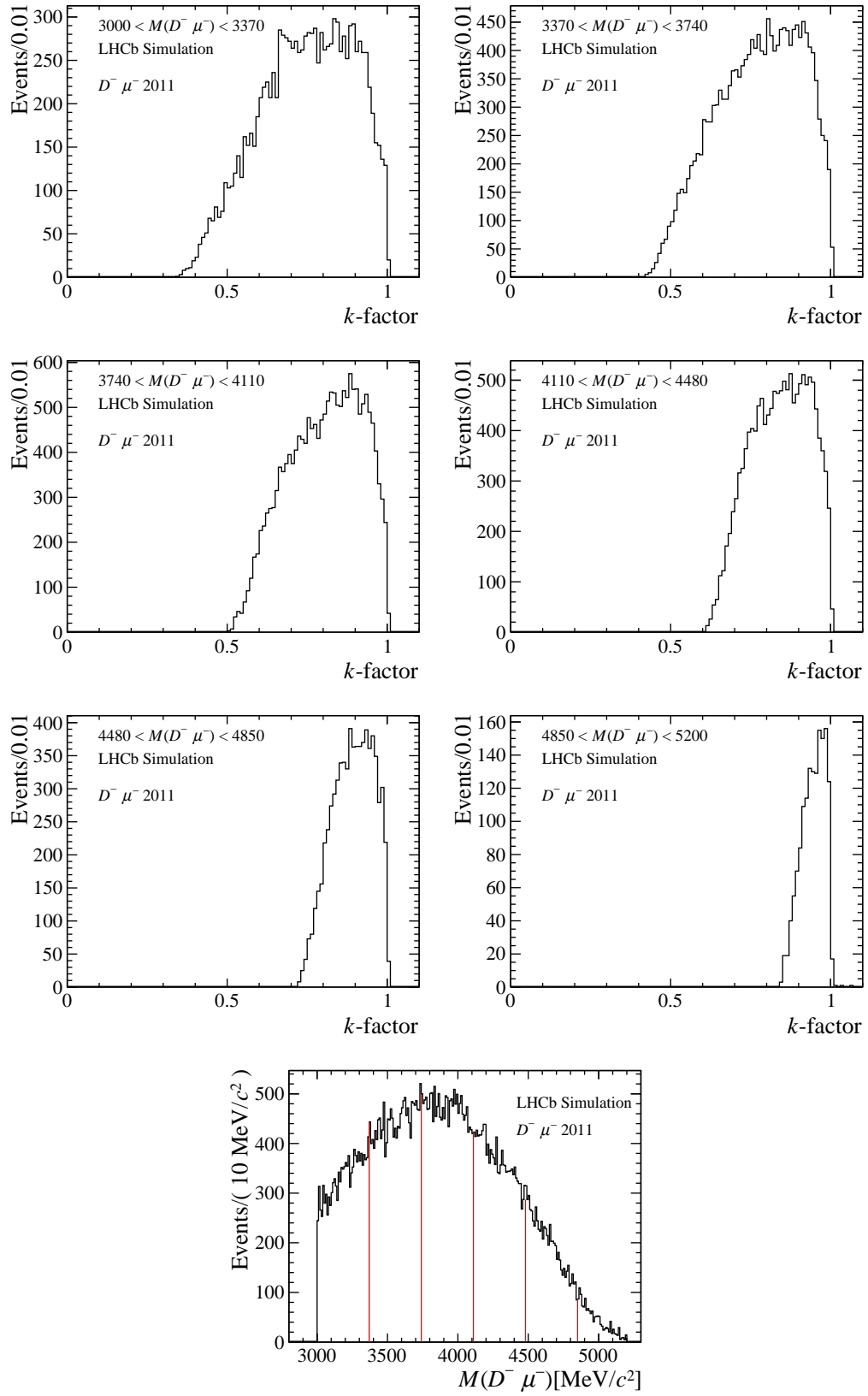
Figure 7.4: k -factor distribution in different mass ranges, correspondently indicated on the reconstructed B^0 mass distribution.
