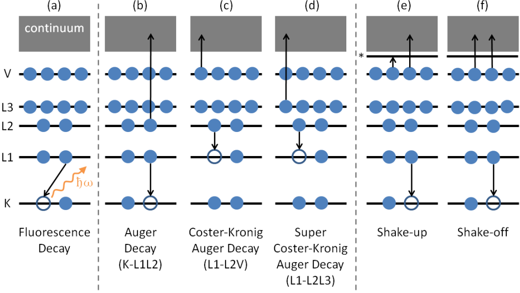
Figure 2.2: Overview of the main de-excitation processes possible after creation of an inner-shell vacancy, namely fluorescence and Auger decay. Also higher-order ionization processes, i.e. shake-up and shake-off, are sketched.
