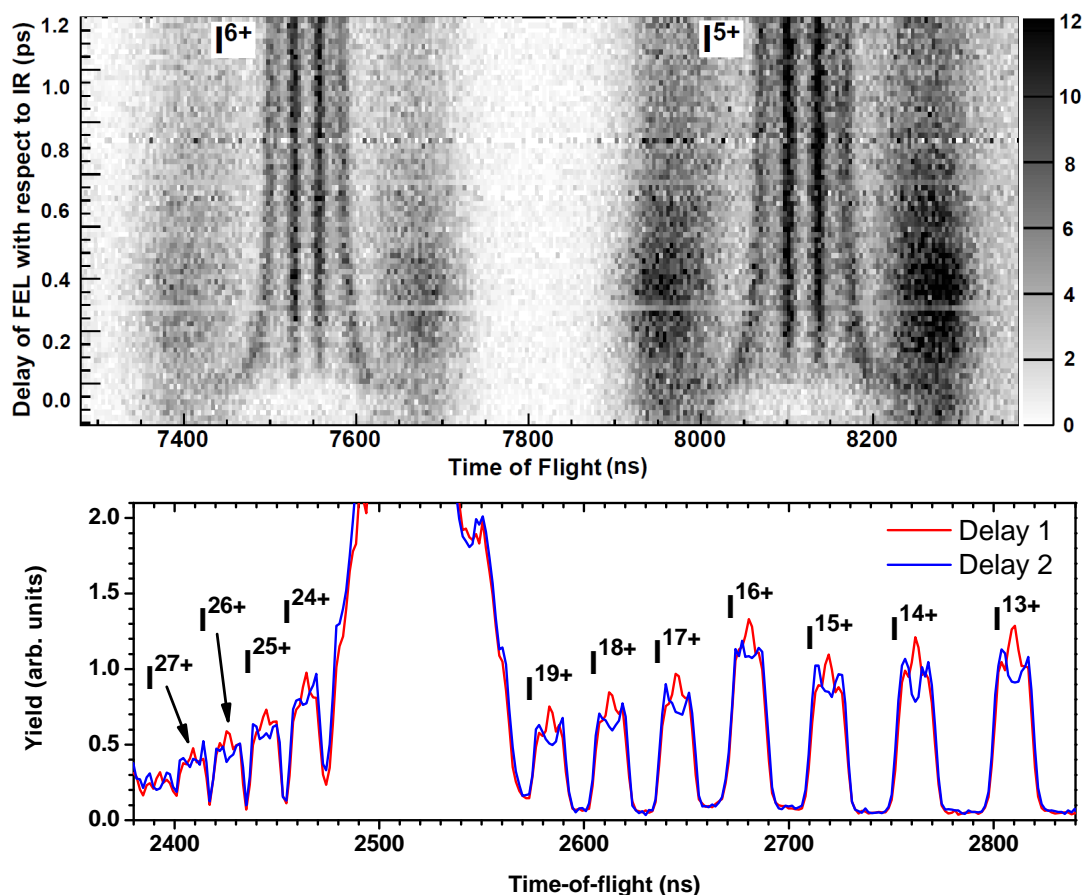
Figure 5.1: (a) Time-of-flight spectrum of I^{5+} and I^{6+} ions resulting from the LCLS-induced fragmentation of CH_3I molecules dissociated by an 800 nm IR laser pulse, shown as a function of IR/ X-ray pump-probe delay. (b) Time-of-flight spectrum for two respective delays between the IR pump pulse and the 1500 eV X-ray probe pulse. The red curve shows the spectrum where the IR pulse arrives 1 ps before the FEL pulse; the blue curve shows the spectrum where the IR pulse arrives 0.1 ps before the FEL pulse. The change of the shape of the TOF peaks reflects large internuclear distance and, thus, decreased Coulomb explosion energy at large IR/X-ray delays.
