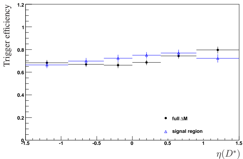
Figure 9.1: Trigger efficiency for data for the whole \Delta M region (full circles) and only the signal region (open triangles).
