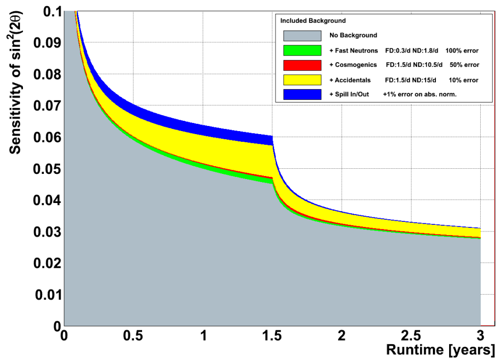
Figure 5.10: Expected sensitivity of Double Chooz for realistic systematic uncertainties and the different background contributions. The Spill In current can be a 0.5-1.4% effect on the absolute normalization, depending on applied cuts. For simplicity 1% is shown.
