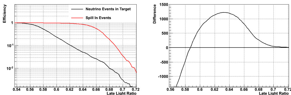
Figure 4.32: Left: Efficiency to accept a neutrino event in the target and a Spill In event for different LLR.
