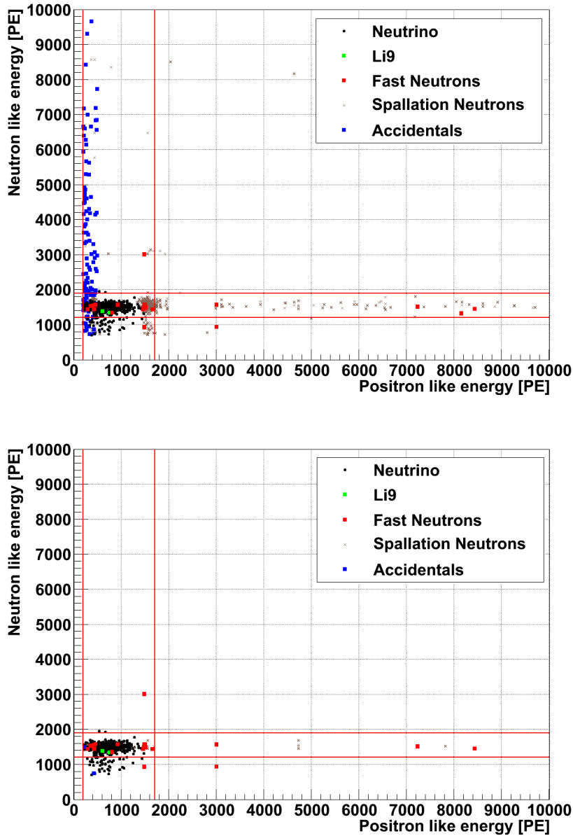
Figure 4.1: Correlation of positron- and neutron-like events produced by simulation for 10 days data taking equivalent.
