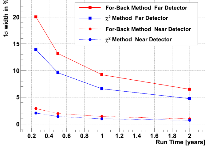
Figure 3.8: 1\sigma width of the relative residual for the reconstructed number of neutrino events for the two different methods described in the text over the runtime.
