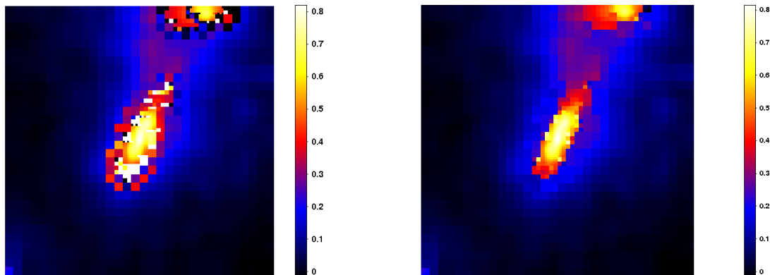
Figure 5.9: The recovery of the convergence from the lensing potential on an AMR grid . Left Panel: The result without our rejection technique, which delivers a quite noisy result. Right Panel: The result with the rejection technique described in the text. The noise has almost disappeared completely.
