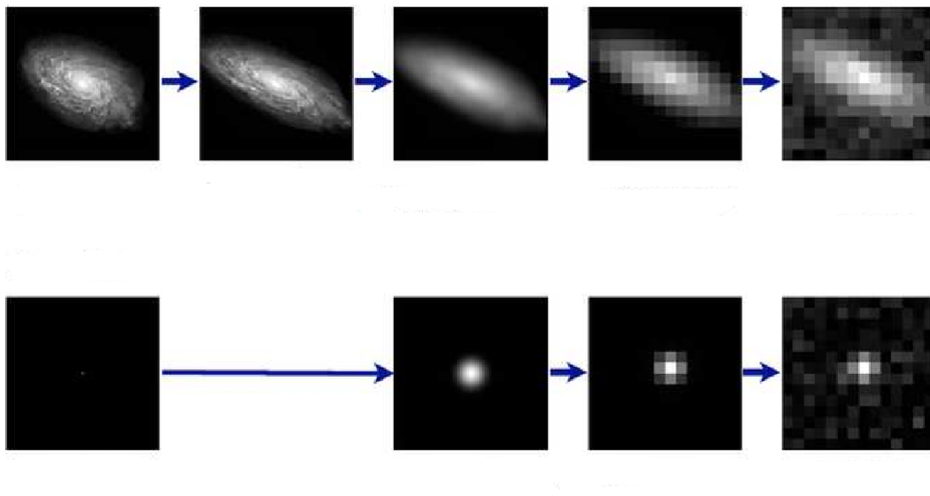
Figure 2.3: From Bridle et al. (2008) . The upper panel shows the ‘forward’ process of gravitational lensing. A galaxy is sheared by the gravitational tidal and its image is convolved afterwards with the PSF. The pixelised detector output contains additionally a significant amount of noise. The lower panel shows the same effects on the image of a star, with the difference that it is not lensed.
