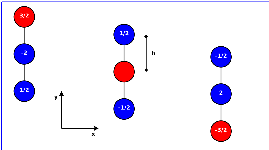
Figure 4.3: The finite-differences scheme for the first component of the deflection angle (Eq. 4.12) is shown in the top panel . The bottom panel shows the scheme for the second component (Eq. 4.13). Marked in red is the grid cell, for which the deflection angle is calculated. The coefficients are given in units of h . Please note, that a higher-order Taylor expansion has been used, which is why the schemes in the figure do not match exactly with Eqs. 4.3, 4.4.
