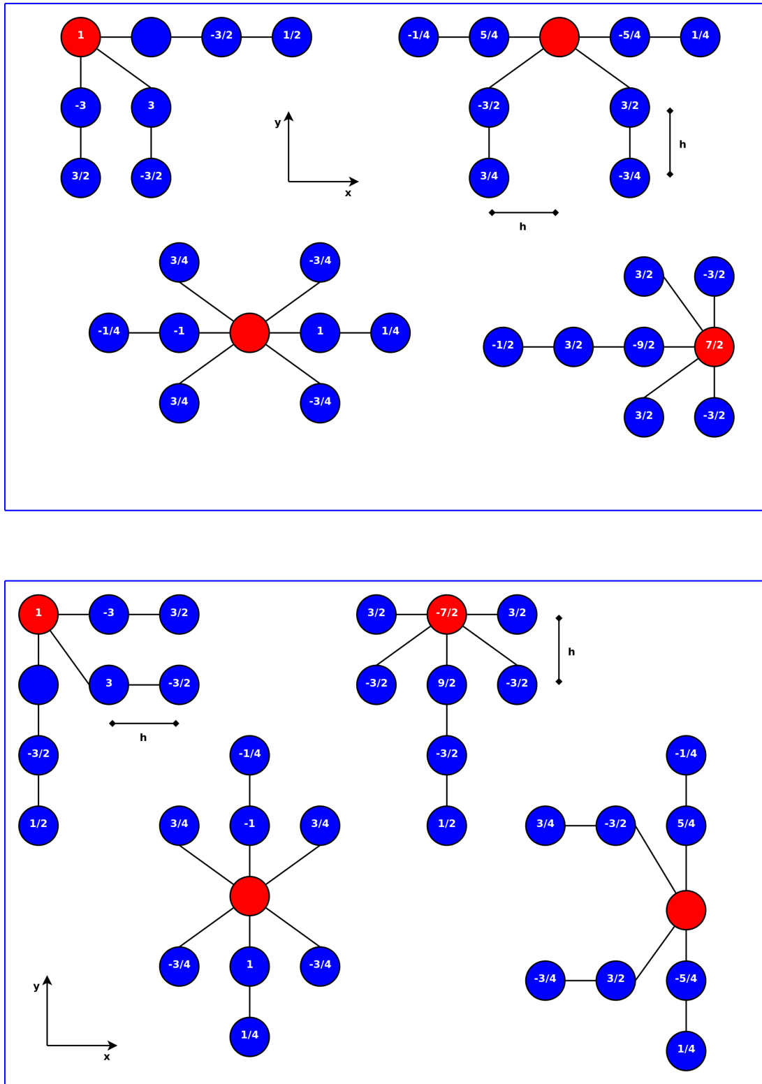
Figure 4.6: The finite-differences scheme for the first component of the G -flexion (Eq. 4.19) is shown in the top panel . The bottom panel shows the scheme for the second component (Eq. 4.20). Marked in red is the grid cell, for which the G -flexion is calculated. The coefficients are given in units of h^{-3} .
