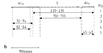
Figure 4. Alignment of the sequenced RNA fragments with the human 7SL RNA sequence. a: Y = pyrimidines. N = unidentified nucleotide. Where indicated, the sequence for all four bases was determined. The arrows indicate the 3' end of each fragment. The dotted line spans the region of cleavage of micrococcal nuclease. b: schematic representation of the dog RNA fragments, numbered from 1 to 5 according to size as in figure 3. The number of nucleotides for each fragment are given. The position of Alu and S sequences within the 7SL RNA are indicated above.
