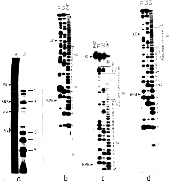
Figure 3. RNA sequence analysis of the 3' terminal portion of fragments 3 and 4. The labelled RNA was obtained from SRP (1 A280 unit/ml) digested 30 min. at 37°C with 10,000 units/ml micrococcal nuclease in 0.4 M KAc and electrophoresed in a 6% polyacrylamide-urea gel. a: ethidium bromide staining (A) and autoradiography (B) of the gel from which the RNA was eluted. b, c and d: sequencing gels of fragments: 3 (20% gel), 4 (10% gel) and 4 (20% gel). The corresponding nucleotides are shown on the side of the sequencing ladder and numbered according to the sequence of Ullu et al. (1). XC = xylene cyanole, BPB = bromophenol blue. T1 and U2 indicate the respective ribonucleases. OH: partial alkaline hydrolysis. -ENZ = untreated RNA. * identical to the rat in this position (4), but T-A transversion as compared with human 7SL RNA sequence.
