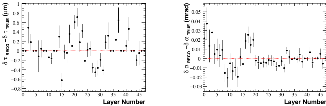
Figure 5.28: Alignment results after 21 iterations, shifts along measurement direction \delta\tau and rotation around beam axis \delta\alpha , error bars given by the alignment method. 450 GeV+ 450GeV, Open-VELO.
