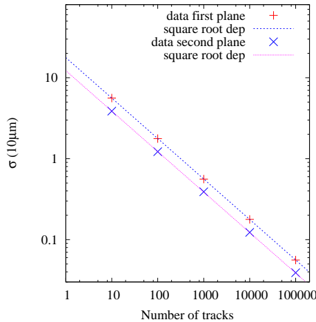
Figure 4.1: Alignment precision dependence on the number of tracks in the alignment sample
