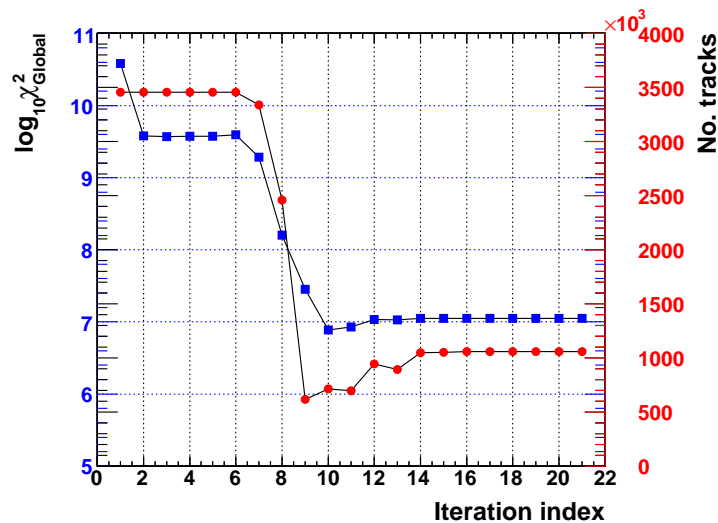
Figure 5.20: Evolution plot of the global \chi^2 and Number of tracks with iteration Number
