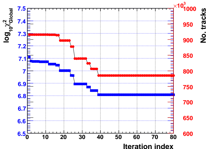
Figure 5.34: \chi^2 and track number versus iteration index for Particle Gun data, ladder alignment
