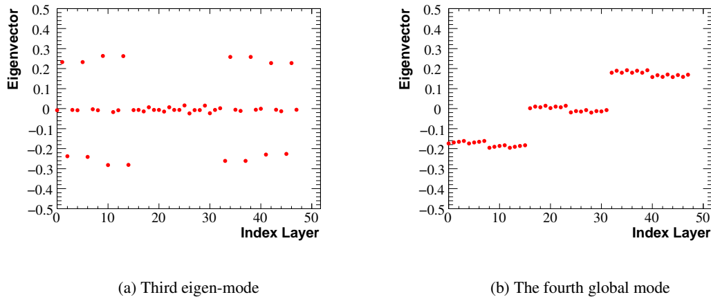
Figure 5.41: Global shearings as eigen modes of the alignment matrix
