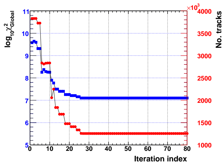
Figure 5.38: \chi^2 and track number versus iteration index for 10 TeV data sample, ladder alignment
