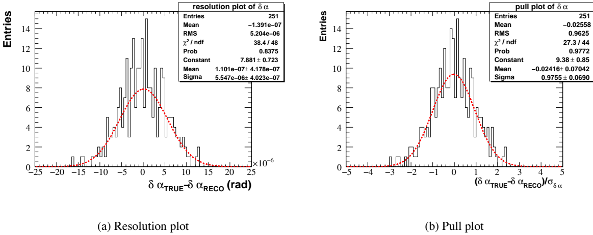
Figure 4.2: Resolution and pull plots for \delta\alpha in a Toy Monte Carlo
