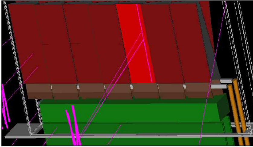
Figure 4.6: One box of IT with 4 sensors triggered by a particle with long tracks, Importance of hierarchy is outlined. Triggered strips in Magenta with the same color for tracks. The first 7 sensors of the Box are shown together with the partially visible gray and red ladders of the layers behind the first layer of sensors. The first sensor with a triggered strip is highlighted with lighter red.
