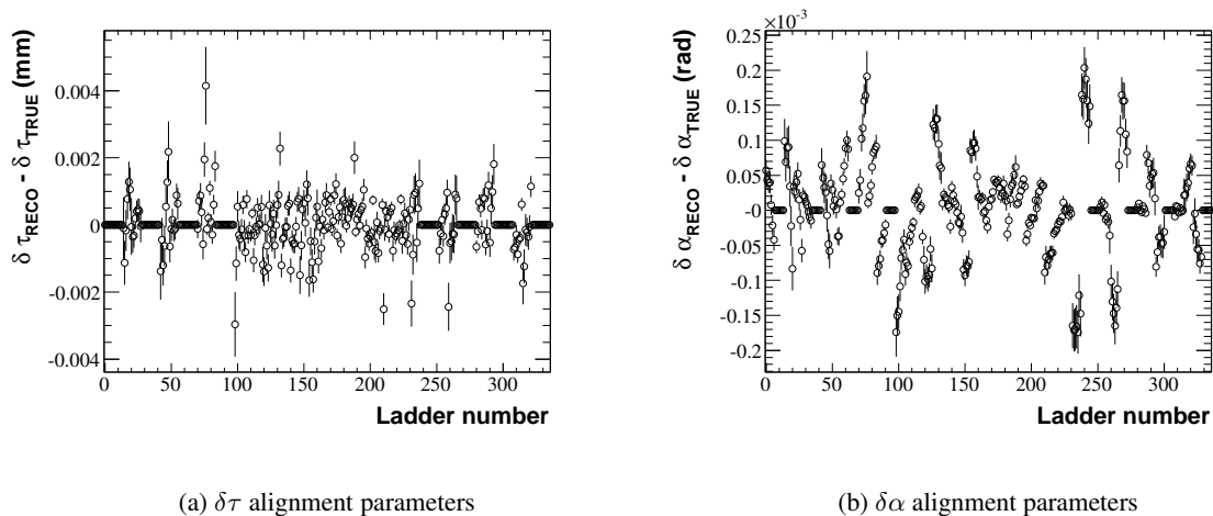
Figure 5.33: Resolution plots, ladder alignment results in \alpha and \tau , for a minimally constrained setting
