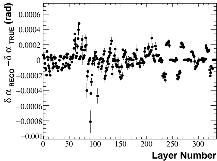
Figure 6.8: \delta\alpha alignment resolutions with Millepede errors estimates, alignment performed for 2 types of alignment parameters at ladder level.
