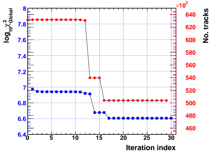
Figure 5.47: Alignment \chi^2 and track number as they evolve with each iteration
