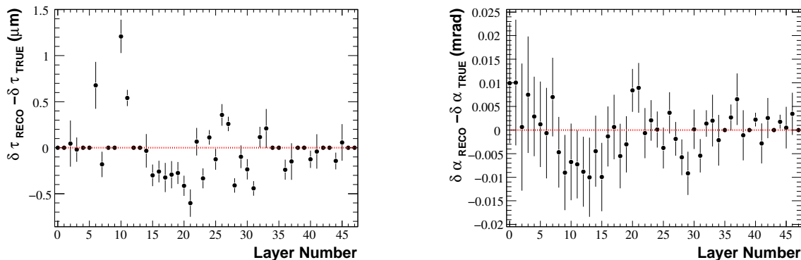
Figure 5.17: Alignment results after 21 iterations, shifts along measurement direction ( \delta\tau ) and rotation around beam axis \delta\alpha , error bars given by the alignment method. Alignment starts with a misaligned geometry.
