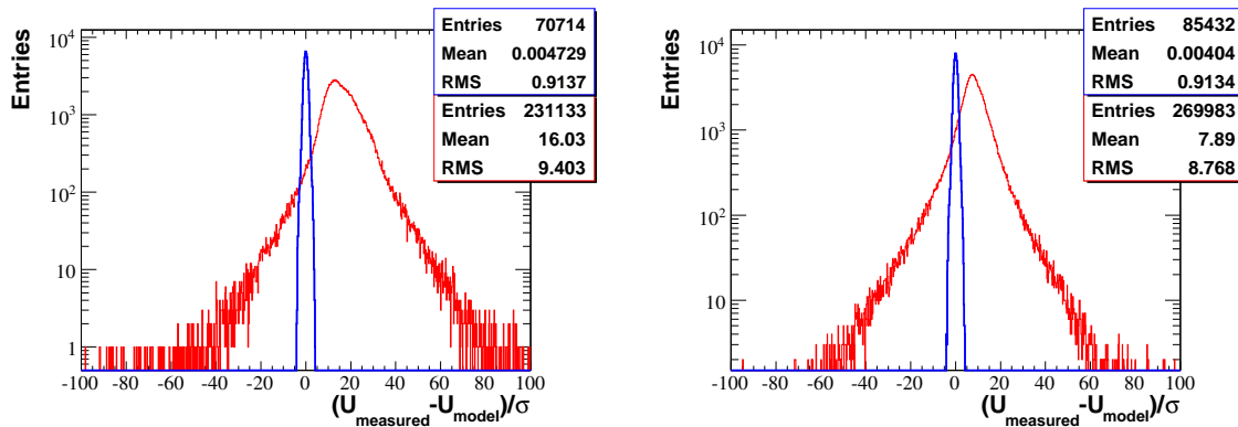
Figure 5.23: Plot of residuals for measurements in two sensors, left a sensor in 1st Station, right a sensor in 3rd Tracking Station. Red histograms are before alignment and blue after alignment. All Minimum Bias events were used in alignment. The blue plot includes only the tracks used in the last iteration step of alignment. Sensors as in 5.22
