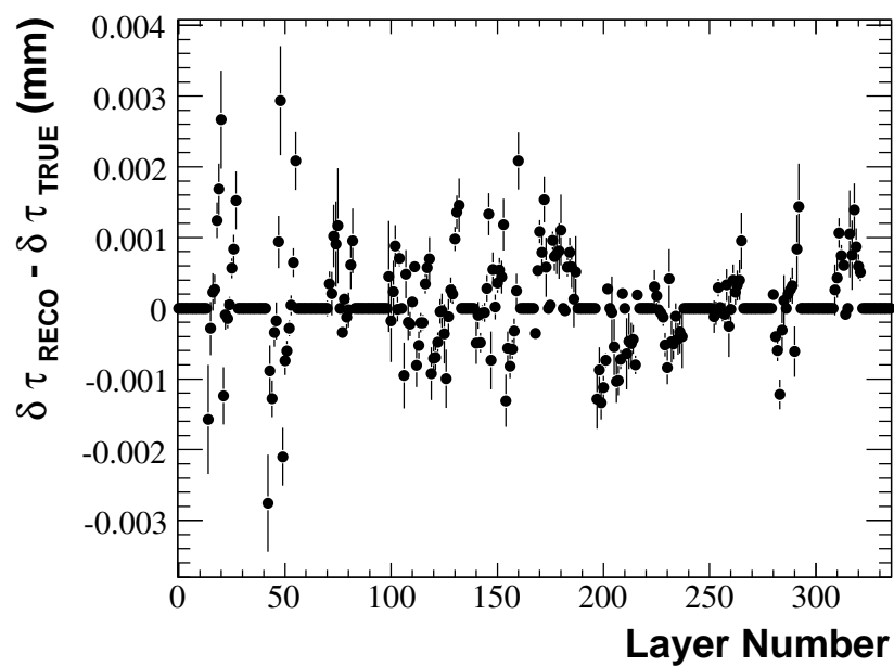
(a) \delta\tau resolution plot
