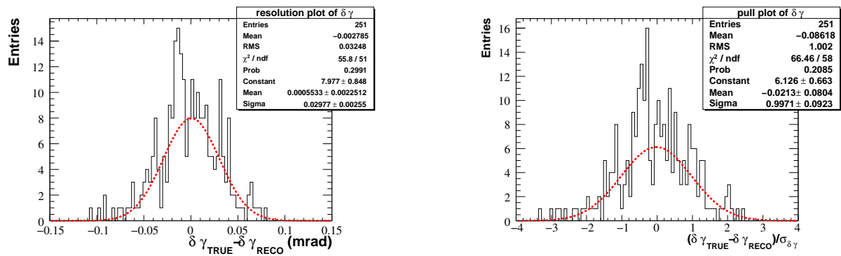
Figure 8.3: IT layers, Toy MC results, resolution and pull-plots of \delta\gamma DoF for 251 independent alignment runs with totally distinct track samples
