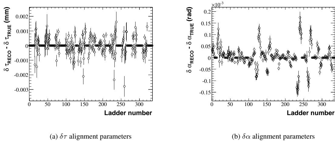
Figure 5.31: Resolution plots, ladder alignment results in \alpha and \tau for alignment with Particle Gun data, over-constrained system
