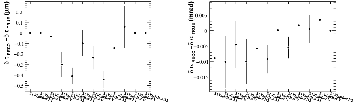
Figure 5.18: Alignment results after 21 iterations, with corresponding Station, Box, Layer index label
