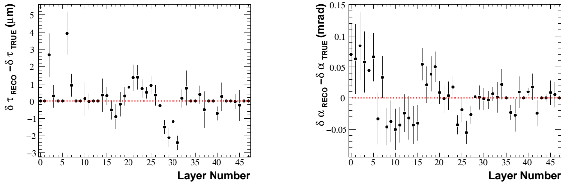
Figure 5.26: Alignment results after 27 iterations, shifts along measurement direction ( \delta\tau ) and rotation around beam axis \delta\alpha , error bars given by the alignment method. 7+7 TeV, Closed-VELO.
