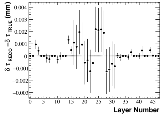
(b) \delta\tau degrees of freedom, reduced sample
