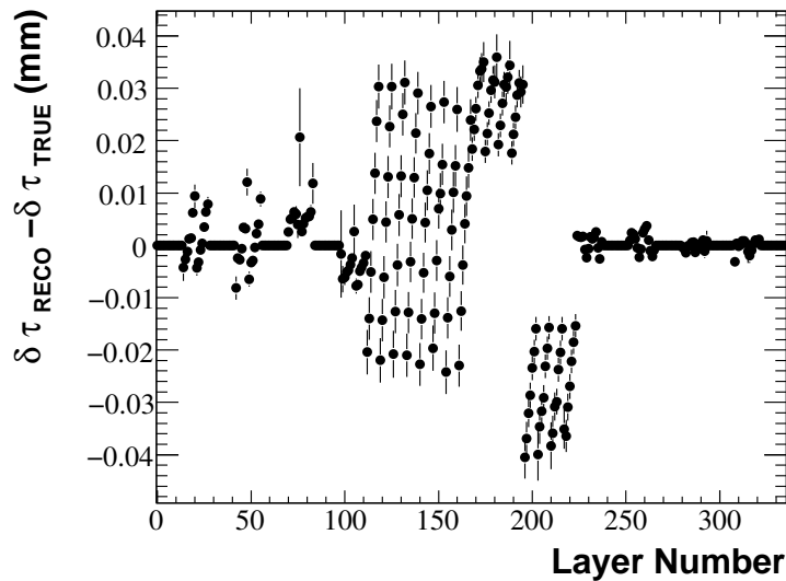
Figure 6.7: \delta\tau alignment resolutions with Millepede errors estimates, alignment performed for 2 types of alignment parameters at ladder level.
