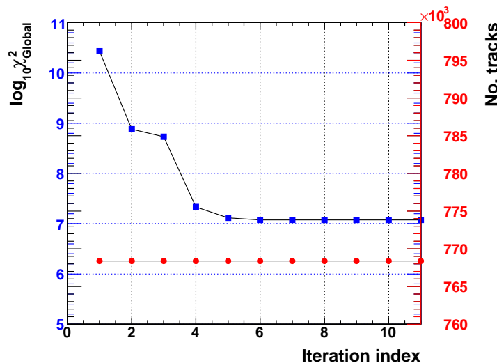
Figure 6.6: Alignment global- \chi^2 evolution and the constant track number in absence of track- \chi^2 quality cut.
