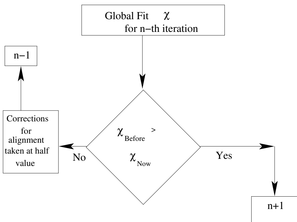
Figure 3.3: Extra quasi-Newton step for the a Newton-Raphson iteration
