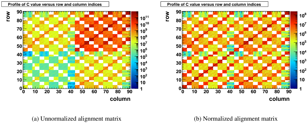
Figure 5.43: Normalized and unnormalized alignment matrix for 91 non-fixed alignment parameters, 47 \delta\alpha , and 44 \delta\tau , matrix axis y is reversed
