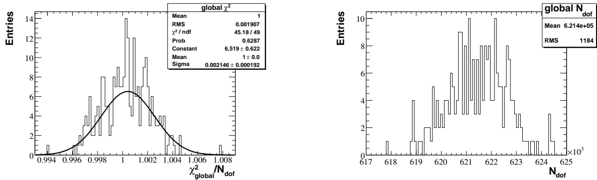
Figure 4.3: The reduced global \chi^2 and Number of degrees of freedom for 251 toy Monte Carlo independent runs, each of 10^5 tracks
