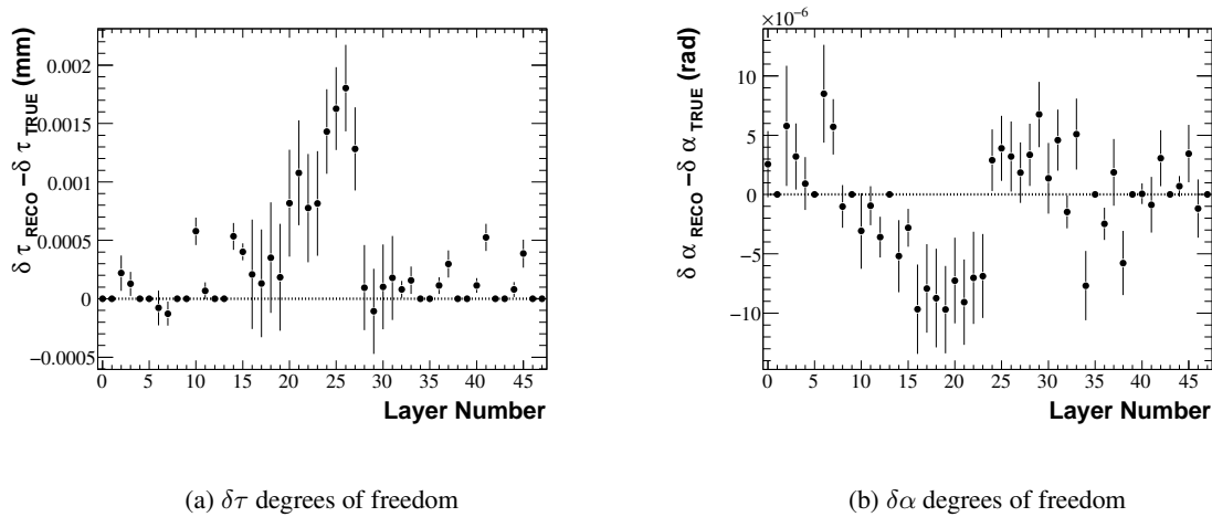
Figure 6.16: Alignment resolutions with Millepede errors estimates, alignment performed for 2 types of alignment parameters at layer level. Alignment used a charge symmetric distribution sample
