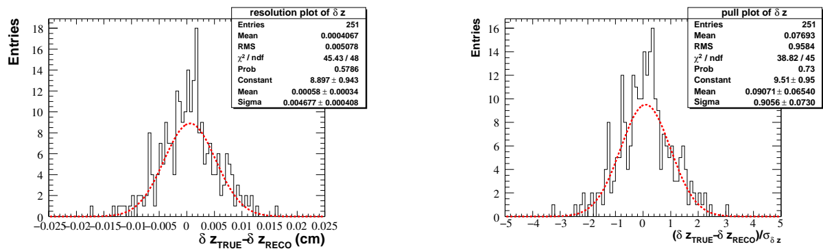
Figure 8.4: IT layers, Toy MC results, resolution and pull-plots of \delta z DoF for 251 independent alignment runs with totally distinct track samples
