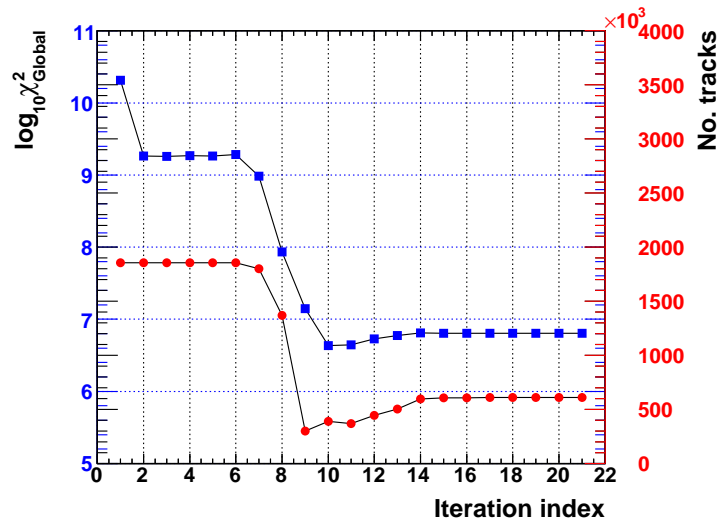
Figure 5.29: 21 iterations, alignment- \chi^2 dependence on iterations, number of useful tracks stability, 450GeV +450GeV, Open-VELO .
