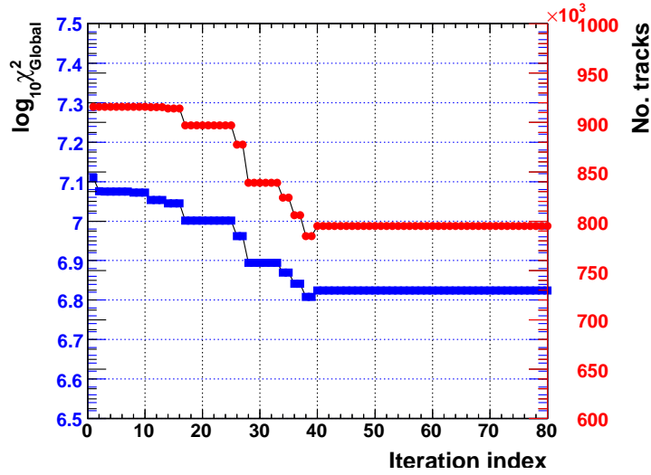
Figure 5.32: \chi^2 and track number versus iteration index for Particle Gun data, ladder alignment
