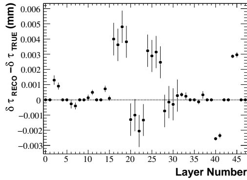
(a) \delta\tau degrees of freedom, full sample results
