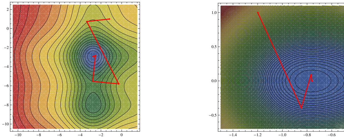
Figure 3.2: Plots of Newton-Raphson steps with the topological contours for the surface of the minimized function. Right Side of plot the function f(x, y) = 0.25x^2 + y^2/9 + 6 + x + y + \cos(x) + \sin(y + 1) and in the Left Side g(x, y) = x^2 + y^2/9 + 20 + 0.1x + y + \exp(\cos(x)) + \exp(-\sin(y)) .
