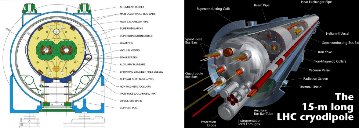
Figure 2.2: An 15-m long LHC dipole with cross-section and length views,
