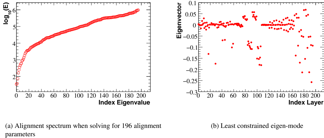
Figure 5.50: Spectrum and the least constrained eigen-mode of the normalized alignment matrix.
