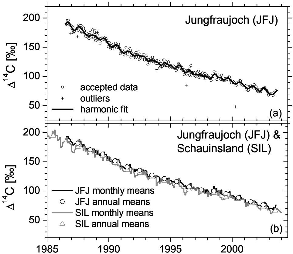
Figure 1 (a) Individual \Delta^{14}\text{C} measurements determined on bi-weekly integrated atmospheric \text{CO}_2 samples from Jungfrauoch. The solid line is a harmonic fit curve calculated through the data. (b) Monthly and annual mean \Delta^{14}\text{CO}_2 values from Jungfrauoch and Schauinsland stations.
