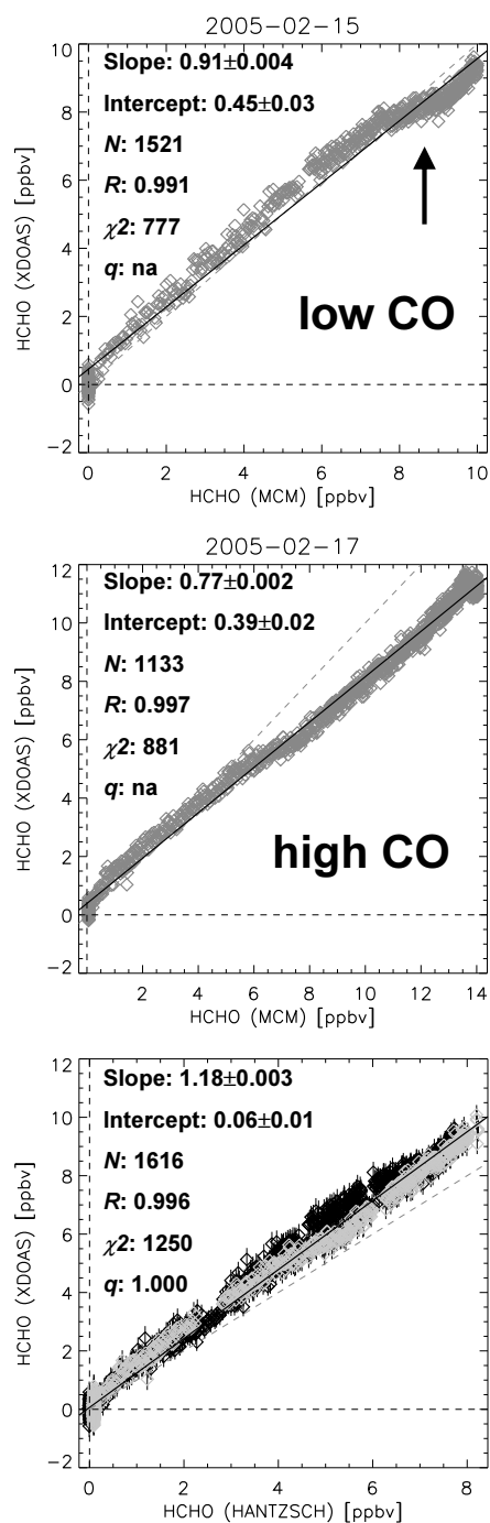
Figure 5.14: Correlation of XDOAS vs model calculation (MCMv3) for the ethene-ozone experiment without additional CO (upper panel) and at excess CO (centre panel). Arrow: occurrence of an unexpected mixing ratio dip. Lower panel: joint correlation of XDOAS vs Hantzsich for the two days, which are colour coded.
