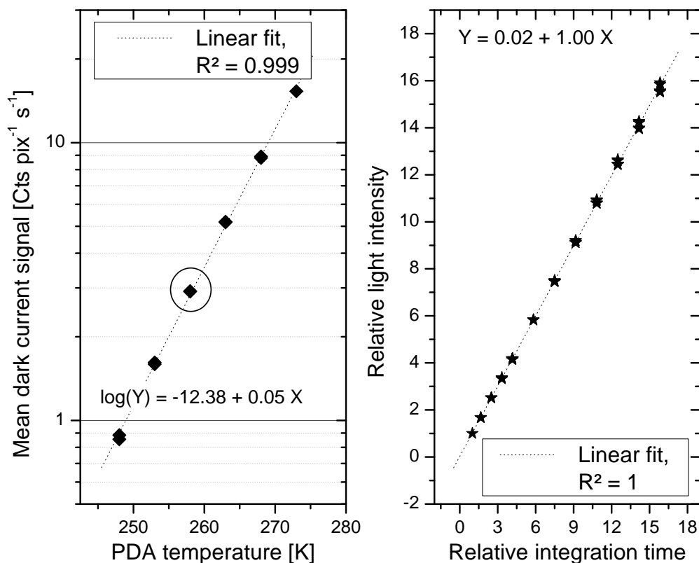
Figure 4.5: Left panel: temperature dependence of the average dark current signal of the Hamamatsu S3904. The circle denotes the standard measurement temperature (258 K = -15° C). Right panel: PDA response signal vs total integration time, both in relative units.
