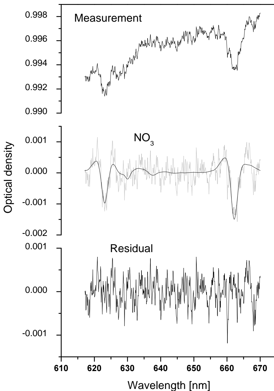
Figure 2.4: Sample fit of \text{NO}_3 . Spectrum recorded on 8 Sep 2005 at 13:57 UTC. RMS (residual) = 3 \times 10^{-4} . Absorption: 70 pptv ( \text{NO}_3 ). \text{NO}_2 , \text{H}_2\text{O} and Fraunhofer structures were not strong enough to be observed in that range.
