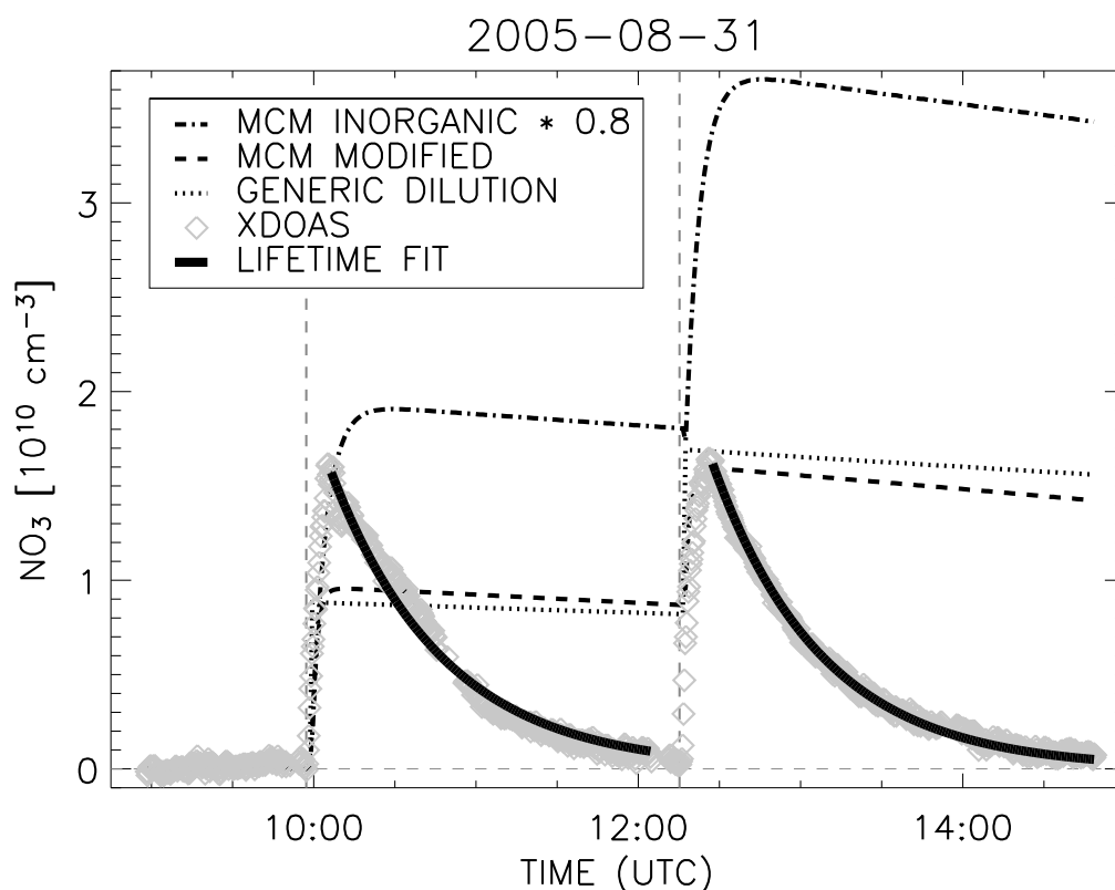
Figure 5.16: \text{NO}_3 time profiles calculated from the plain inorganic MCM mechanism (dashed-dotted line, scaled down by 20%), calculated from a modified MCM mechanism including reactions (viii) to (xi) from Table 5.3 (dashed line), and measured by the XDOAS (diamonds). Dotted line: effect of the dilution at generic concentrations. Solid line: exponential decay fit to the measured \text{NO}_3 data. Vertical lines: \text{NO}_2 injections.
