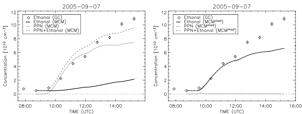
Figure 5.20: Left panel: time profiles of the product pairs ethanal / PPN in the \text{NO}_3 -propanal experiment as measured by the GC (diamonds) and as modelled using the MCMv3 (lines). Modelled and detected ethanal differ by a factor of 7. Right panel: results of a modified MCMv3 propanal module where PPN formation is suppressed.
