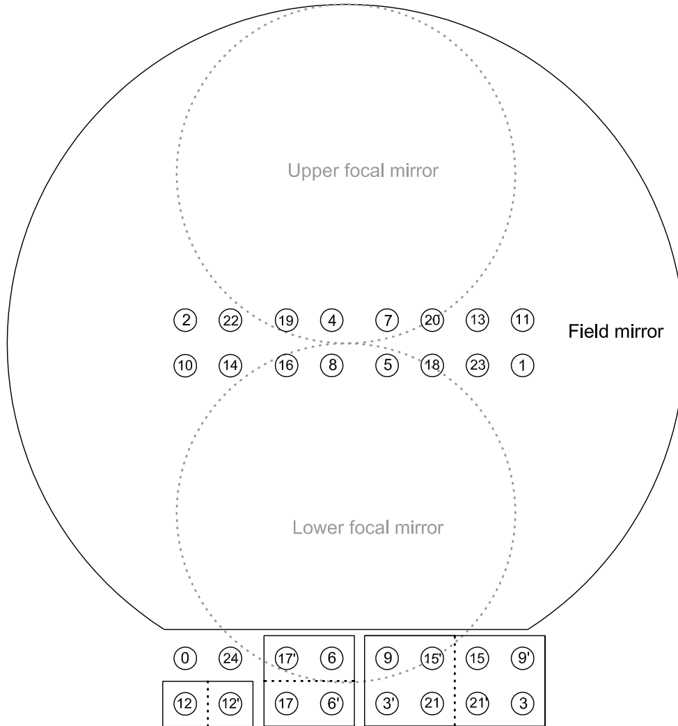
Figure 4.3: Light spot chart of the White cell with a front view of the field mirror (on top) and the three prisms (in line below). The set-up shown yields a total path length of 960 m being the longest path that can be realised providing reasonable light transmittance. Grey dotted lines mark the focal mirrors being situated at the other end of the chamber. Numbers denote the order of passing with 0 being the entrance and 24 being the exit spot.
