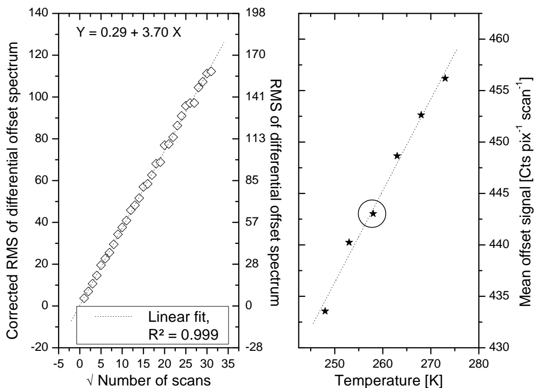
Figure 4.4: Left panel: dependence of the offset noise on the square-root of the number of scans at -15^\circ\text{C} . Right panel: temperature dependence of the electronic offset of the Hamamatsu S3904. The straight line is meant to guide the eye. The circle denotes the data point at the standard measurement temperature ( 258\text{ K} = -15^\circ\text{C} ).
