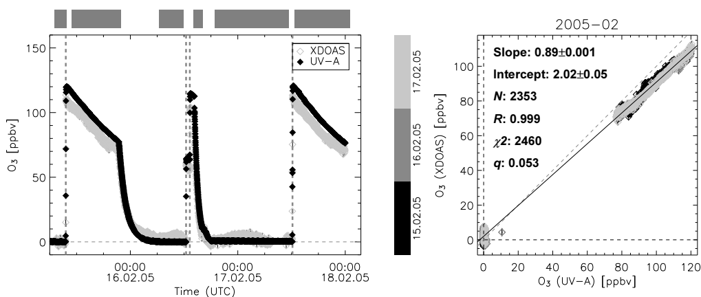
Figure 5.3: Left panel: O 3 profiles recorded by XDOAS and UV absorption in Feb 2005. Grey vertical lines: O 3 injections. Grey bars: data included in the correlation. Right panel: correlation plot. The days are colour coded.
