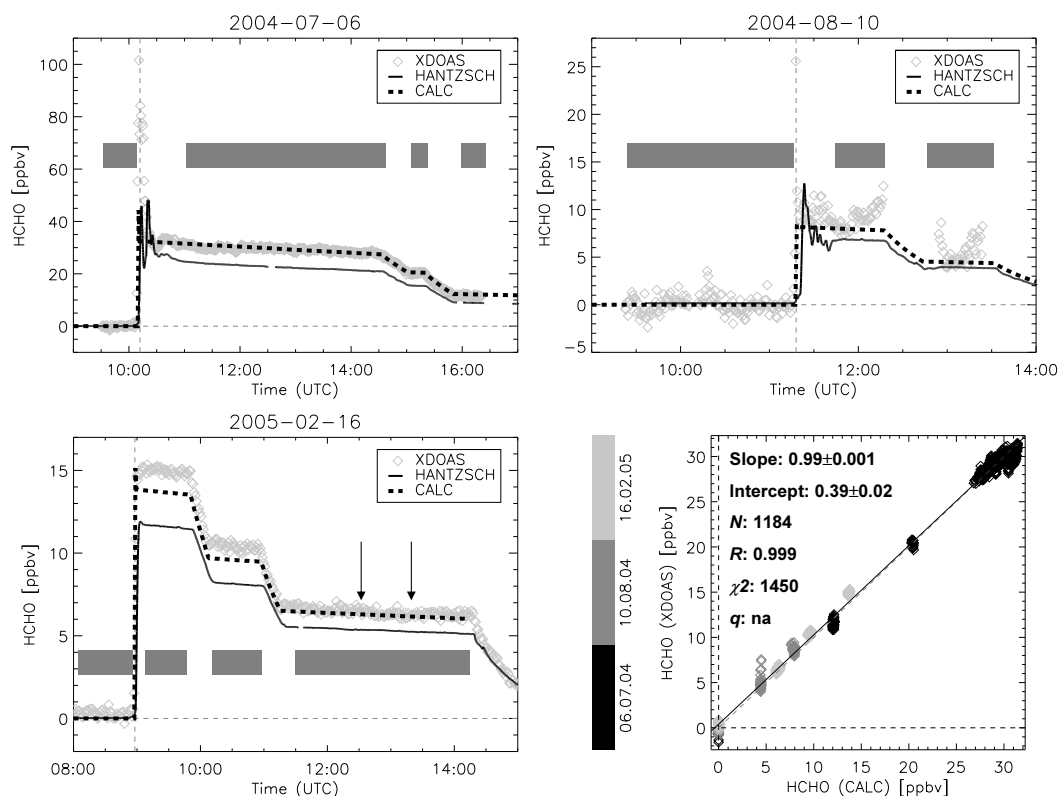
Figure 5.10: Upper left panel: HCHO profiles on 6 Jul 2004 as measured by XDOAS and Hantzsich, and as calculated. Grey vertical line: HCHO injection. Upper right panel: data from 10 Aug 2004. Lower left panel: data from 16 Feb 2005. Arrows: ozone additions. Grey bars: data included in the correlation. Lower right panel: correlation plot. The days are colour coded.
