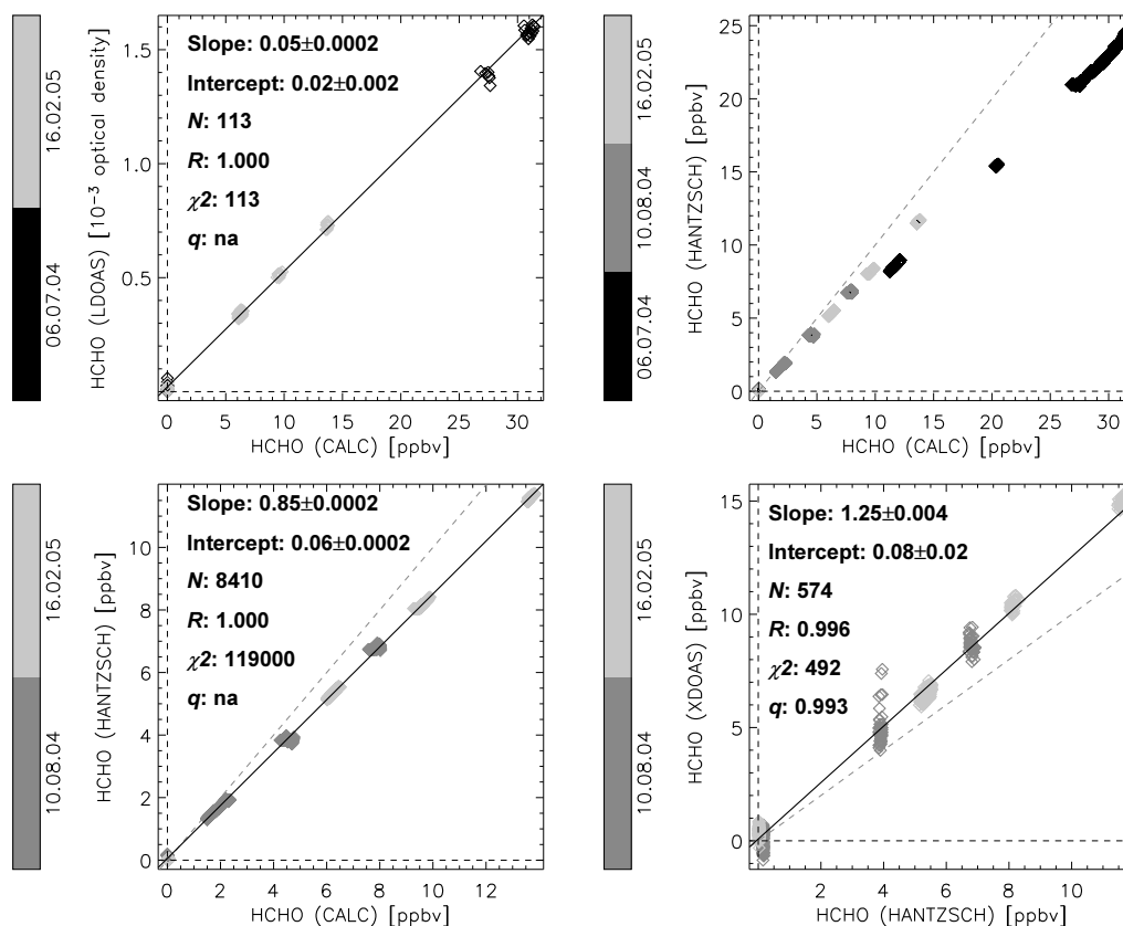
Figure 5.11: Upper left panel: correlation plot of LDOAS vs calculation. LDOAS data in optical densities. Upper right panel: Hantzscht vs calculation, all days. Lower left panel: Hantzscht vs calculation, two days only. Lower right panel: XDOAS vs Hantzscht for two days. The days are colour coded.
