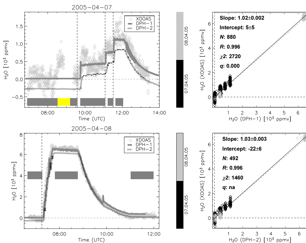
Figure 5.4: Left panels: profiles of H_2O recorded by XDOAS and two DPHs on 7 Apr (upper) and 8 Apr (lower) 2005. Grey vertical lines: water vapour injections. Yellow bar: period of daylight exposure. Grey bars: data included in the correlation. The data of DPH-2 were displaced by -300 ppmv for clarity. Right panels: correlation plot of XDOAS against DPH-1 (upper) and DPH-2 (lower). The days are colour coded.
