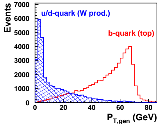
Figure 2.7: Generated transverse momentum distribution of the scattered u/d -quark in simulated W production events compared to the b -quark from simulated top decays.
