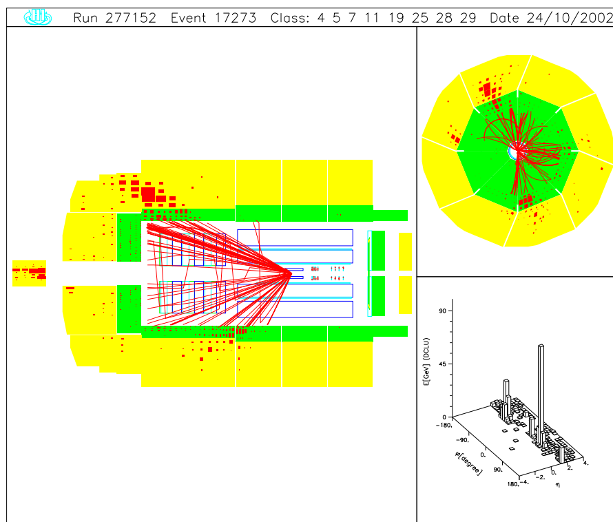
Figure E.1: t \rightarrow bW \rightarrow bq\bar{q}' candidate. P_T^{jet1,2,3} = 70, 69, 21 GeV , M_{jets} = 171 GeV , M_{2jet}^{Wcomb.} = 71 GeV.
