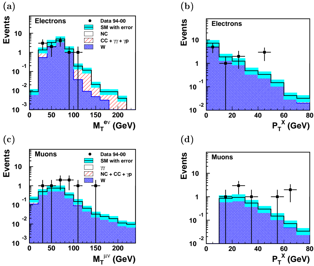
Figure 6.9: Final distributions of the transverse mass M_T^{l\nu} and the hadronic transverse momentum after the W selection.
