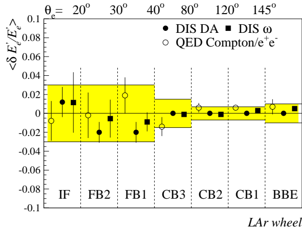
Figure 5.1: The mean fractional energy shift \delta E_e/E_e from the absolute energy scale obtained by two different reconstruction methods (DA-method, \omega -method). The error band shows the systematic uncertainty on the energy scale. Taken from [45].
