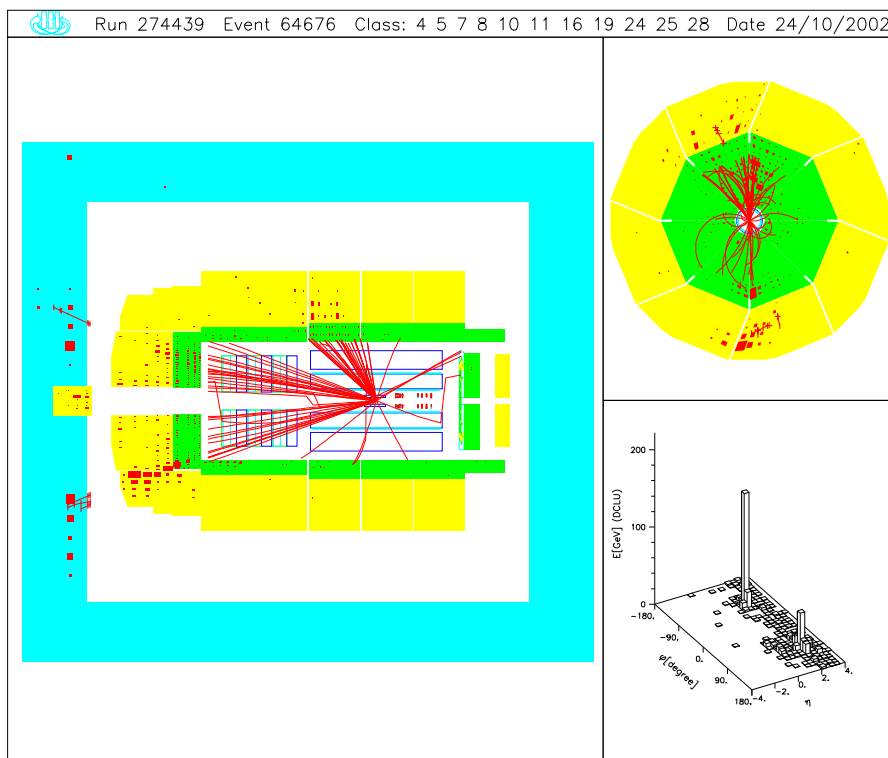
Figure E.5: t \rightarrow bW \rightarrow bq\bar{q}' candidate.
