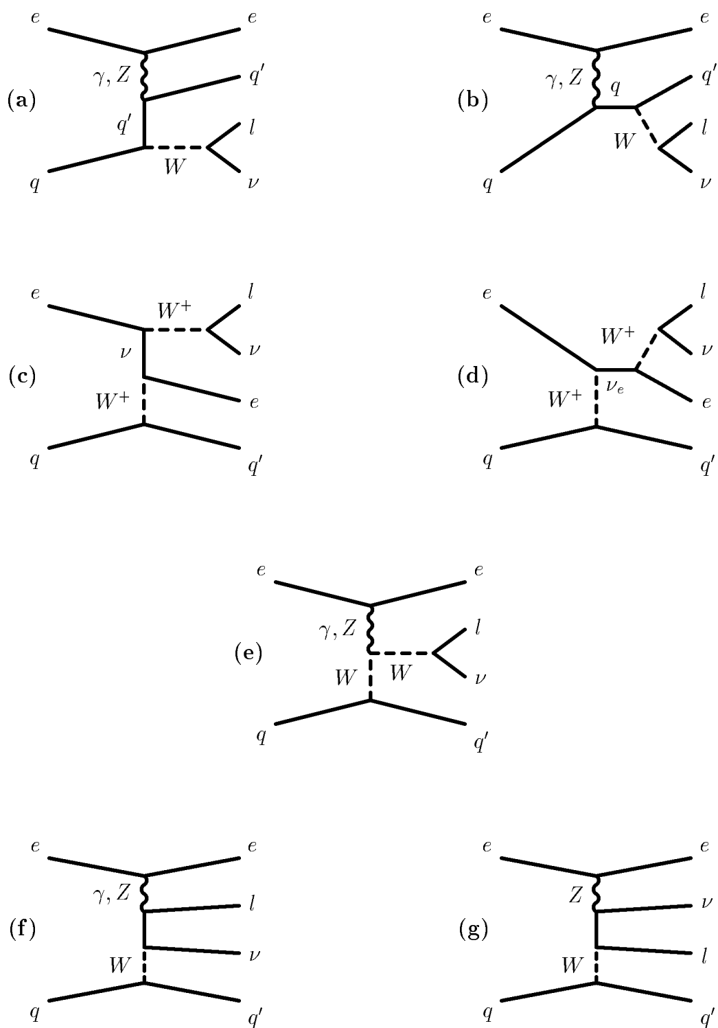
Figure 2.8: Leading order diagrams for W production in the process eq \rightarrow eq'lv .
