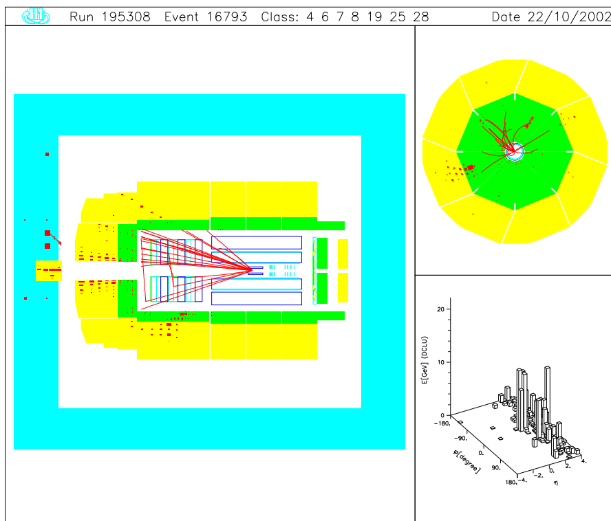
Figure A.5: W \rightarrow \mu^+ \nu candidate. P_T^\mu = 60_{-12}^{+19} \text{ GeV} , P_T^{\text{miss}} = 31 \text{ GeV} , P_T^{\text{jets}} = 26 \text{ GeV} , M_{e-\nu-\text{jets}} = 113 \text{ GeV} .
