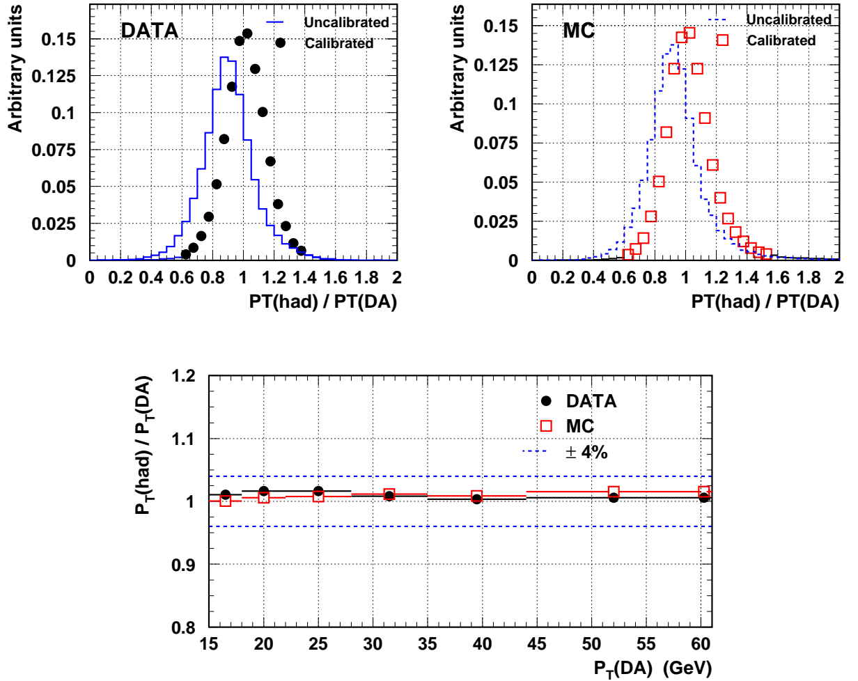
Figure 5.3: The P_T balance P_T^{\text{had}}/P_T^{DA} is shown for data and Monte Carlo before and after the calibration of the hadronic energy scale (upper plots). The lower plot shows the P_T balance as a function of P_T^{DA} .
