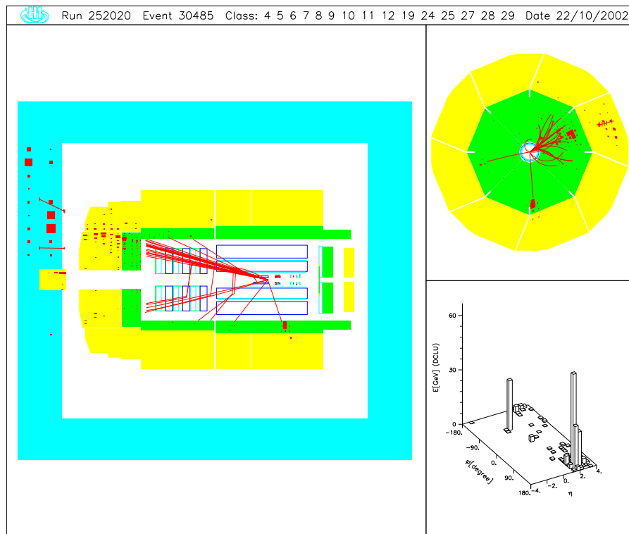
Figure A.3: W \rightarrow e^+\nu candidate with tagged scattered electron. ( top candidate )
