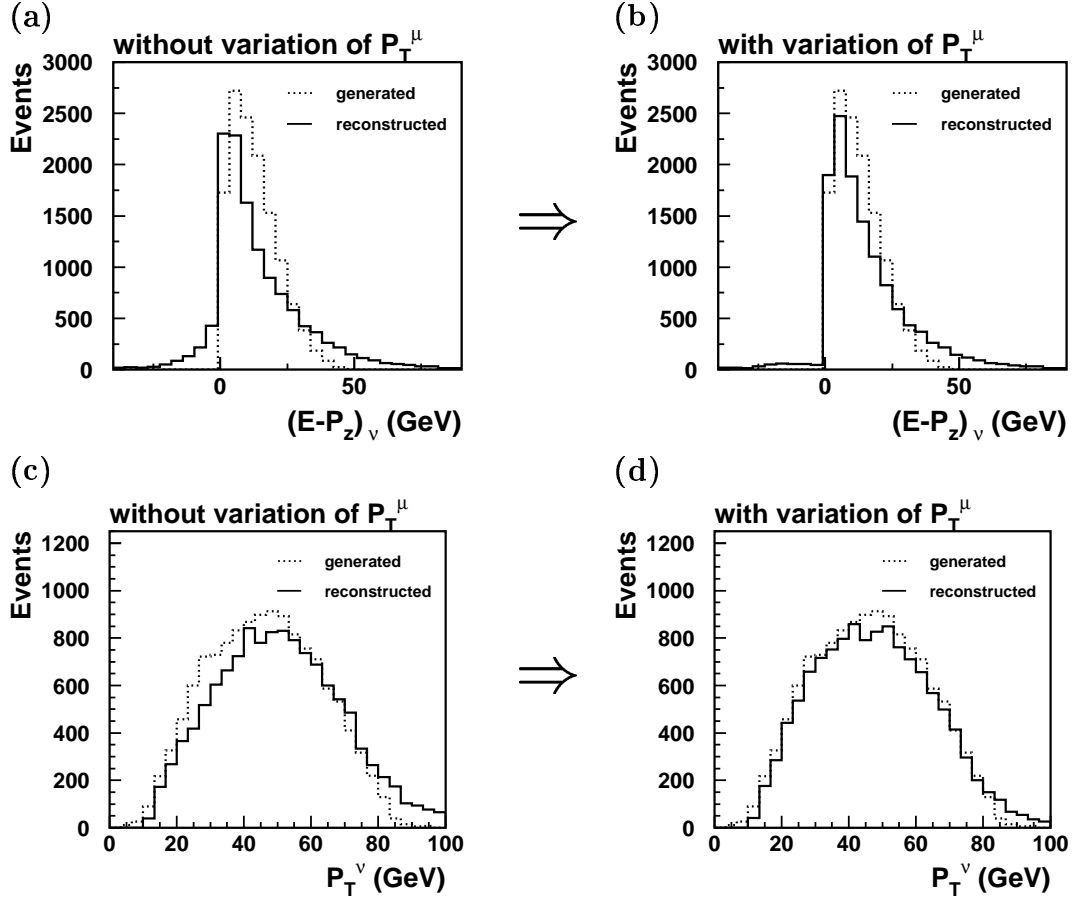
Figure 6.14: Monte Carlo distributions of the reconstructed (E - P_Z)_\nu and P_T^\nu for top events in the muon channel. The distributions are shown before and after a variation of the muon track momentum as described by equation 6.16. For events with two solutions for (E - P_Z)_\nu , one solution is chosen according to the prescription in table 6.6.
