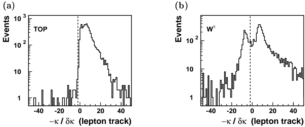
Figure 6.26: The significance of the charge determination of lepton tracks for (a) simulated top production and (b) simulated Standard Model W^\pm production. Positively charged tracks have values of \frac{-\kappa}{\delta\kappa} above zero, negatively charged tracks below zero. In (b) the two contributions from W^+ and W^- production are clearly separated. The cut on the lepton charge applied in the top analysis is indicated as a dashed line.
