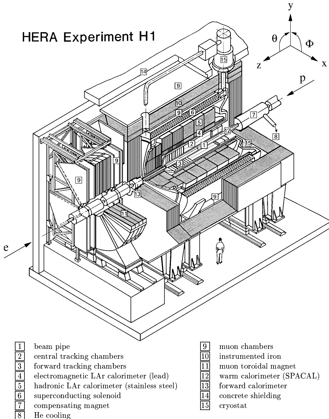
Figure 3.2: The H1-Detector.
