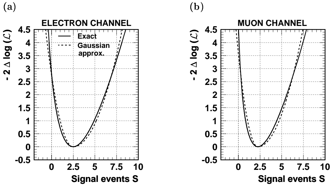
Figure 8.2: The log-likelihood functions of the signal fit in the in the electron (a) and muon (b) channels. They are shown as functions of the signal normalization. The exact log-likelihoods (solid lines) are compared to approximations (dashed lines) consisting of two half parabolas for each function (one on each side of the minimum).
