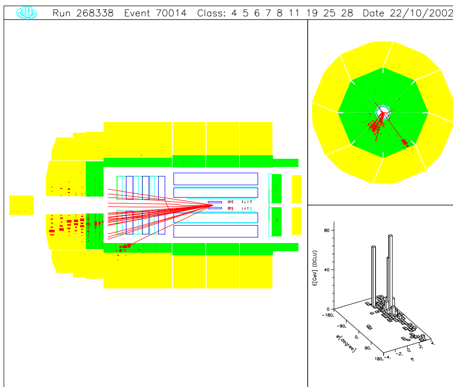
Figure A.4: W \rightarrow e^+ \nu candidate. ( top candidate ) P_T^e = 32 \text{ GeV} , P_T^{\text{miss}} = 67 \text{ GeV} , P_T^{\text{jets}} = 48 \text{ GeV} , M_{e-\nu-\text{jets}} = 160 \text{ GeV} .
