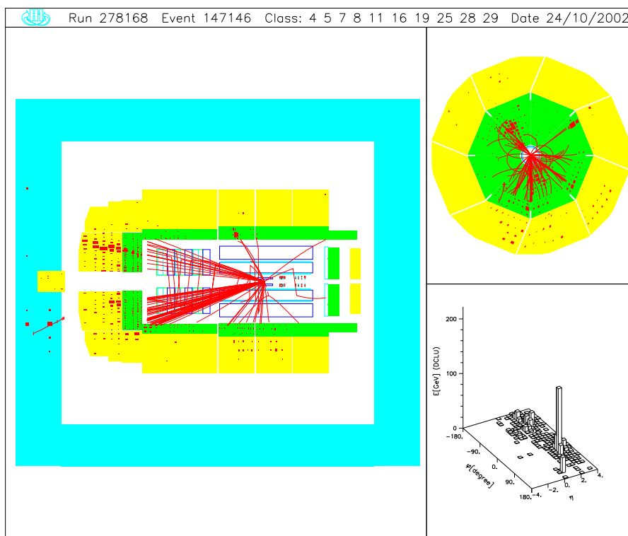
Figure E.4: t \rightarrow bW \rightarrow bq\bar{q}' candidate.
