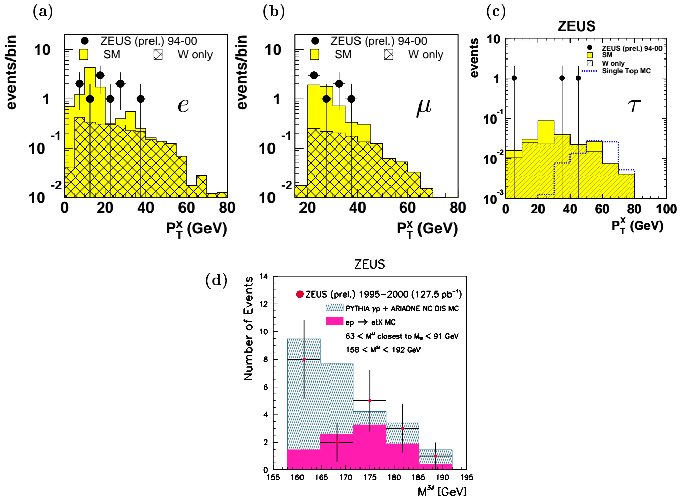
Figure 8.9: Preliminary results on isolated leptons and single top production obtained by the ZEUS collaboration. Shown are the hadronic transverse momentum distributions in the electron channel (a), muon channel (b), tau channel (c) and the 3-jet mass distribution in the hadronic channel (d). In (c) and (d), the top simulation is shown with arbitrary normalization. Taken from [75, 76].
