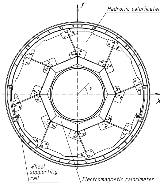
Figure 3.4: Transverse section of the Liquid Argon Calorimeter.
