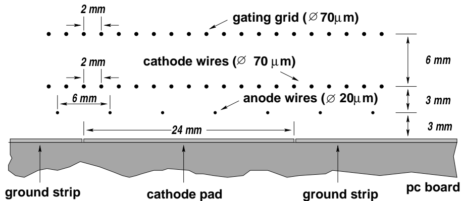
Figure 3.8: Cross section of the TPC readout chamber.
