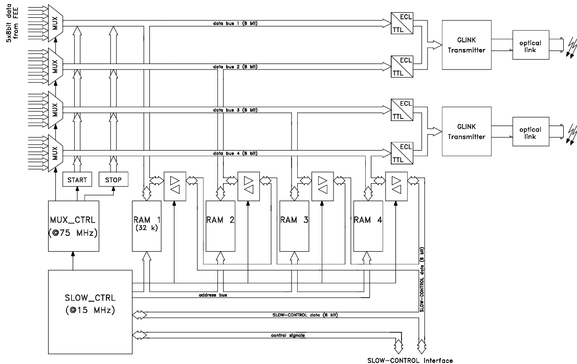
Figure 4.9: Schematic view of the Motherboard.
