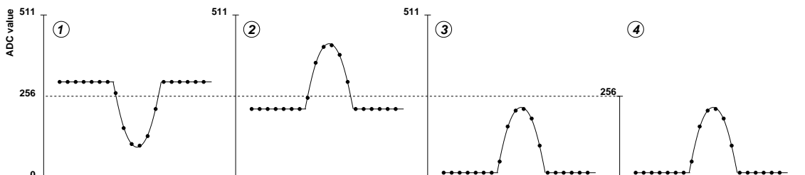
Figure 5.5: The different steps of signal processing inside the ALTRO chip.
