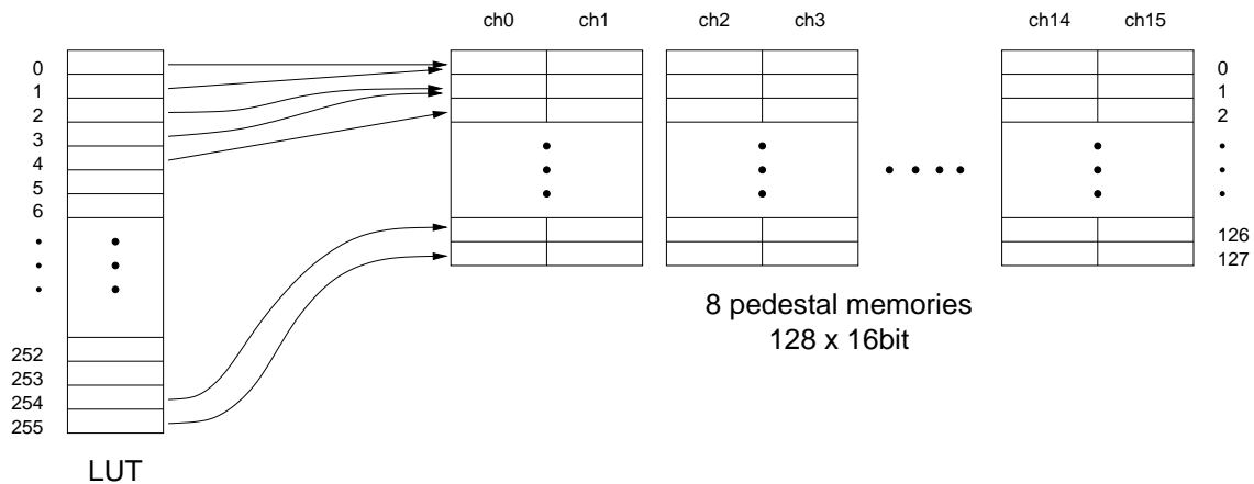
Figure 5.7: Implementation of the pedestal memory using a look-up table.
