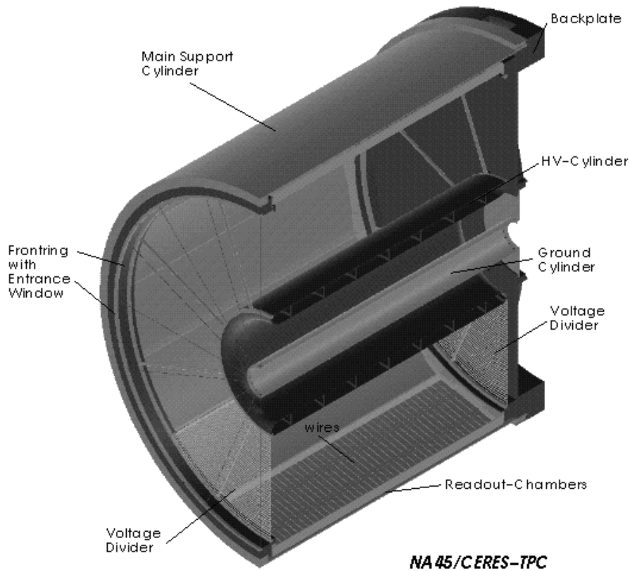
Figure 3.5: Perspective view of the TPC.
