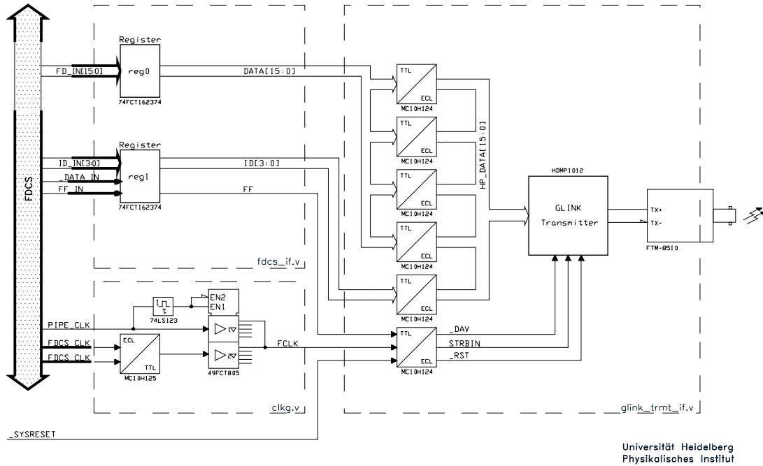
Figure 4.15: Transmitter part of the FDCS-to-PCI bridge.
