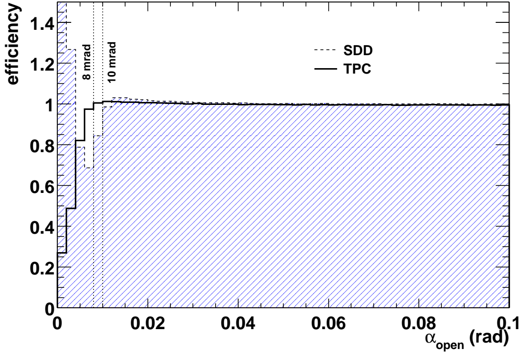
Figure 7.6: Two-track resolution of the TPC and the SDD as a function of opening angle.
