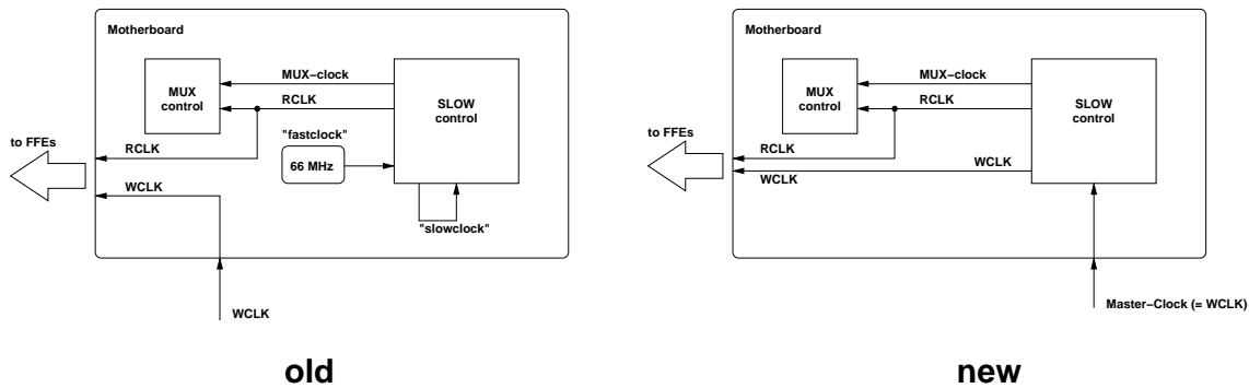
Figure 5.2: Clock distribution.
