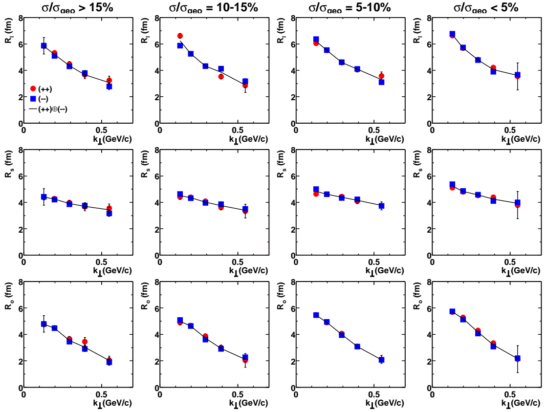
Figure 7.12: R_l , R_s , and R_o for (++) and (--) particle pairs for E_{\text{beam}} = 158 \text{ AGeV} . Also shown are the results for a combined analysis of both charges. All radii are not corrected for momentum resolution.
