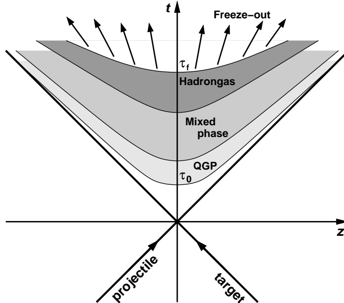
Figure 1.4: Evolution of a heavy ion collisions in Minkowski's representation of space-time.
