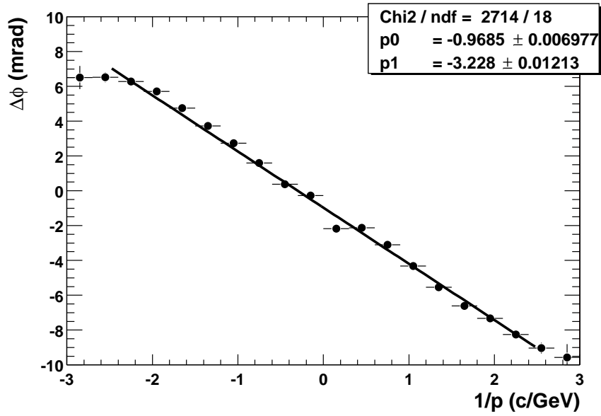
Figure 6.9: Influence of the fringe field on target tracks. Shown is the deflection \Delta\phi as a function of the inverse momentum. \Delta\phi(p^{-1}) is parameterized by a polynomial of first order.
