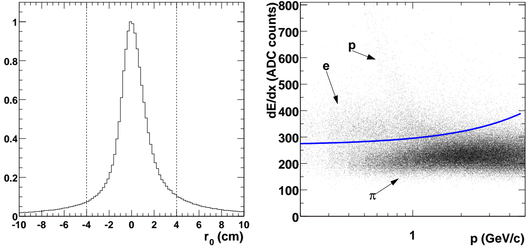
Figure 7.5: Track selection cuts for E_{\text{beam}} = 40 AGeV. Left: track offset r_0 at target. Right: energy loss dE/dx . The applied cut are indicated by the lines.
