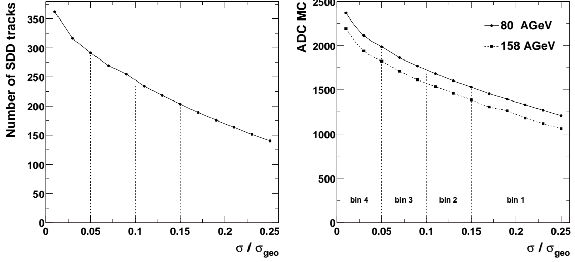
Figure 7.2: The number of SDD tracks and the ADC value of the MC detectors as a function of the centrality. The curves are obtained with the help of a detector simulation [79].
