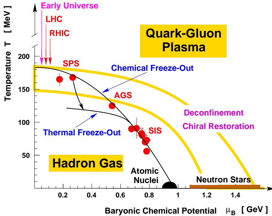
Figure 1.1: QCD phase diagram of hadronic matter [5].
