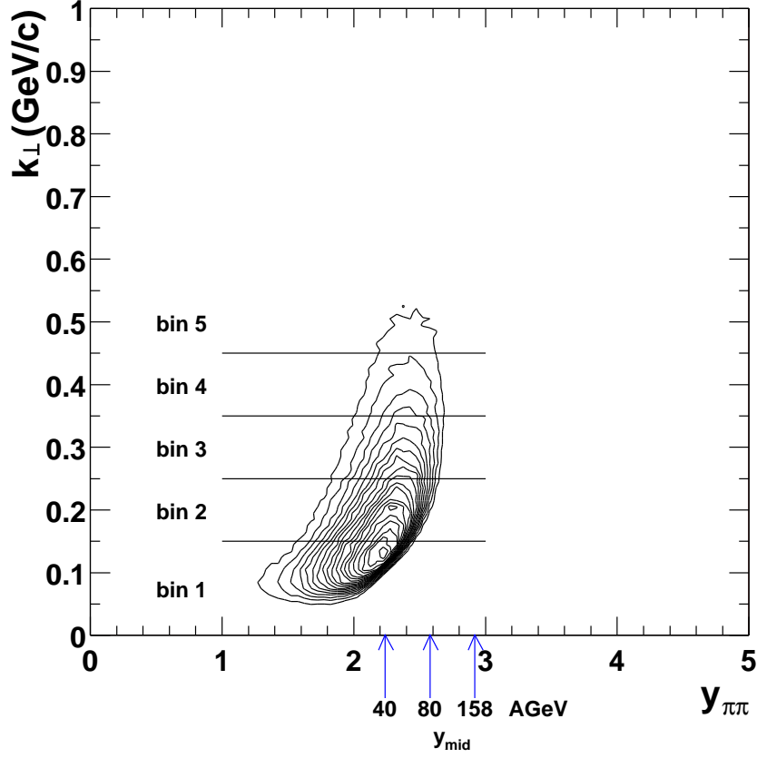
Figure 7.7: Acceptance for \pi\pi -pairs. Midrapidity for the three beam energies are indicated by the arrows. The bins in k_{\perp} are indicated by the horizontal lines.
