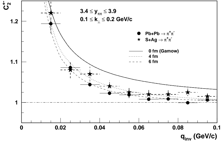
Figure 2.3: Measured two-particle correlation function C^{+-} for non-identical charged particles as a function of the relative pair momentum q_{\text{inv}} . Also shown are the calculated correlation functions based upon the Coulomb interaction for a point-like source (solid line) and finite-sized sources of radii 4 fm (dotted line) and 6 fm (dashed line). The Figure is taken from [50].
