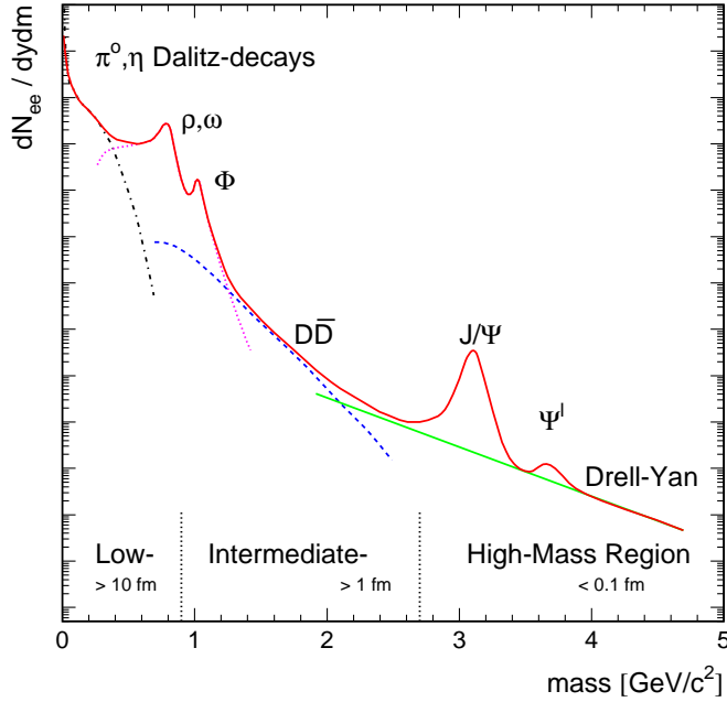
Figure 1.5: Schematic dilepton mass spectrum.
