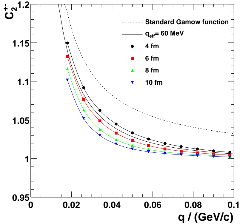
Figure 2.4: Calculated C^{+-} correlation functions for different source sizes. The standard Gamow function and the parameterization according to (2.60) with q_{\text{eff}} = 60 MeV are shown for comparison. Results are from [52].
