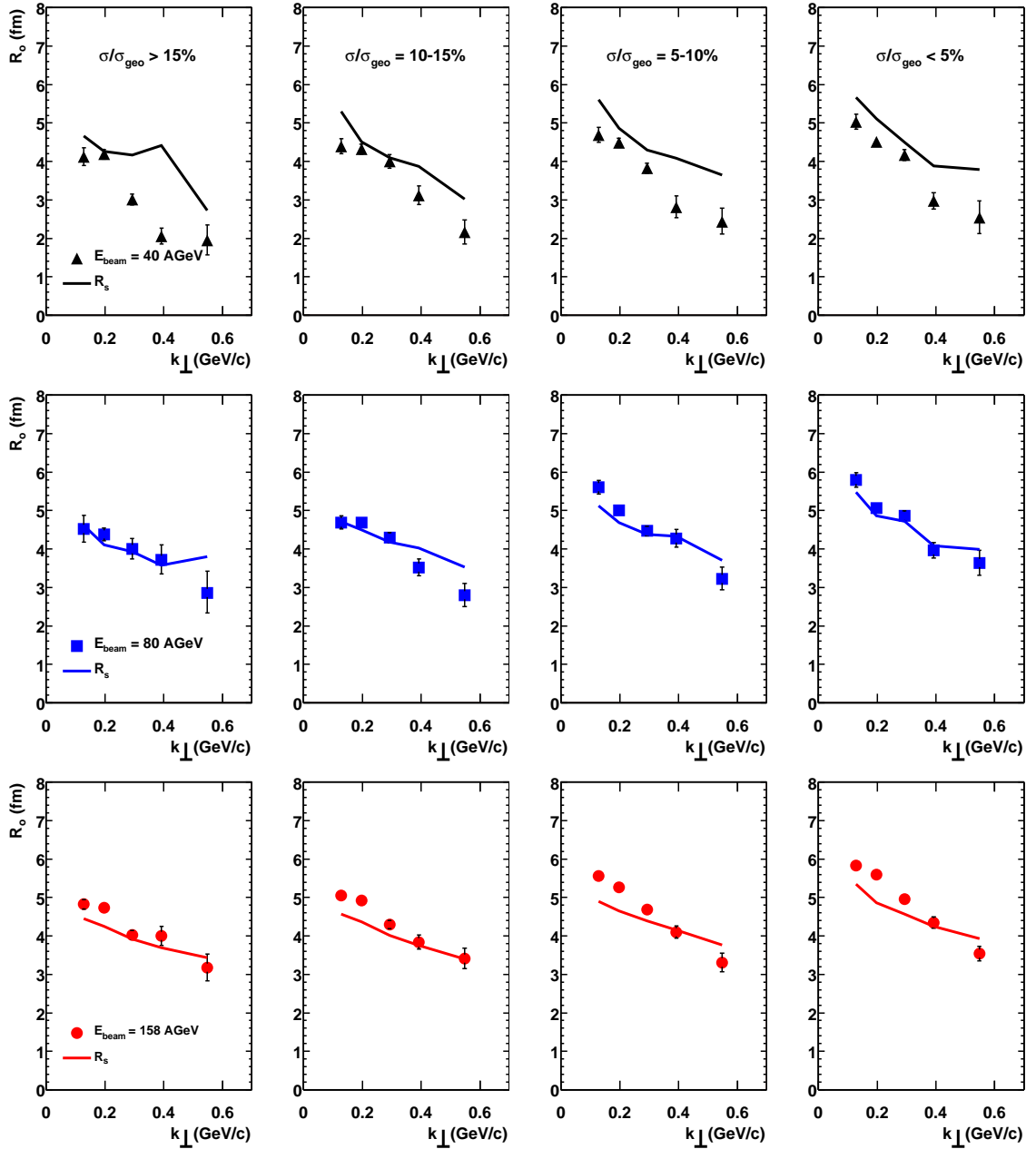
Figure 8.4: R_o for 40, 80, and 158 AGeV beam energy (from top to lower panel). The radii are shown vs. k_{\perp} for different centralities. The lines show the results of R_s for comparison.
