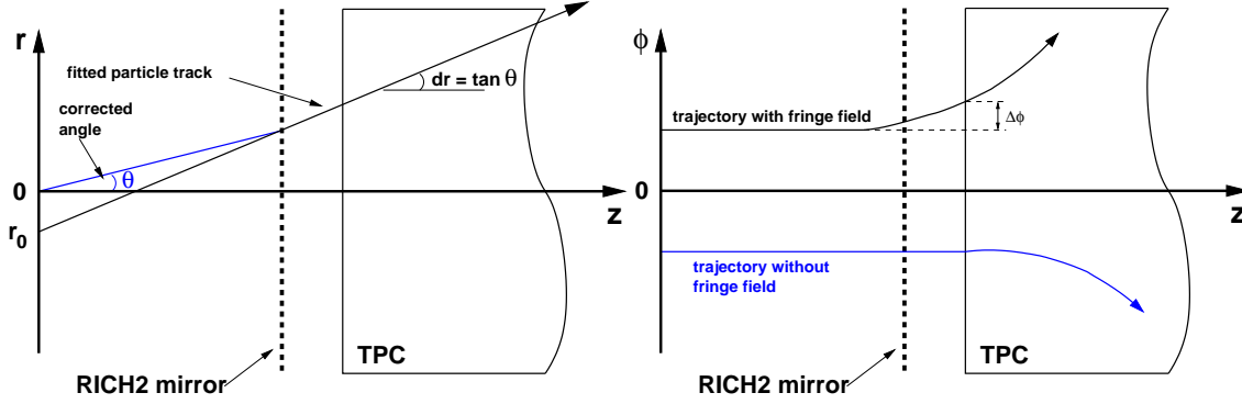
Figure 6.4: Momentum fit.
