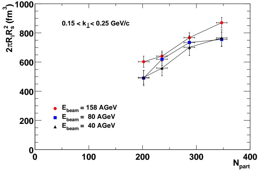
Figure 8.12: The effective volume V_{\text{eff}} as a function of N_{\text{part}} for different beam energies.
