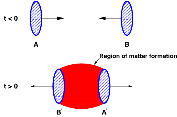
Figure 1.3: Schematic representation of an ultrarelativistic nucleus-nucleus collision in Bjorken's description. Due to the Lorentz contraction in longitudinal direction the colliding nuclei are reduced to thin disks.
