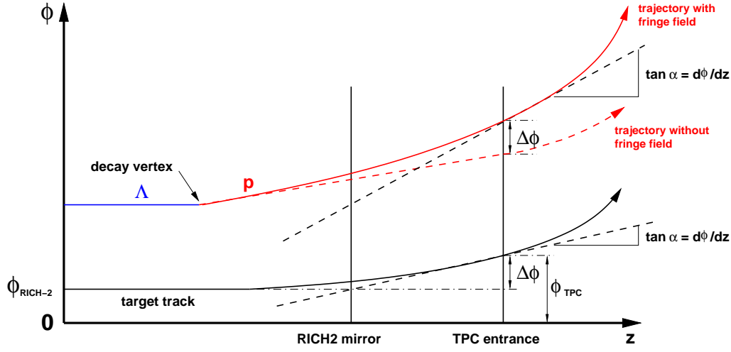
Figure 6.8: Effect of the fringe field on target tracks and tracks coming from secondary vertices (in this case from the decay of a \Lambda ), both with the same momentum. The measured \Delta\phi for the target track is also used to correct the trajectory of the secondary particle.
