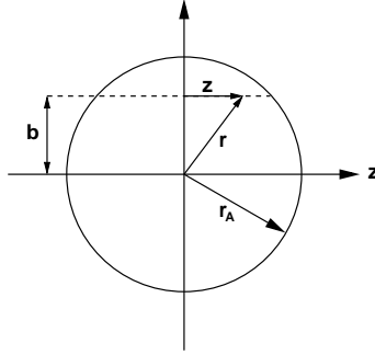
Figure 7.3: The thickness function.
