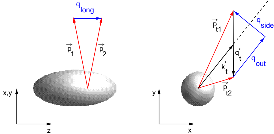
Figure 2.2: Coordinate system according to Bertsch-Pratt parameterization.
