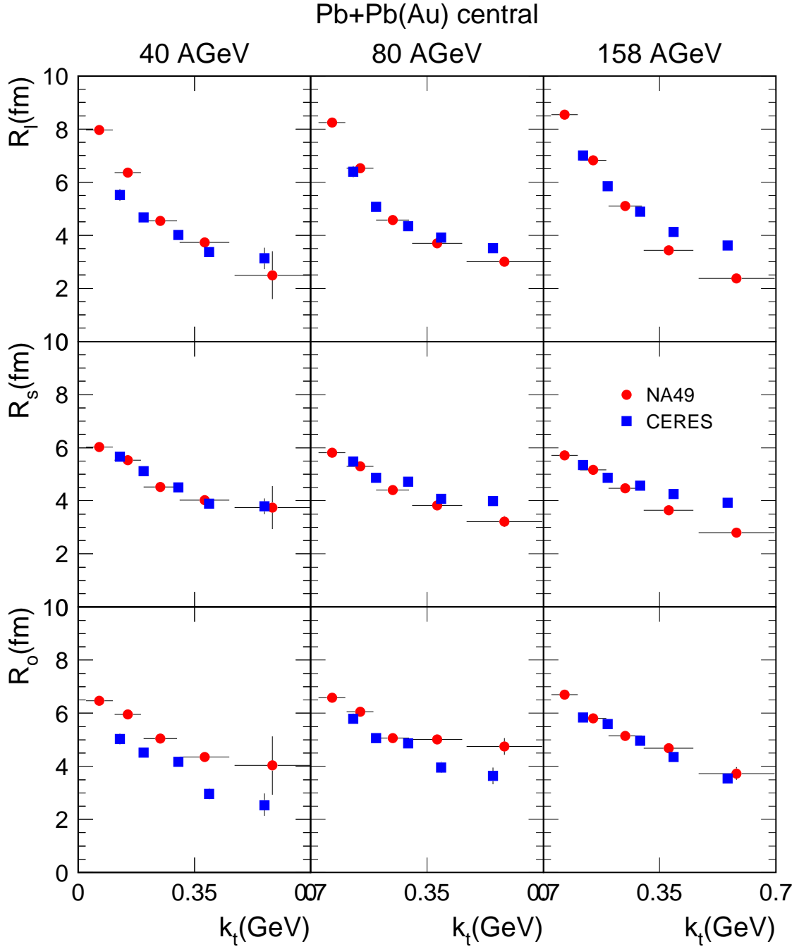
Figure 8.15: Comparison of HBT radii with results from NA49.
