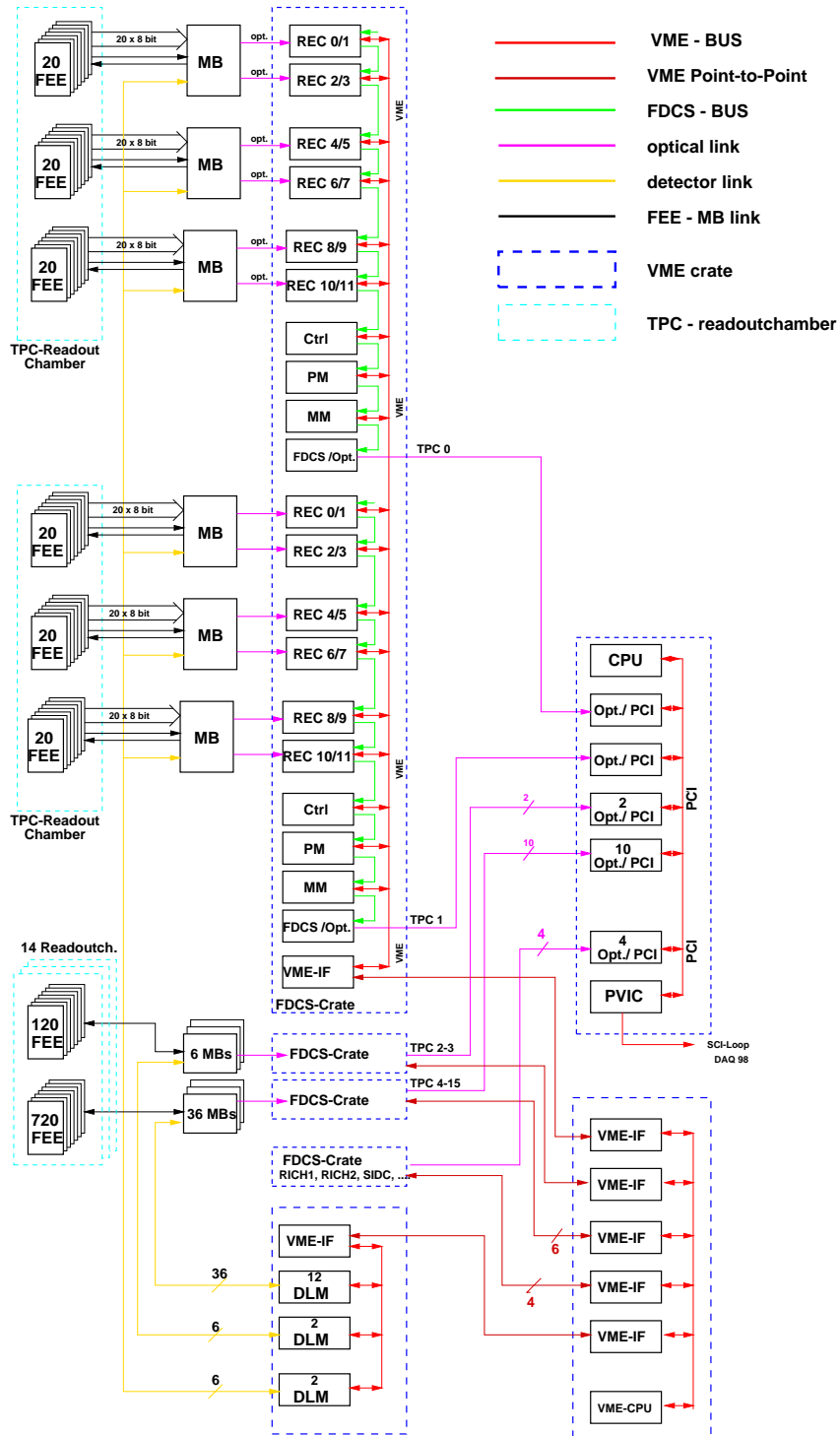
Figure 4.1: Overview of the complete readout tree for the TPC.
