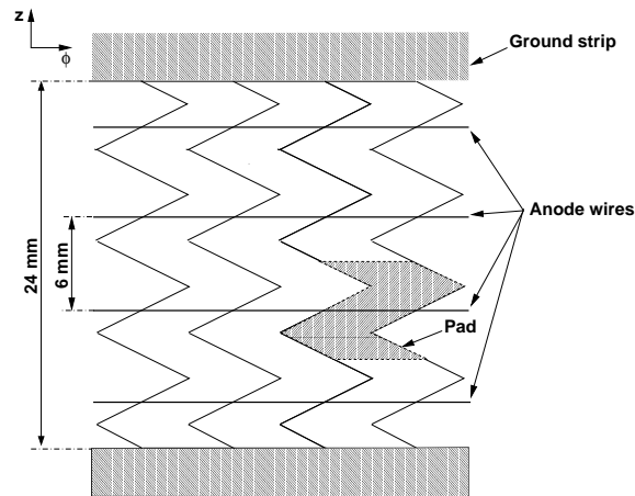
Figure 3.10: Layout of the pad plane. Four chevron structures are connected to one readout channel which is framed by ground stripes.
