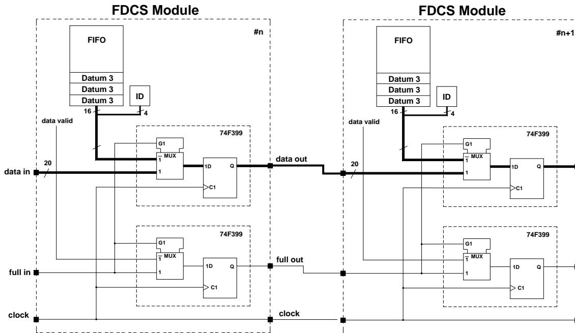
Figure 4.17: Schematic picture of the FDCS .
