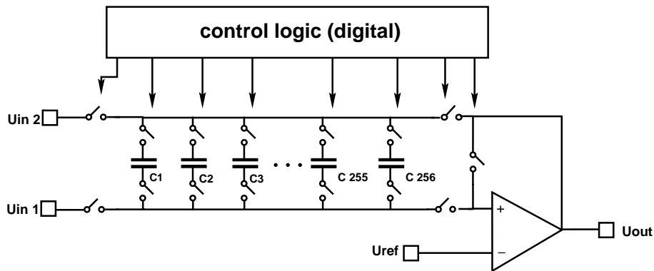
Figure 4.8: Schematic view of the SCA.
