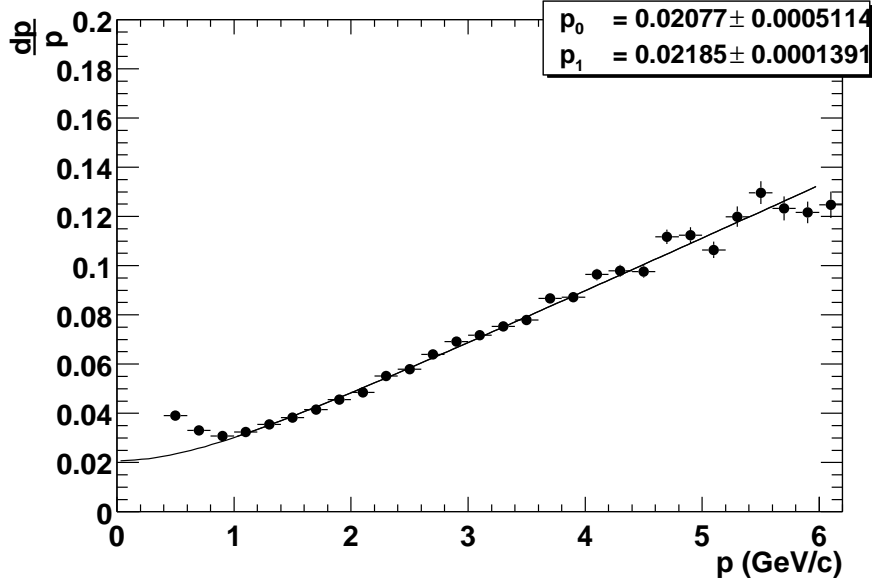
Figure 6.6: Momentum resolution of the TPC.
