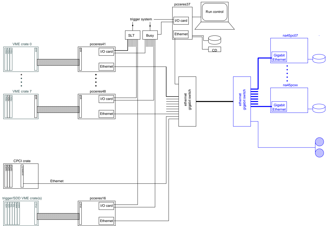
Figure 5.1: Overview of the CERES data acquisition in 2000.
