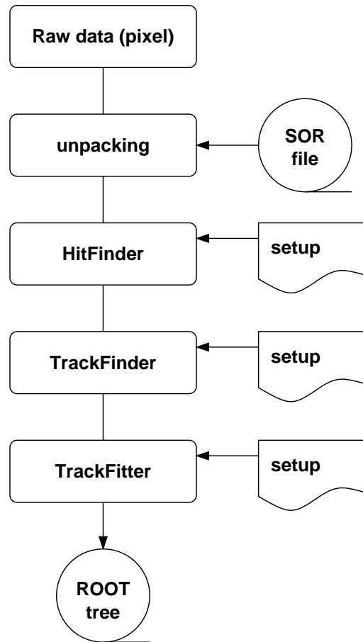
Figure 6.2: Schematic view of the different steps in the reconstruction chain. During unpacking, all information about the detector calibration is read from the Start Of Run (SOR) file. The setup files contain data (e. .g. threshold values) which control the behavior of the analysis steps.
