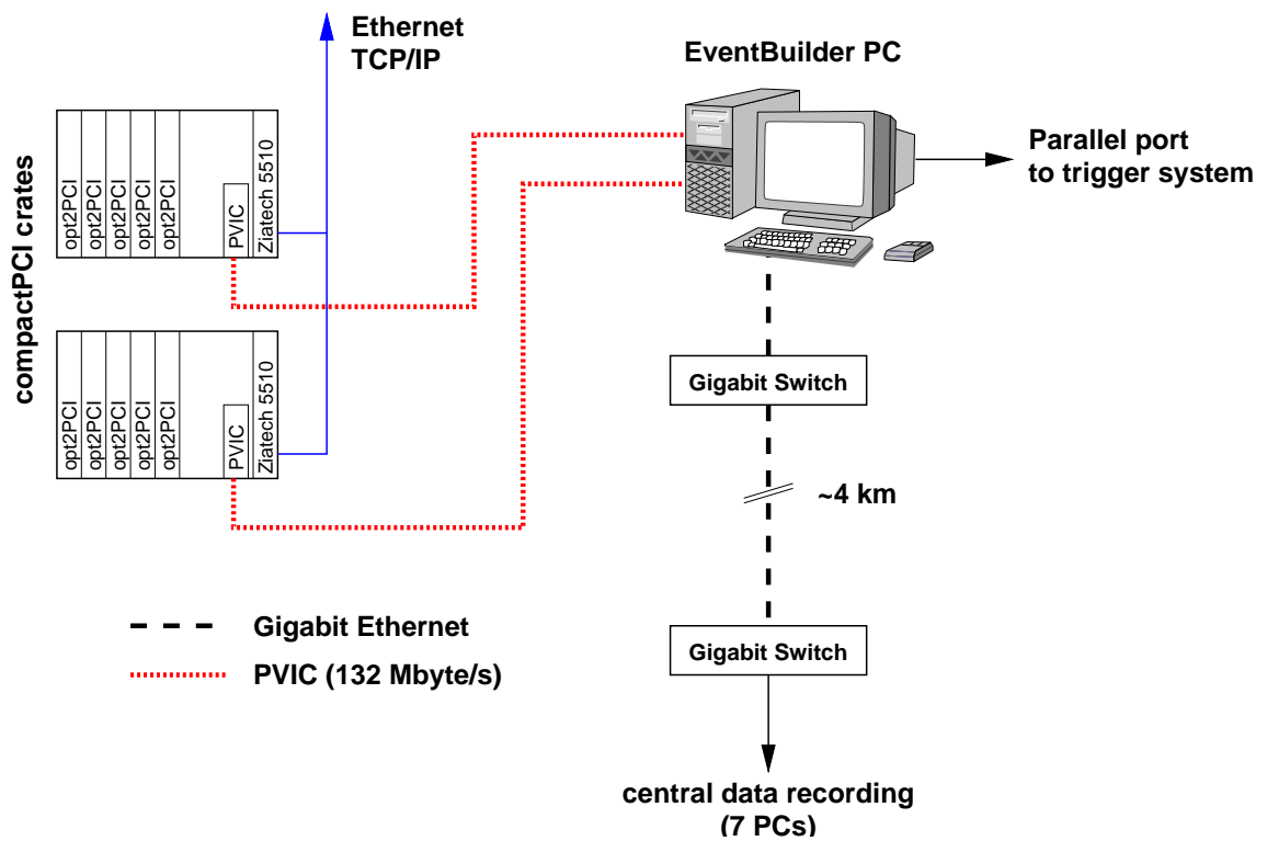
Figure 4.18: The interface of the readout electronic to central data recording.
