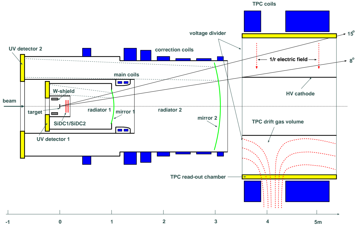
Figure 3.1: Schematic view of the CERES spectrometer.
