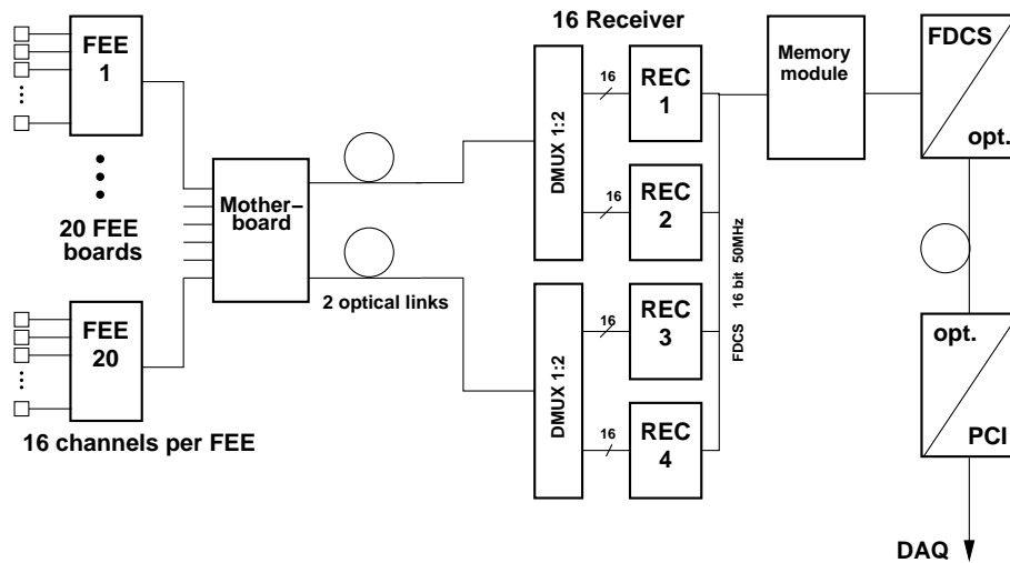
Figure 4.11: Data-path for one MotherBoard .
