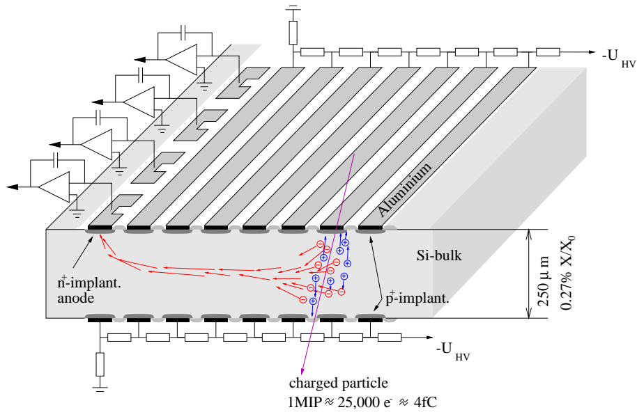
Figure 3.3: Working principle of the Silicon Drift Detectors.
