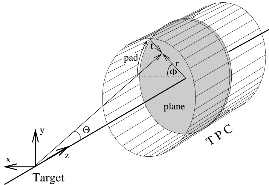
Figure 3.6: The coordinate system of the TPC.
