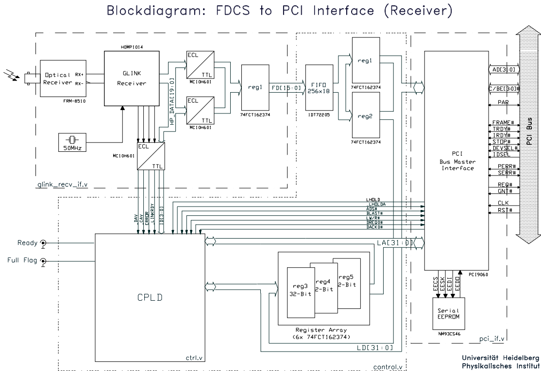
Figure 4.16: The receiver part of the FDCS-to-PCI bridge.
