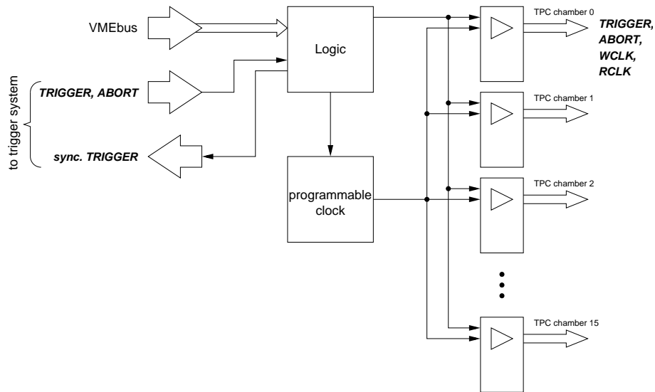
Figure 4.10: Schematic of the ClockModule .
