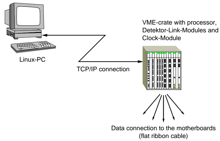
Figure 5.10: Client-server architecture of the TPC software.
