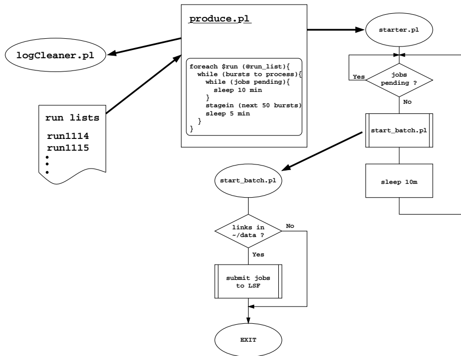
Figure 6.1: Production of the raw data is done in a automated way and controlled by simple Perl scripts.
