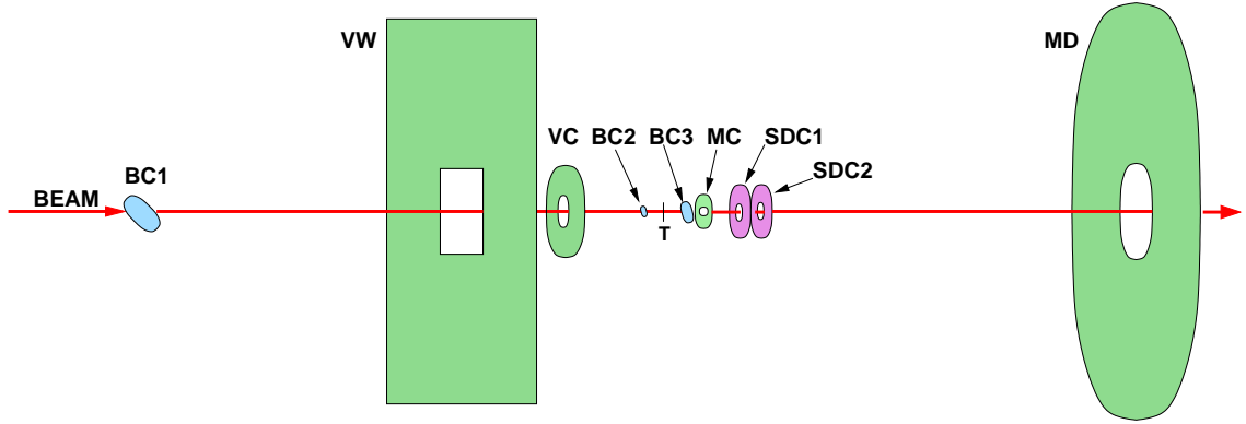
Figure 3.2: Schematic view of the target region with the trigger detectors.
