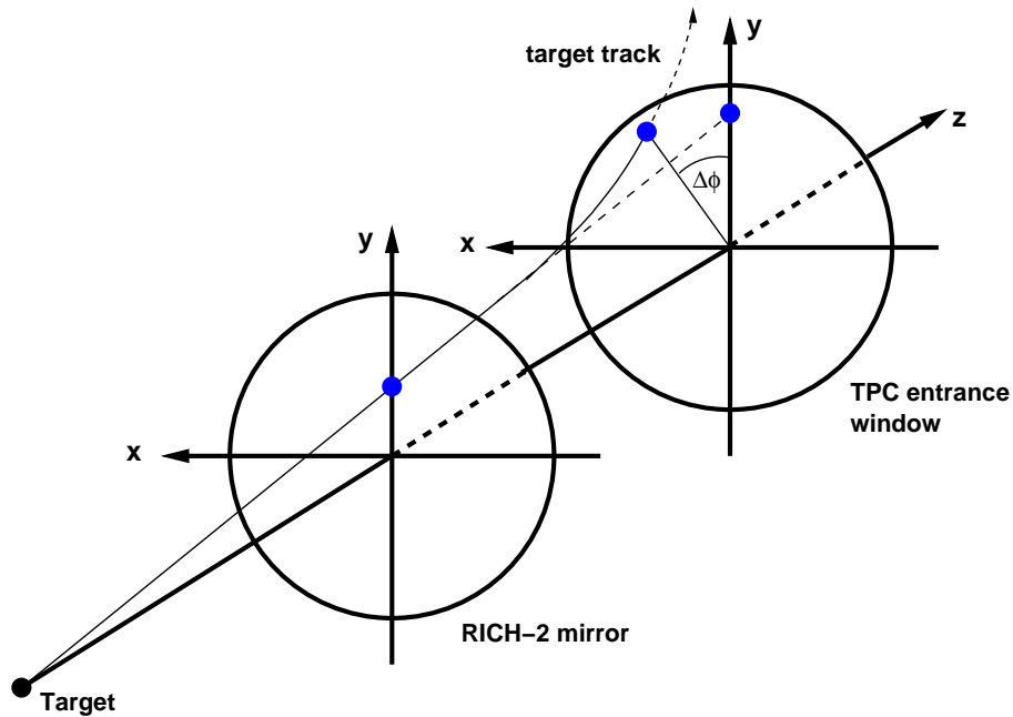
Figure 6.7: Effect of the fringe field on tracks. The remnant magnetic field in front of the TPC entrance window is bending charged particles in \phi direction. \phi(z) is no longer constant and the particles enter the TPC with some slope d\phi/dz .
