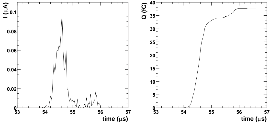
Figure 4.4: Simulated pad-signal. The current is shown in the left Figure. The right Figure shows the accumulated charge.
