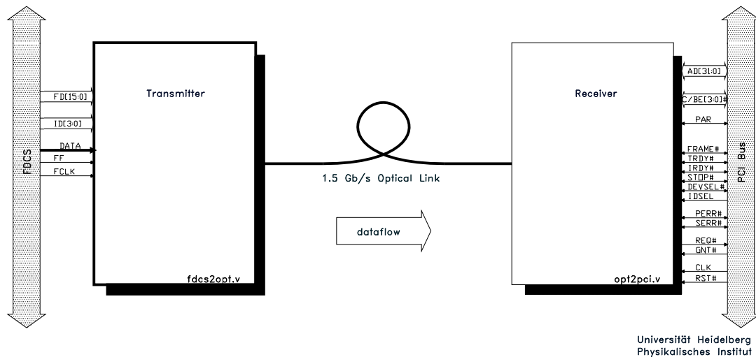
Figure 4.14: Block diagram of the FDCS-to-PCI interface.
