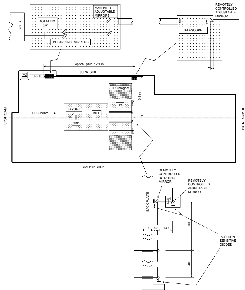
Figure 3.11: Overview of the laser system.
