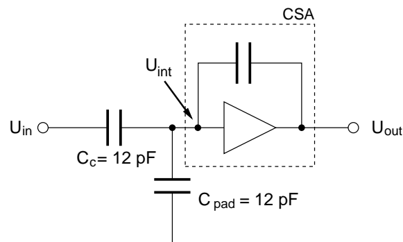
Figure 4.5: Circuit for stimulating the amplifier with realistic signals.
