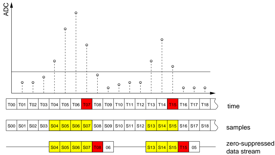
Figure 5.6: Zero suppression. Trigger at t = 0 .
