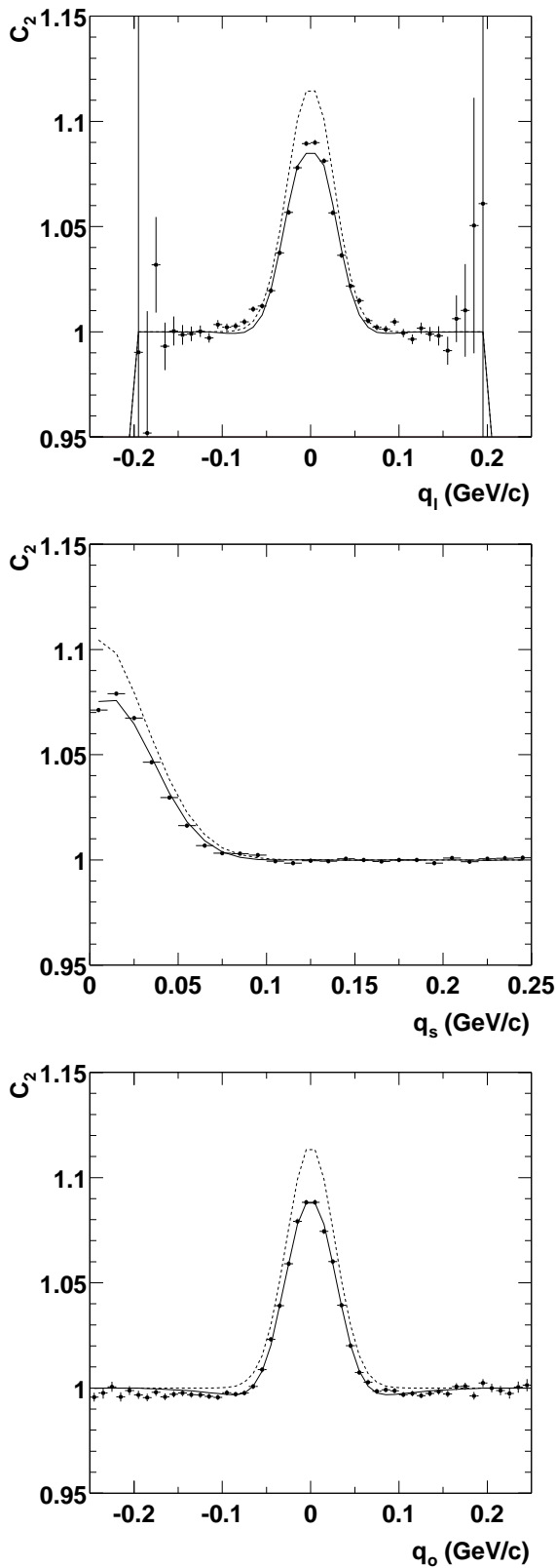
Figure 7.8: One-dimensional projections of the three-dimensional correlation function C_2 in the Bertsch-Pratt parameterization. The solid lines show the fit of (7.13) to the data points. For comparison also the parameterization (7.13) without Coulomb correlations are shown by the dashed lines.
