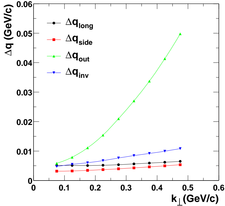
Figure 7.9: Resolution of the long -, side -, out -components of the momentum difference as a function of the mean transverse pair momentum k_{\perp} .
