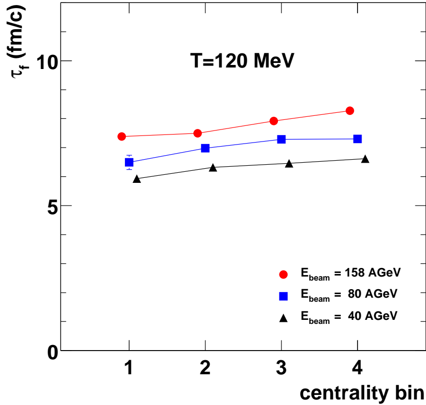
Figure 8.2: Freeze-out time \tau_f as a function of centrality of the collision.
