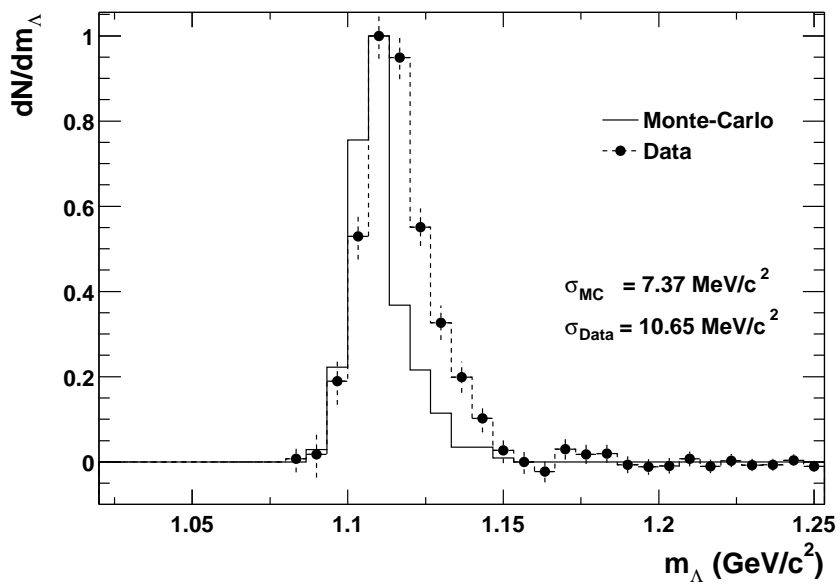
Figure 6.10: Invariant mass spectrum of the \Lambda . Shown are the results of a Monte-Carlo simulation of the TPC (solid line) and the mass spectrum as reconstructed from data (points and dashed line).
