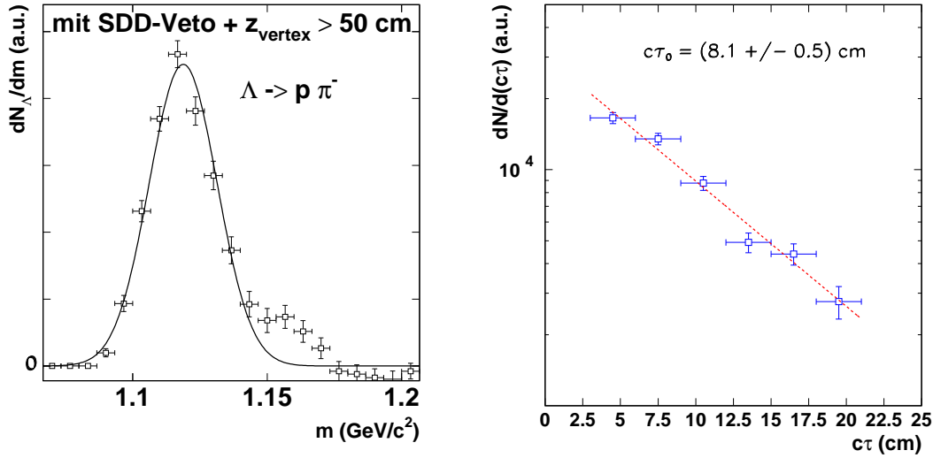
Figure 1.7: The reconstructed mass and lifetime of the \Lambda hyperon at a beam energy of 40 AGeV. Figures are from [25].
