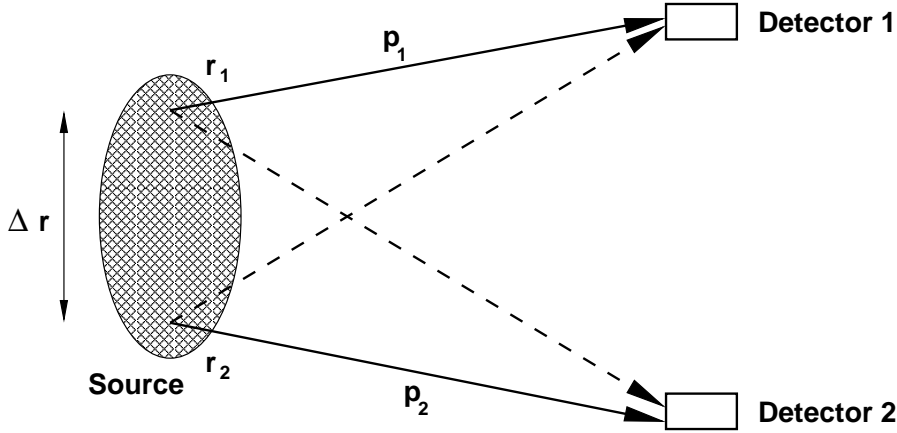
Figure 2.1: Schematic representation of the emission of two indistinguishable particles from two points \vec{r}_1 and \vec{r}_2 of the source. The momenta of the two particles are measured with two detectors.
