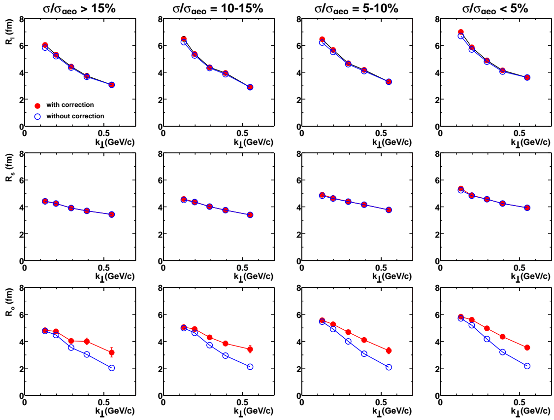
Figure 7.11: Comparison of uncorrected and corrected HBT radii for E_{\text{beam}} = 158 AGeV.
