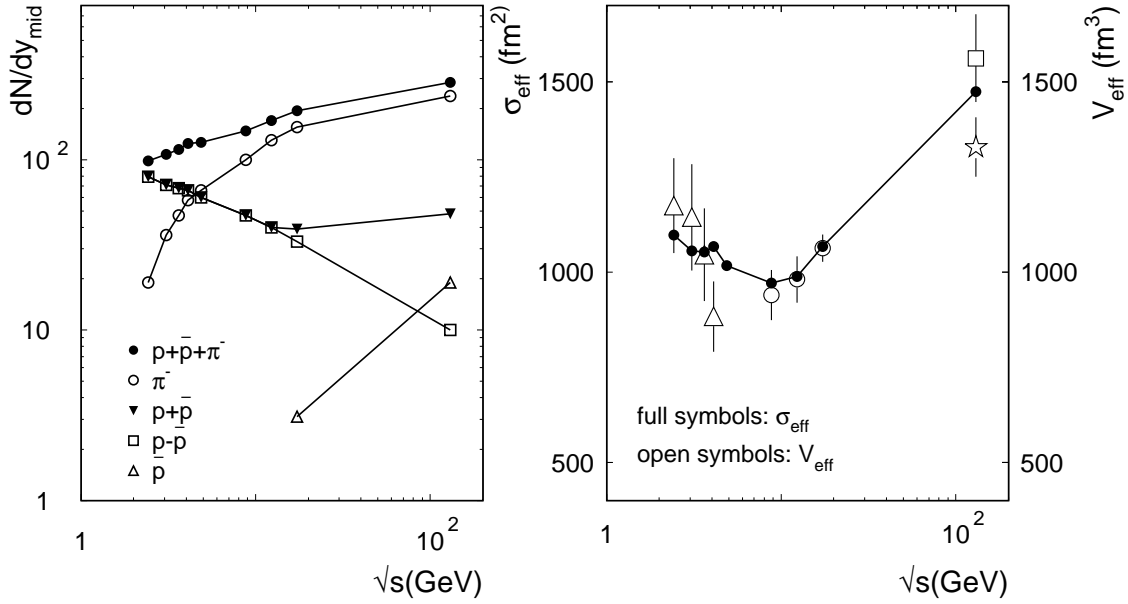
Figure 8.14: Left: Midrapidity yields of protons, anti-protons and negative pions as a function of \sqrt{s} . Right: Effective particle number \sigma_{\text{eff}} and effective volume V_{\text{eff}} vs. \sqrt{s} .
