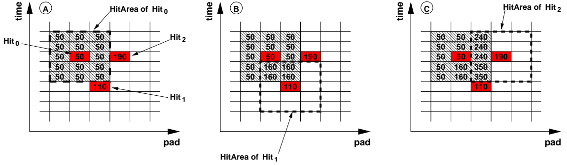
Figure 6.3: Example for the treatment of overlapping hits in the HitFinder . The flags in the HitArea of \text{Hit}_0 are filled with its maximum amplitude plus the maxima for the overlapping hits \text{Hit}_1 and \text{Hit}_2 .
