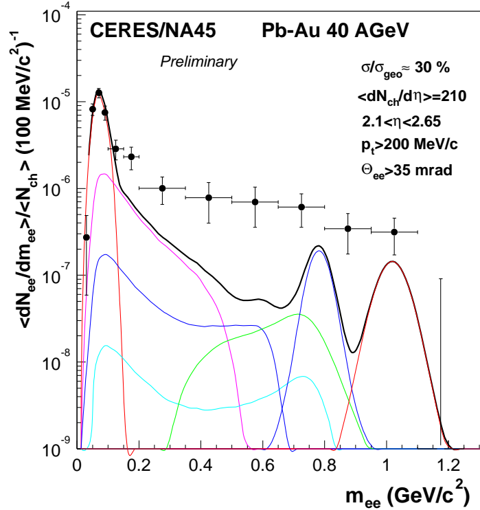
Figure 1.6: Invariant mass spectrum of e^+e^- pairs recorded in central Pb-Au collisions at 40 AGeV.
