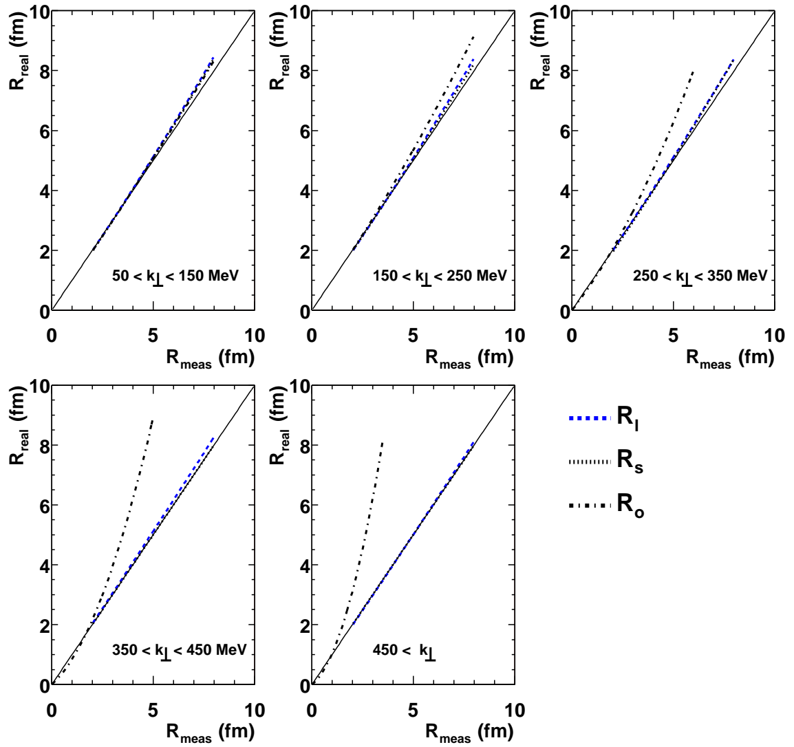
Figure 7.10: Deviation of the reconstructed radii R_{\text{meas}} from the real radii R_{\text{real}} due to the finite momentum resolution of the TPC.
