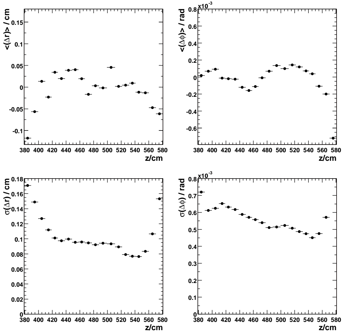
Figure 6.5: Residuals of the track fit for runs at beam energy of 158 AGeV with magnetic field.
