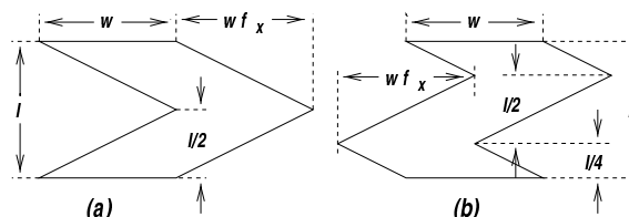
Figure 3.9: Chevron pads.
