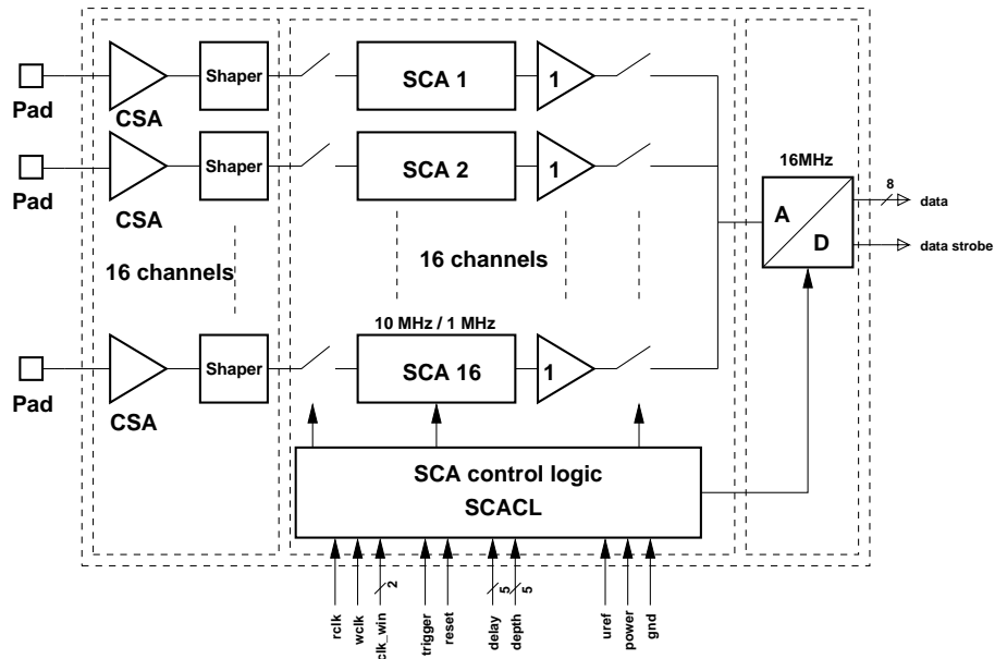
Figure 4.2: Sketch of a FEEboard.
