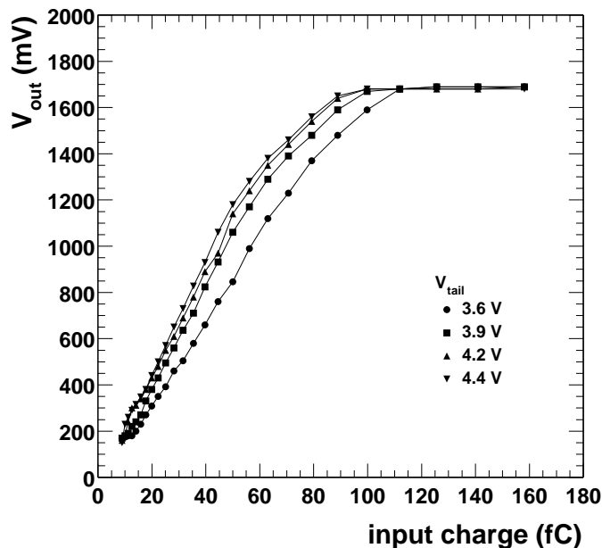
Figure 4.7: Linearity of the preamplifier.
