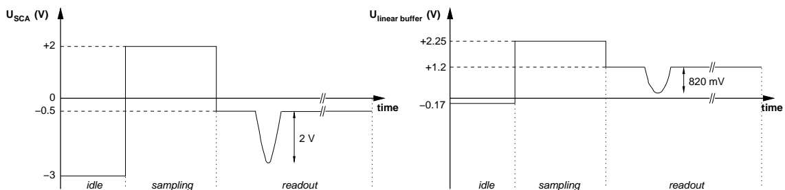
Figure 5.3: The main purpose of the linear buffer is to adjust the output signal of the SCA to the input of the FEDC.
