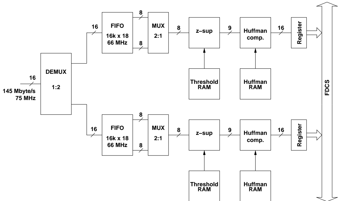
Figure 4.12: Schematic view of the Receiver board.
