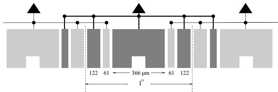
Figure 3.4: Anode structure of the SDD.
