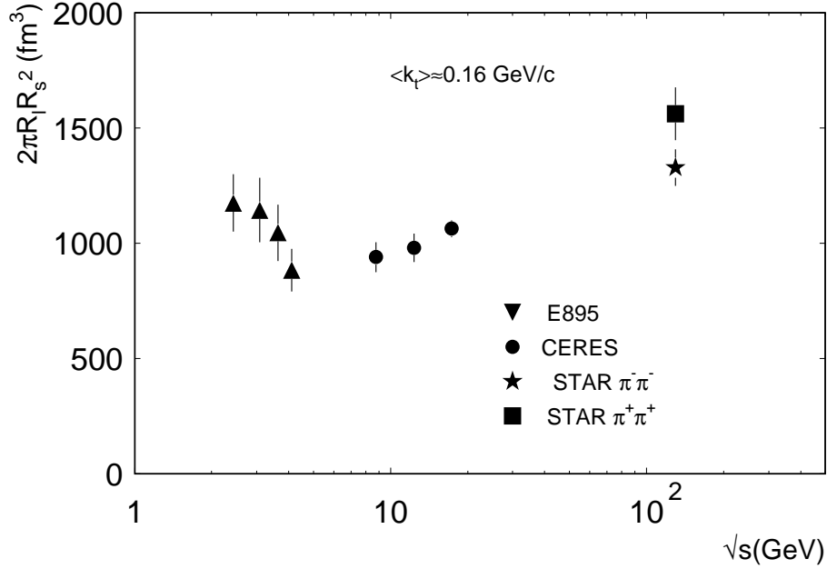
Figure 8.13: The effective volume V_{\text{eff}} as a function of \sqrt{s} . The data points from the experiment E895 are at a mean transverse pair momentum \langle k_{\perp} \rangle = 0.15 \text{ GeV}/c [95], STAR is at \langle k_{\perp} \rangle = 0.17 \text{ GeV}/c [96], and the CERES points are the average of the k_{\perp} bins at \langle k_{\perp} \rangle = 0.12 \text{ GeV}/c and \langle k_{\perp} \rangle = 0.2 \text{ GeV}/c .
