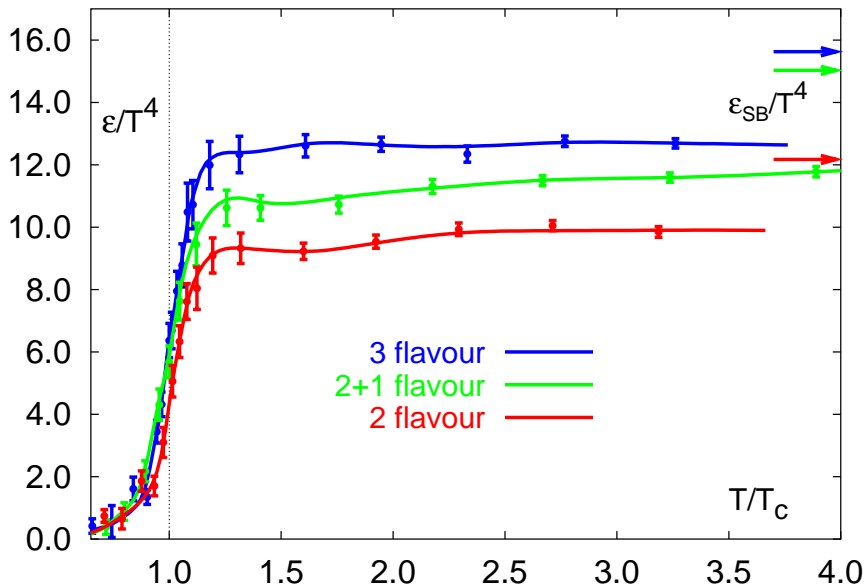
Figure 1.2: Result of lattice QCD calculations for the energy density \varepsilon (in units of T^4 ) as a function of the temperature T (in units of the critical temperature T_c ). Here \varepsilon is shown for different numbers of quark flavors where 2 + 1 means two light and one heavy flavors (Figure from [11]).
