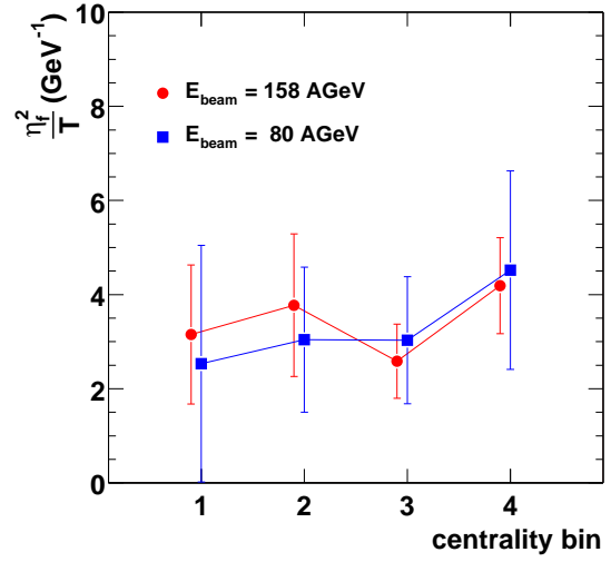
Figure 8.8: The fit parameter \eta_f^2/T_f for the different centrality bins.
