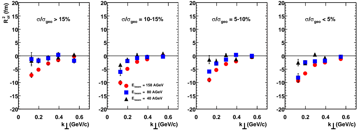
Figure 8.6: The cross-term R_{ol}^2 .
