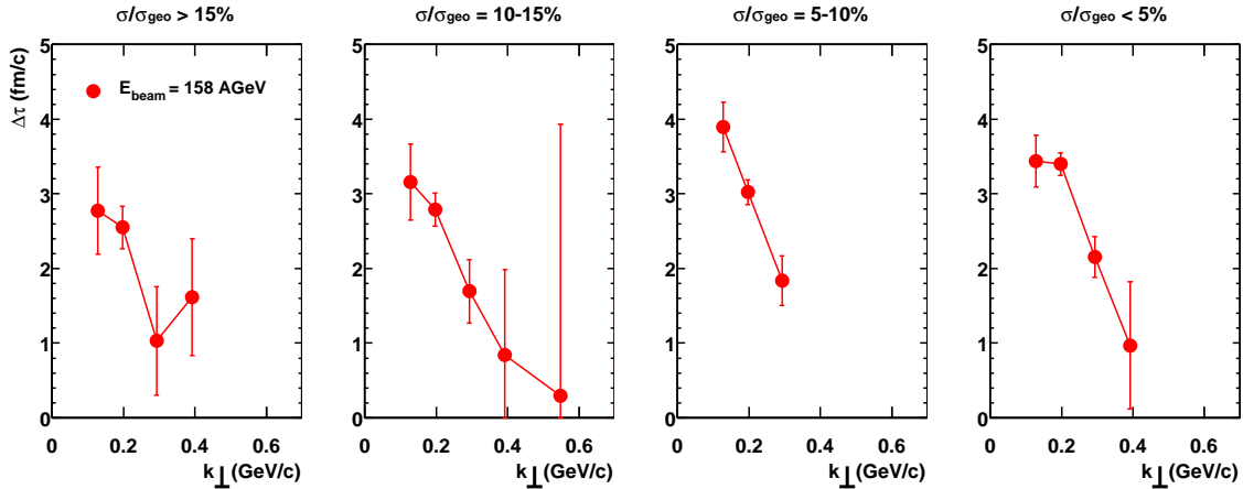
Figure 8.5: Duration of particle emission \Delta\tau for beam energy of 158 AGeV.
