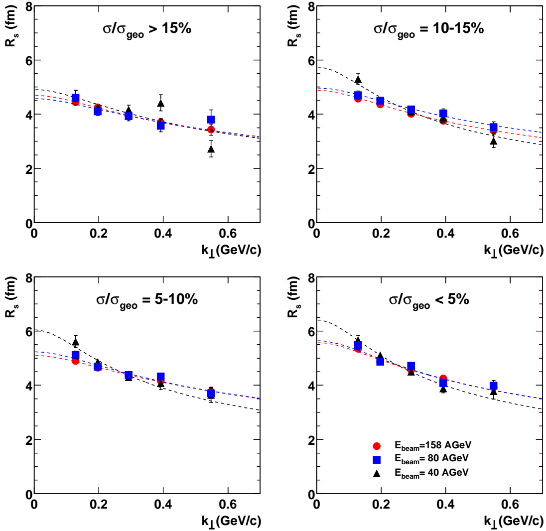
Figure 8.3: R_s as a function of k_{\perp} for the three beam energies and the different multiplicity bins.
