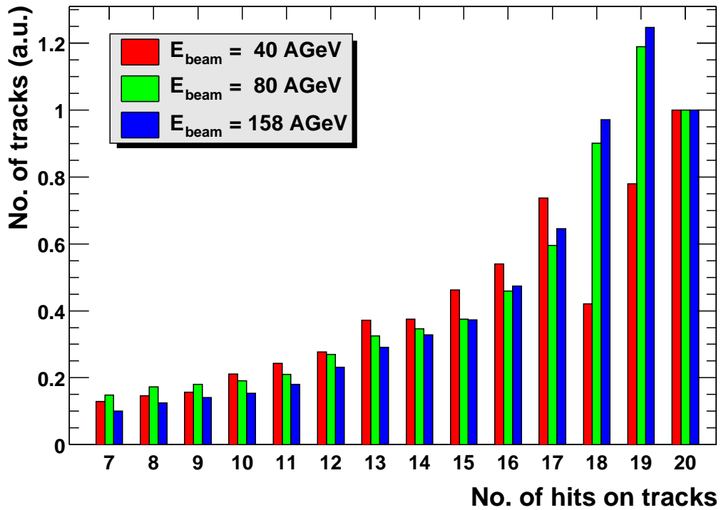
Figure 7.4: Distribution of track lengths, measured in number of hits. The distributions for the different beam energies are arbitrarily normalized to 1 at a track length of 20 hits.
