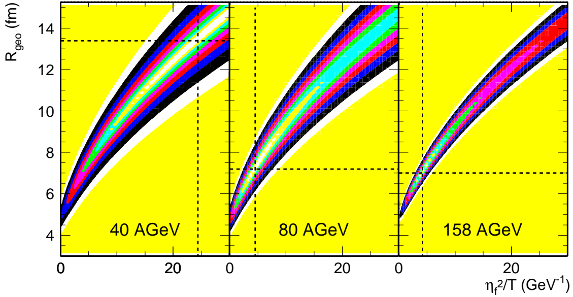
Figure 8.10: Contour plot of \chi^2 , obtained by fitting (8.4) to R_s .
