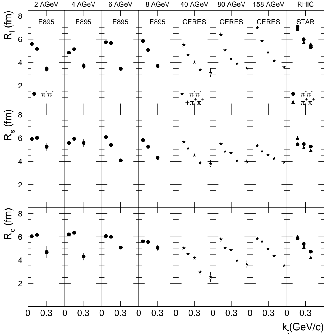
Figure 8.11: k_{\perp} dependence of HBT radii in central Pb-Pb, Au-Au, and Pb-Au (CERES) collisions at different beam energies. RHIC and AGS data are taken from [95, 96].
