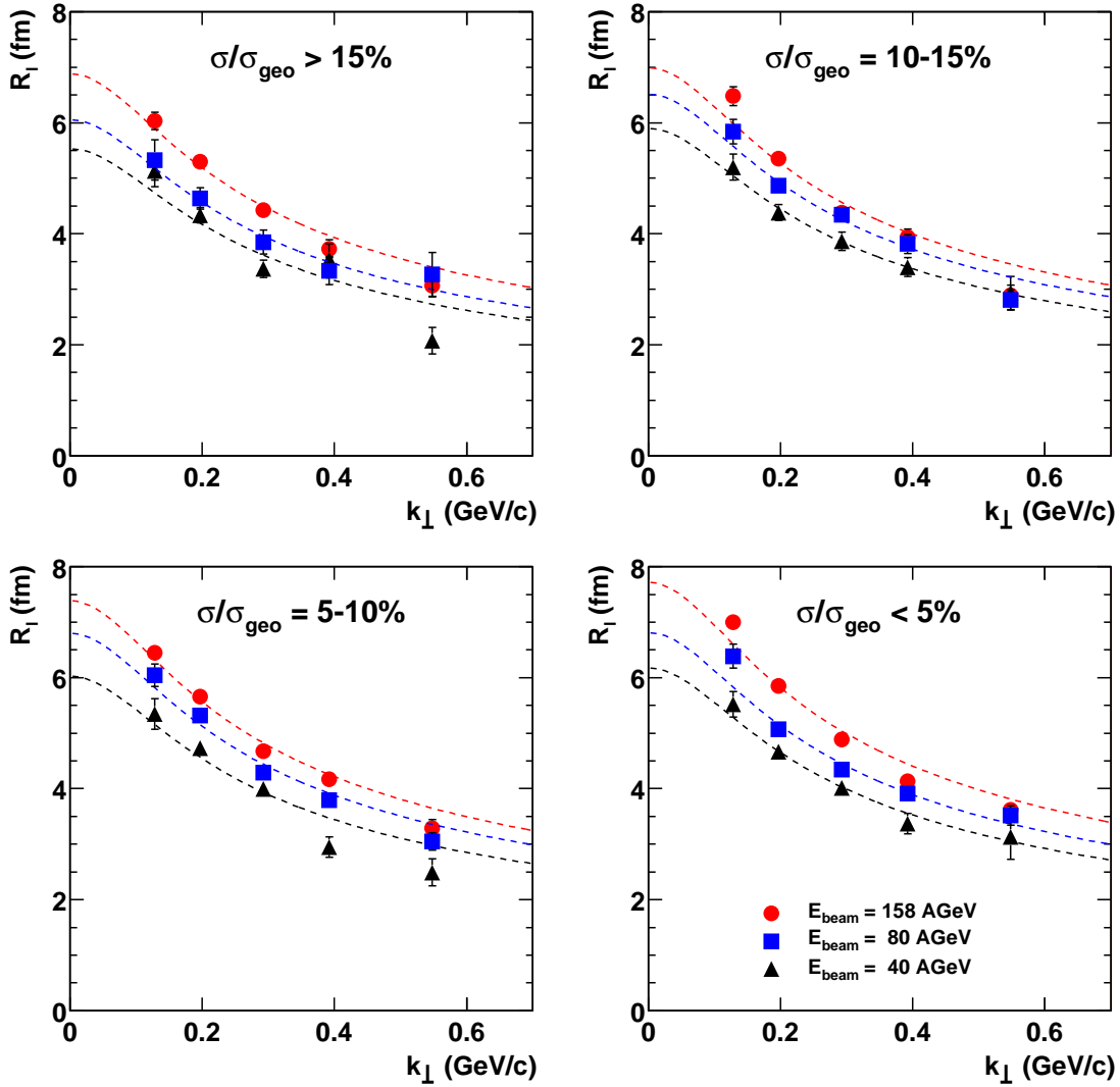
Figure 8.1: R_l for different values of E_{\text{beam}} and different centralities as a function of the mean transverse pair momentum k_{\perp} .
