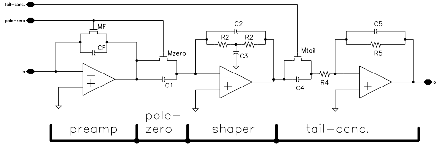
Figure 4.3: Schematic of the charge-sensitive amplifier used in the FEEboards .
