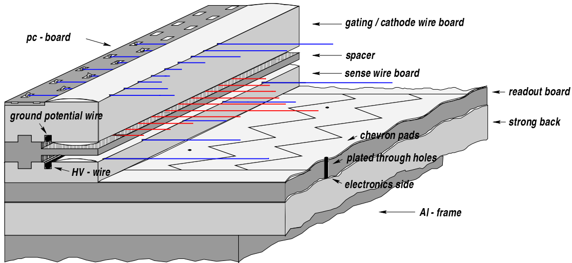
Figure 3.7: Perspective view of the TPC readout chamber.
