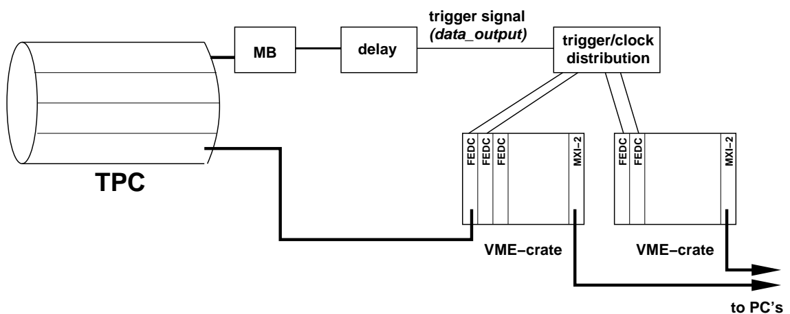
Figure 5.9: FEDC trigger distribution.
