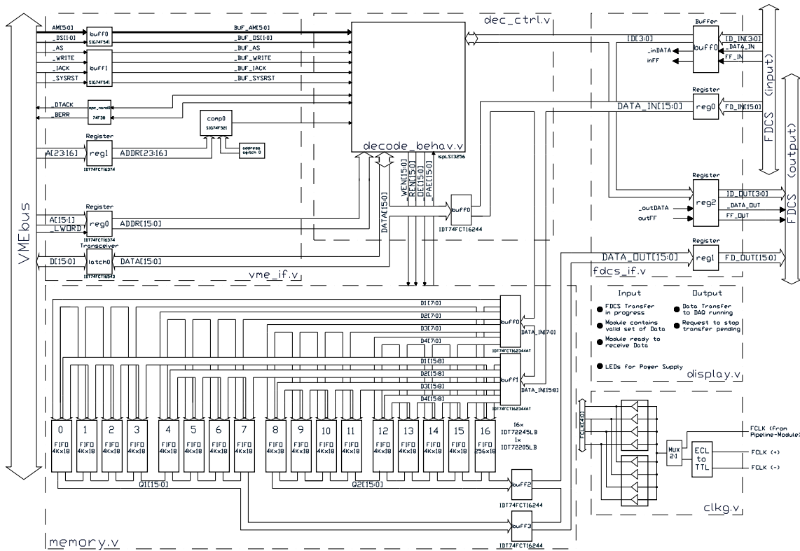
Figure 4.13: Schematic view of the MemoryModule.
