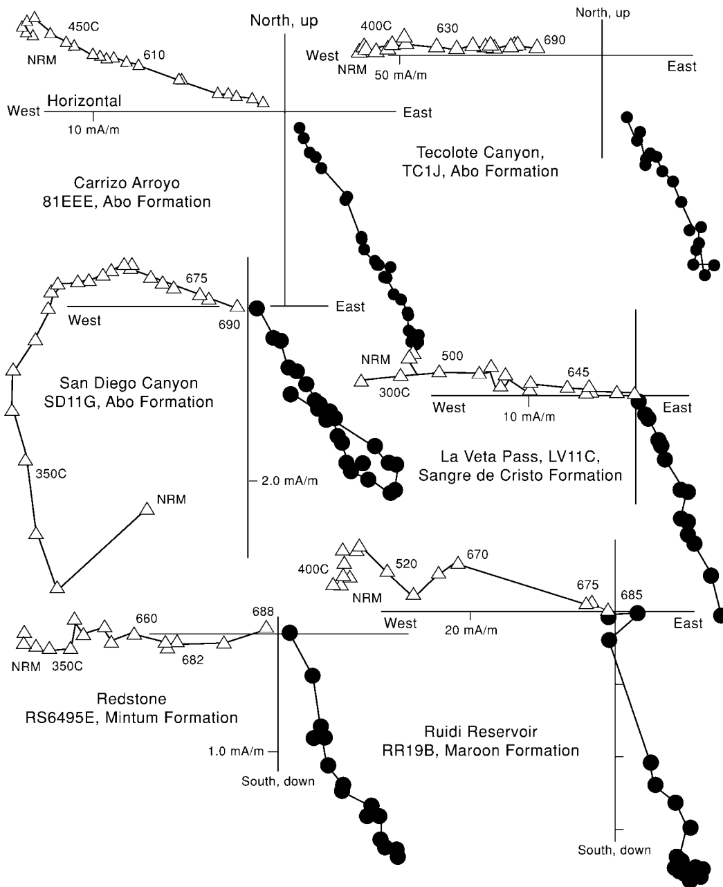
Figure 4. Representative orthogonal demagnetization diagrams from six localities showing typical response to thermal demagnetization of upper Pennsylvanian to lower Permian red beds considered in this study. In each, the endpoint of the magnetization vector is plotted in geographic coordinates onto the horizontal projection ( filled symbols ) and the true vertical projection ( open symbols ). Peak demagnetization temperatures ( ^{\circ}\text{C} ) are given beside the vertical projections. In each example, a magnetization of southeast declination and shallow inclination is isolated over a wide range of laboratory unblocking temperatures.
