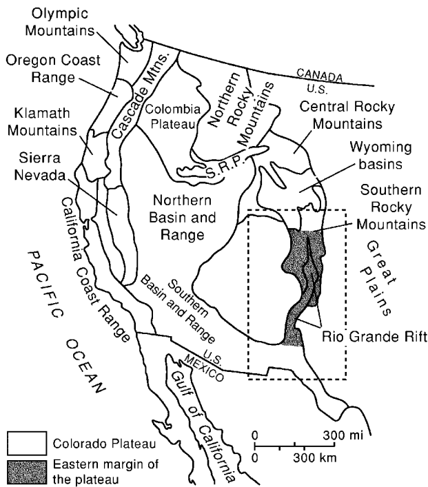
Figure 1. Generalized map of physiographic provinces of the Cordillera of the western United States. The dashed box is the region shown in figures 2, 3, and 5.
