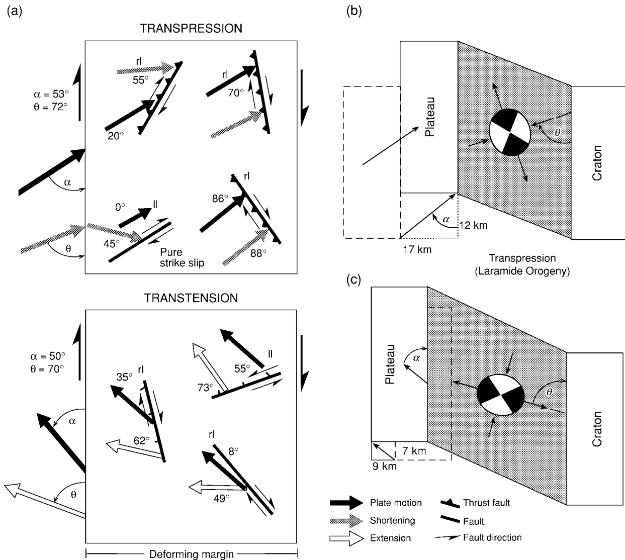
Figure 8. a , Map-view diagram showing the relations between shear zone trends, plate motion direction, and kinematic directions ( s_1 and s_3 ). b , Map-view diagram representing the deforming eastern margin of the Colorado Plateau (gray) located between a fixed craton and an obliquely converging plateau (Laramide orogeny). c , Same as above, except for obliquely diverging plates (Rio Grande rift). Also depicted are the geometric relations used to derive northward translation estimates for both tectonic events.
