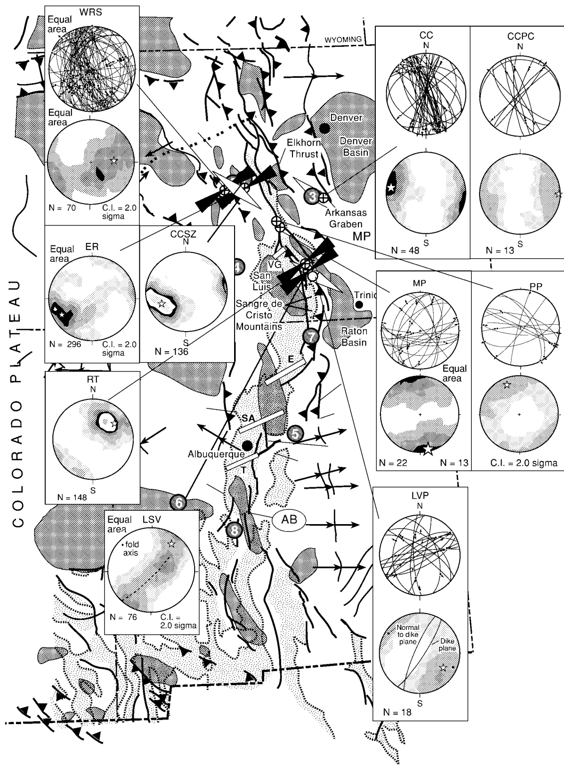
Figure 3. Generalized map and representative equal area projection contour plots of axes associated with Laramide uplift bounding structures and of s_1 associated with Oligocene extensional structures. A star indicates the mean orientation of the shortening and the extension direction, respectively. For equal area projections of actual fault data, the arrows indicate motion of hanging wall. Note that with exception to the White Rock stock data, all of the equal area projections contour plots on the left side of the figure are of s_3 axes, contour plots on the s_1 axes.
