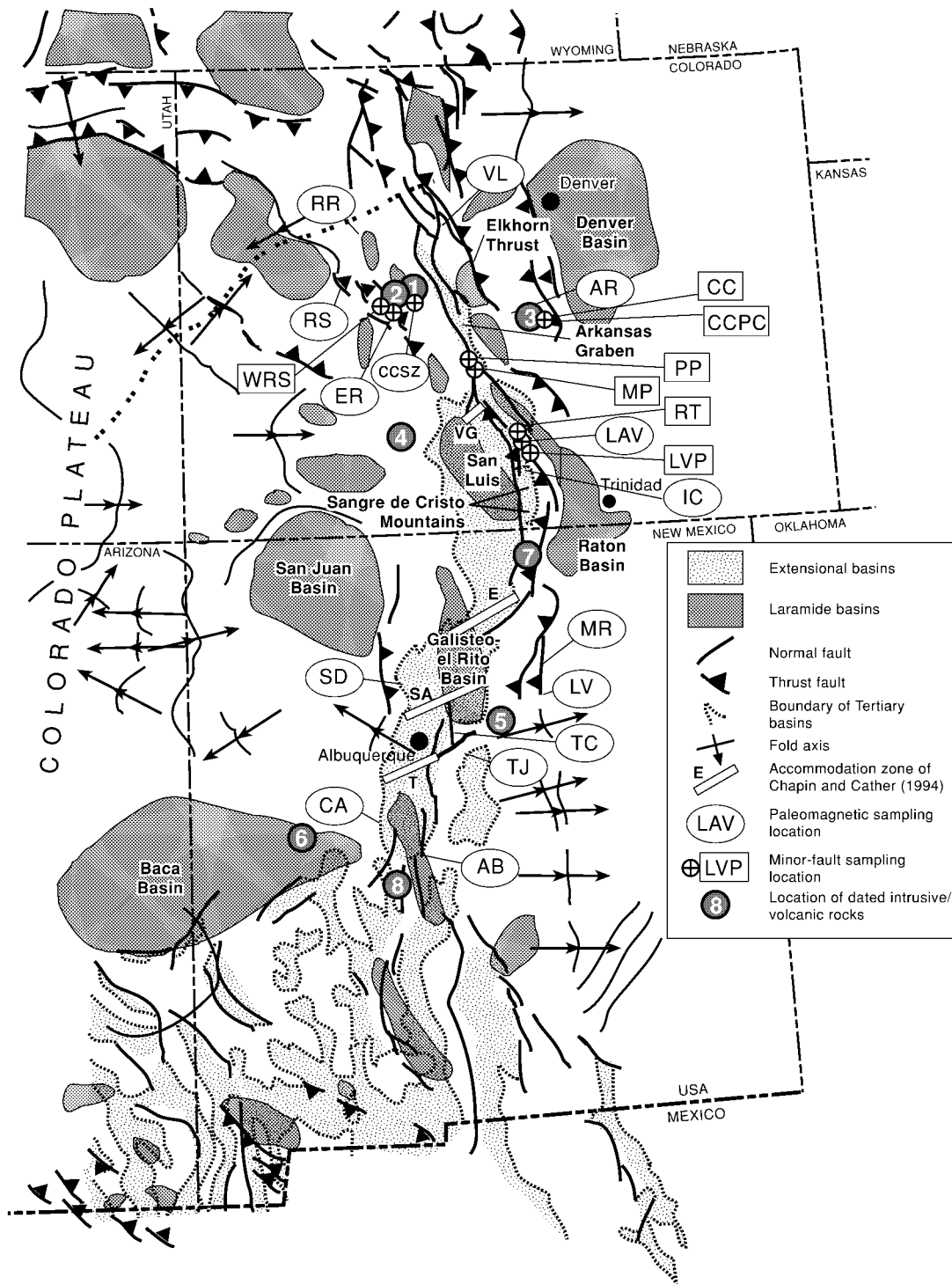
Figure 2. Generalized map of foreland uplifts and basins, and locations of paleomagnetic and minor-fault sampling sites (base map modified from Dickinson et al. 1988). Abbreviations for sites where minor-fault data and paleomagnetic samples were collected are given in tables 1 and 2, respectively. Abbreviations for accommodation zones: VG = Villa Grove; E = Embudo; SA = Santa Anna; T = Tijeras. Numbered locations: 1 = intrusions along the Castle Creek structural zone; 2 = White Rock stock; 3 = Cripple Creek diatreme; 4 = San Juan volcanic field; 5 = Ortiz volcanic field; 6 = Mogollon-Datil volcanic field; 7 = Latir volcanic field; 8 = Socorro volcanic field (see Chapin and Cather 1994 for additional detail).
