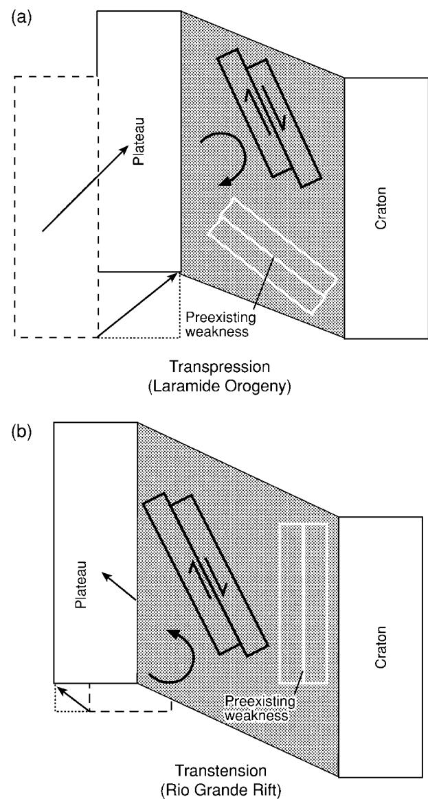
Figure 6. Map-view diagrams showing how individual blocks may rotate during transcurrent deformation. Dashed lines show predeformation position of shear zone elements. a , During transpression, clockwise vertical axis rotation and concomitant dextral simple shear accommodates narrowing of the deforming zone. b , During transtension, anticlockwise vertical axis rotation and concomitant dextral shear accommodates broadening of the deforming zone.
