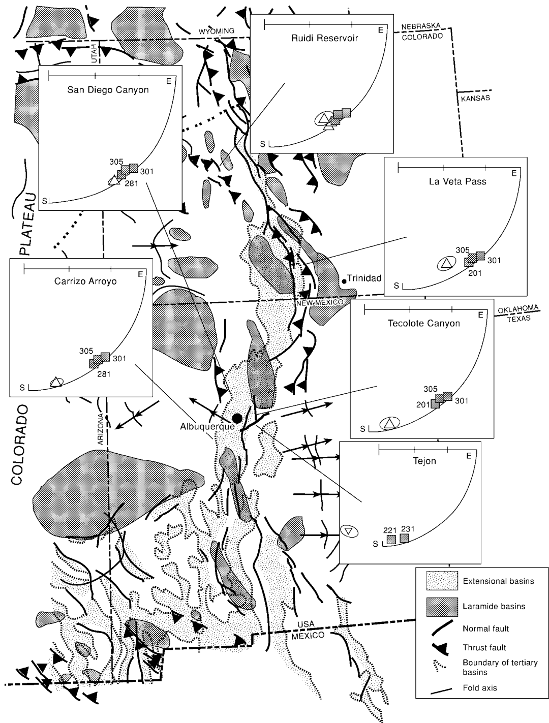
Figure 5. Generalized geologic map of the eastern and the northeastern margin of the Colorado Plateau. Inset diagrams show paleomagnetic data, plotted in the southeast quadrant of an equal area projection, with observed locality means (based on data from several individual sites; see table 3) and the associated reference directions with the inferred age of the reference directions given in millions of years.
