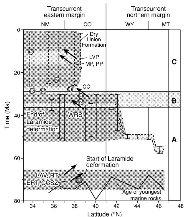
Figure 7. Time versus latitude chart schematically representing the timing of the Laramide orogeny and Rio Grande rifting (modified from Dickinson et al. 1988; Chapin and Cather 1994). Numbered locations refer to igneous events in figure 2. Solid error bars show the range of cessation of sedimentation in transpressional basins. Dashed error bars show the age range of sedimentation of the Santa Fe Formation within basins of the Rio Grande rift. Dashed polygons show the beginning and end of the Laramide as presented in Dickinson et al. (1988). A , Laramide orogeny and continued northeast-directed convergence. B , Transition phase lasting 1–6 m.yr., in which extension is likely given the widespread occurrence of volcanic activity. C , Rio Grande rift marked by the onset of sediment accumulation (Santa Fe Formation); rifting may continue to the present. The rift may terminate near the Arkansas graben (Dry Union Formation) because the trend of bounding structures changes to the northwest and becomes subparallel to the calculated divergence direction.
