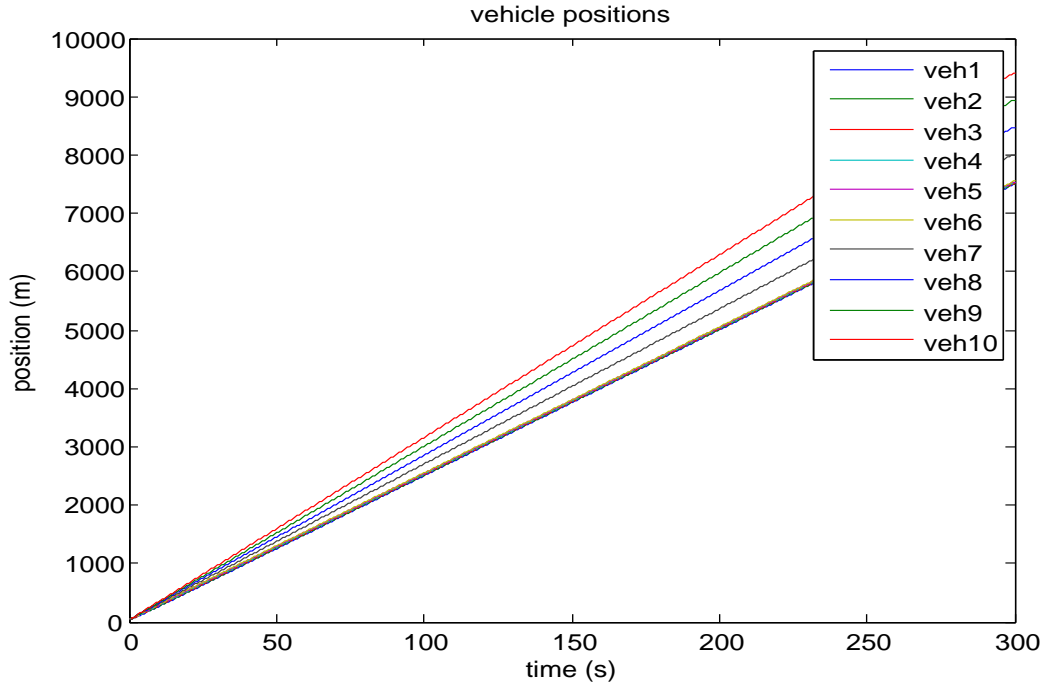
Fig. 4.11: Due to false data injection, vehicles are no longer string stable.
