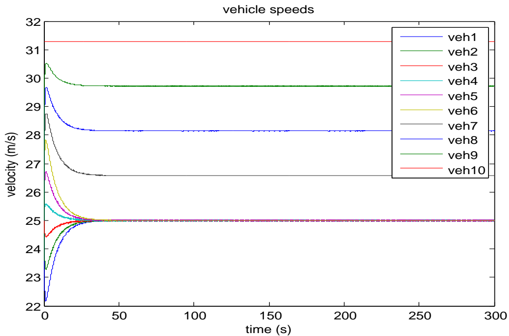
Fig. 4.10: Due to false data injection, vehicles do not attain the desired velocity.
