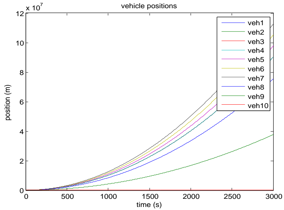
Fig. 7.3: The vehicles are absolutely not string stable.
