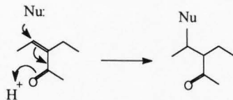
Fig. I-3. Possible reaction mechanisms between macrocyclic unsaturated diester PAs with a nucleophilic atom ( Nu ).
