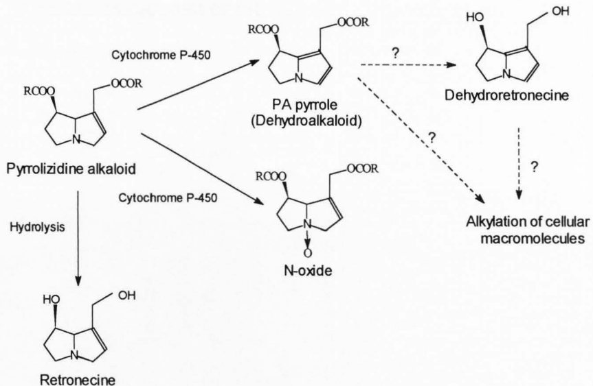
Fig. 1-2. Known and postulated metabolic pathways of pyrrolizidine alkaloids.
