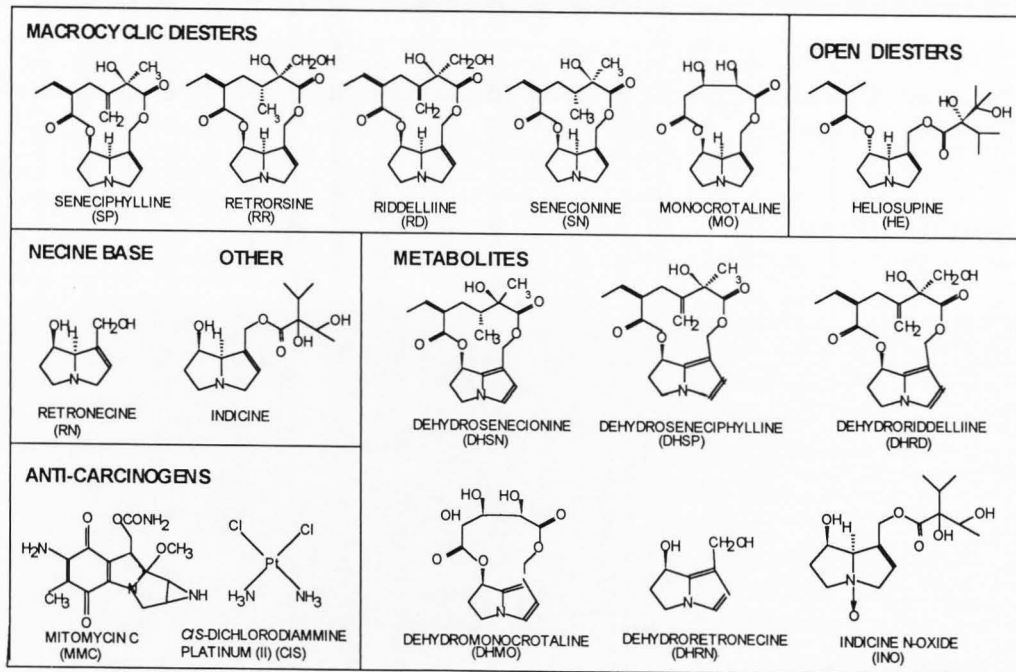
Fig. M -1. Chemical structures of pyrrolizidine alkaloids and anti-carcinogens examined in this dissertation.
