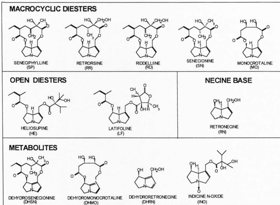
Fig. II-1. Chemical structures of pyrrolizidine alkaloids and their metabolites examined in this dissertation.
