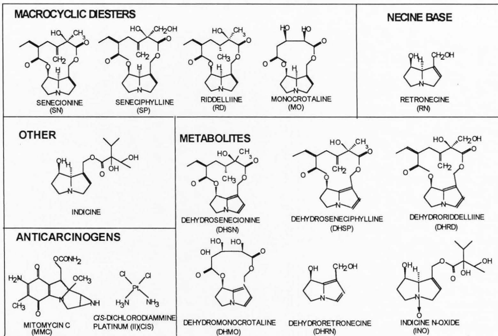
Fig.III-1. Chemical structures of PA, pyrrolic PAs, and anti-carcinogens examined in this dissertation.
