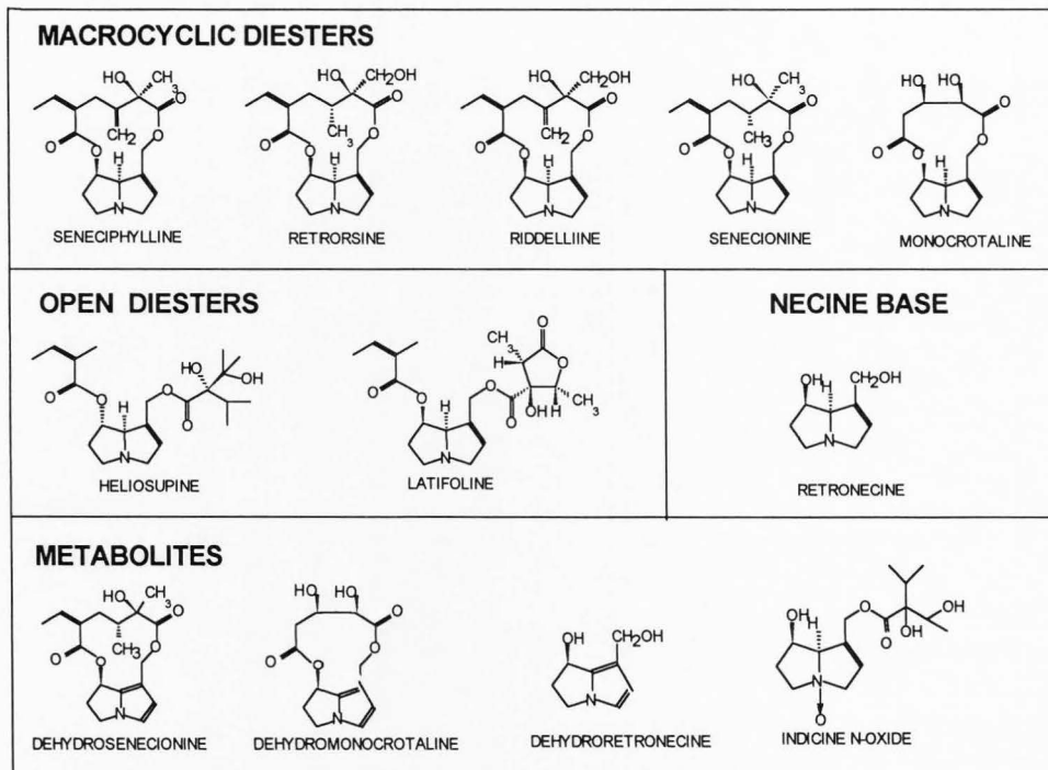
Fig. I-1. Chemical structures of pyrrolizidine alkaloids and their metabolites.
