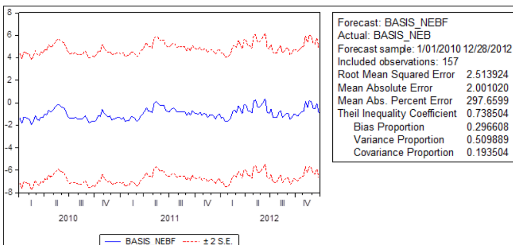
Figure 47. Lag-52 Singular forecast, Nebraska live cattle steers
