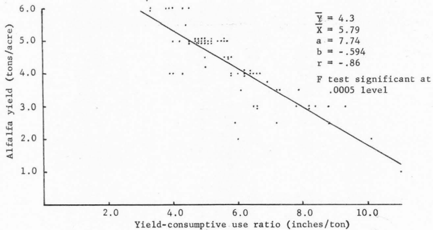
Figure 2. Relationship of alfalfa yield to yield-consumptive use ratio, Sevier Valley, 1962.
