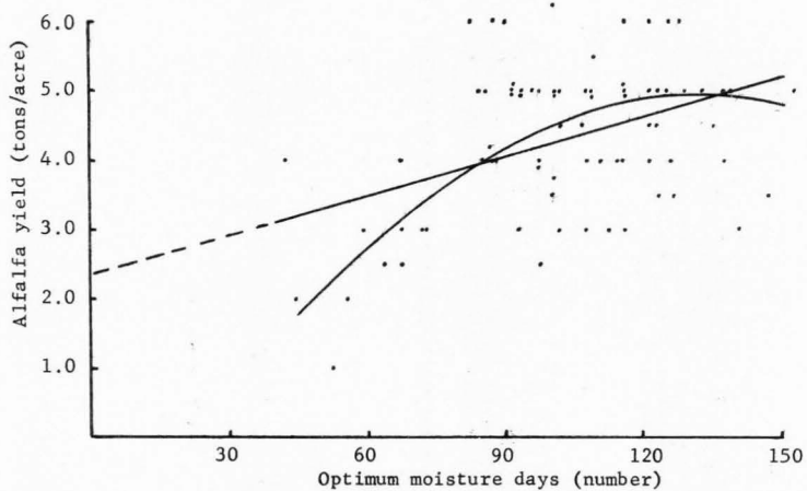
Figure 5. Alfalfa yields and optimum moisture days in the growing season on sample fields, Sevier Valley, 1962.
