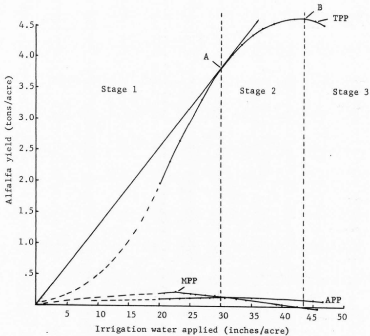
Figure 10. Alfalfa yield and irrigation water use relationship for Sevier Valley, 1962.
