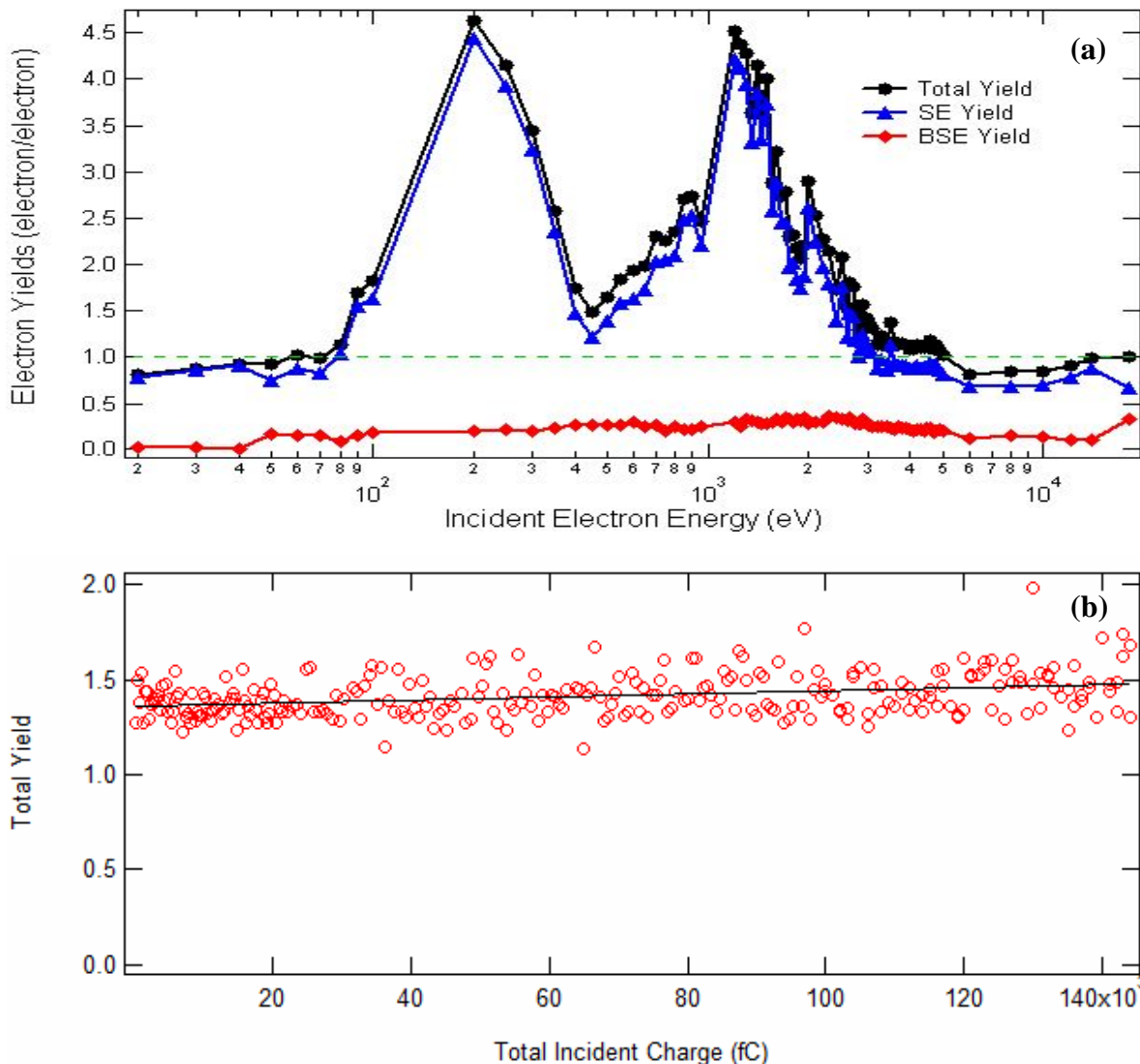
Figure 3. (a) Electron induced yield curve from 99.9% pure alumina 1 mm thick. Note the severe depression, due to positive surface charging, in the yield where E_{\max} should be. (b) Yield measured on 1 mil thick Kapton with 400 eV incident pulses. Discharge methods were employed after each pulse and no significant charging was observed over the entire dose. The slight rise in the yield is due to instrumental drift over the 6 hours needed to collect this data set.
