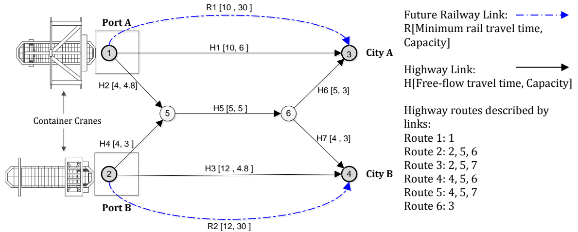
Fig. 5.3 A small example network
