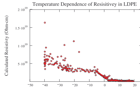
Fig. 7. Calculated resistivity as a function of temperature in 25 μm LDPE from -40.0(±0.5)°C to 20(±0.5)°C.
