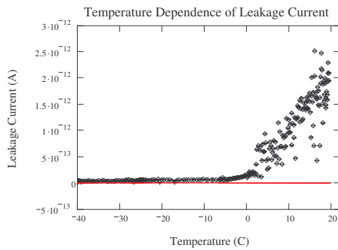
Fig. 6. Leakage current through 25 μm LDPE sample from -40.0(±0.5)°C to 20(±0.5)°C. The straight line seen below the collected data is the base noise level of the system while all equipment is powered on but no measurements are being taken.
