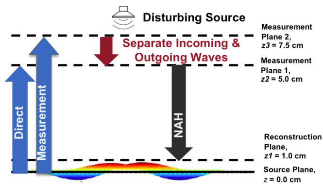
Figure 1: A diagram of the process to find the acoustic properties of a source by making a measurement in a reverberant field. A direct pressure measurement is made on two separate planes, the incoming and outgoing waves are separated, then NAH is performed to propagate back to the source.
