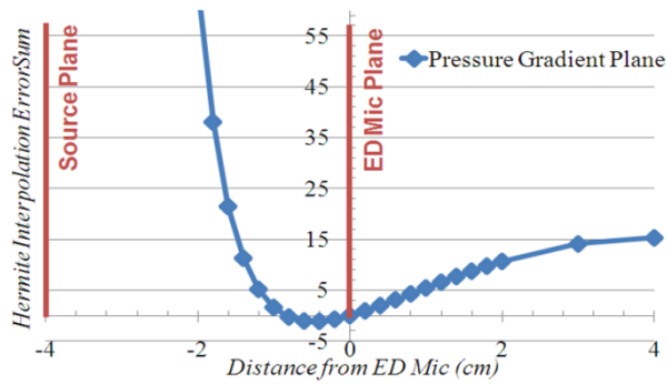
Figure 4: The error associated with using a separate plane's pressure gradient as an approximation. The pressure gradient was approximated on a plane that varied from two cm closer to the source to four cm further away from the source. As can be seen, when the gradient measurement is approximated on a plane close to the actual plane, very little error is introduced. The test frequency shown here is 300 Hz.
