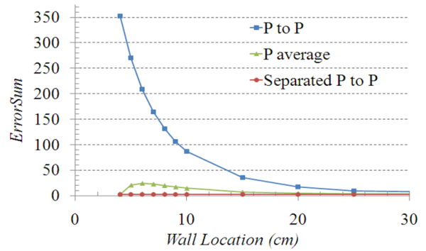
Figure 5: The error associated with performing NAH when a reflection is present. The reflective wall is varied from 4 to 30 cm. Free-field NAH shown in blue shows a large error when the reflective wall is close to the measurement plane. When the spatial Fourier transform technique is used before NAH, shown in red, there is minimal error in the NAH reconstruction regardless of how strong the reflection is. An additional separation technique not described in this paper is shown in green.
