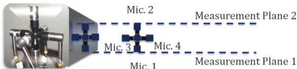
Figure 3: The six-microphone probe allows pressure measurements to be made simultaneously on two separate planes, while the four microphones between the planes are used to calculate the pressure gradient.
