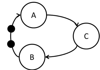
(c) Valid H-SDF initial condition with two tokens in the loop
