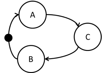
(b) Valid H-SDF initial condition with one initial token in the loop
