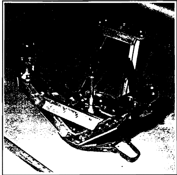
Figure 2 Ejection Mechanism for NUSAT. Source: NASA.
