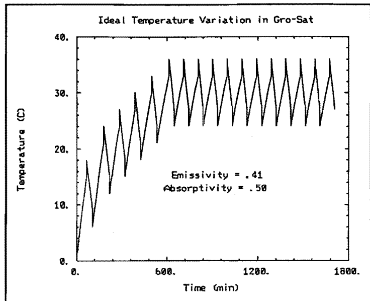
Figure 3 Satellite Temperature Variation
