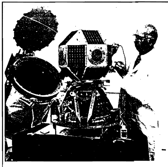
Figure 1 NUSAT. Source: NASA.
