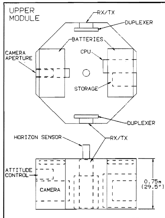
Figure 5.1 Top and Side View of Upper Module Structure of Satellite.
