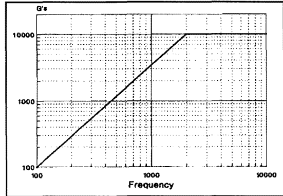
Figure 5 Shock Spectrum
