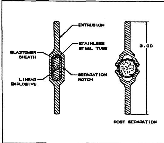
Figure 4 Frangible Joint Before and After Function
