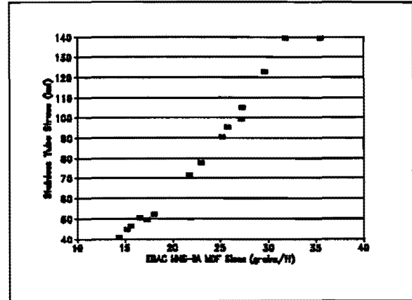
Figure 8 Stress in 0.049 inch Stainless Steel Tube
