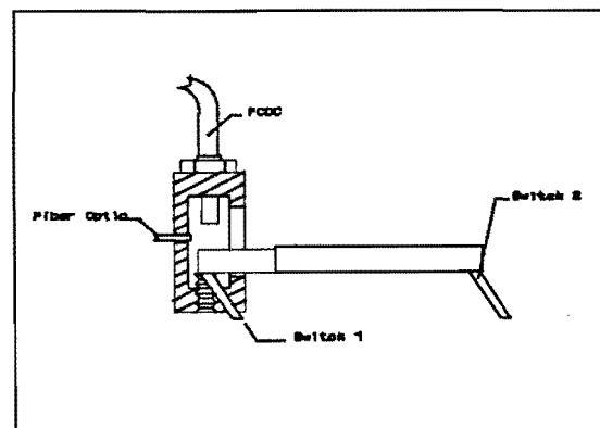
Figure 6 Initiation Test Fixture and Switches
