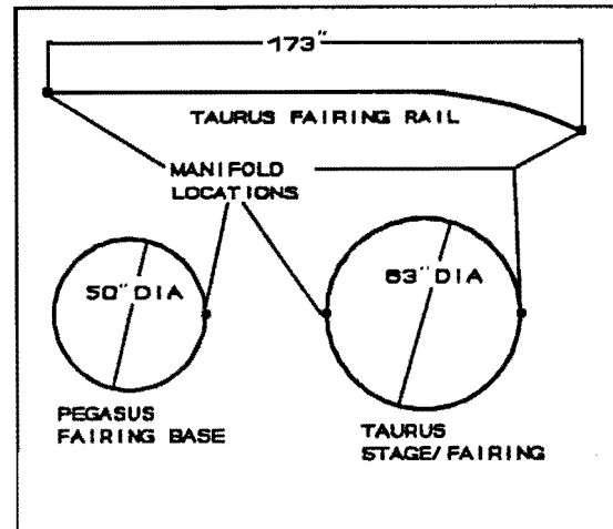
Figure 11 Joint Shapes
