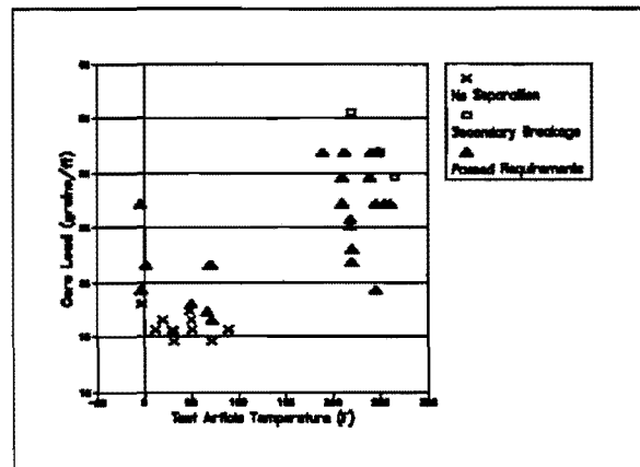
Figure 9 Results of Extrusion Tests as a Function of Temperature
