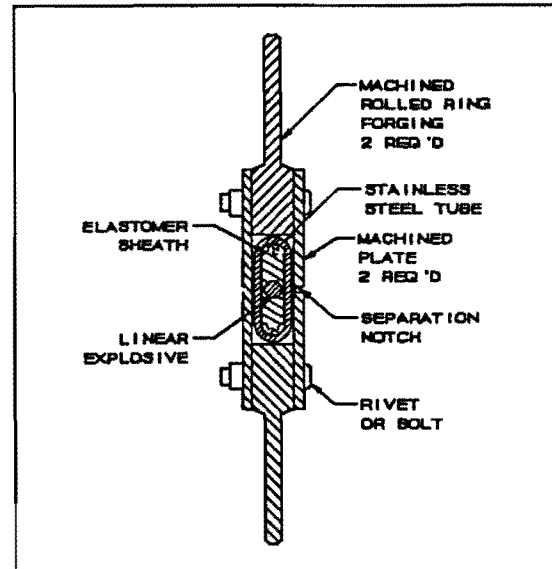
Figure 3 Typical Solid Joint
