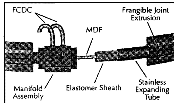
Figure 1 Frangible Joint
