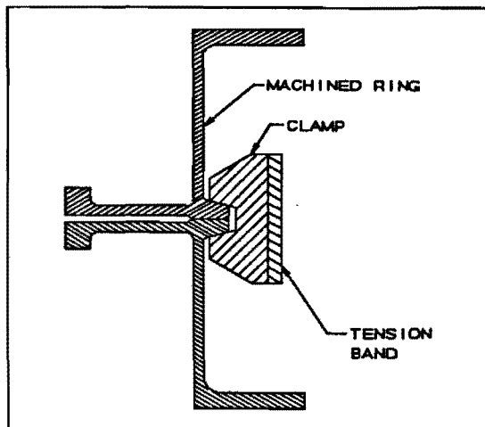
Figure 2 Typical V-Band
