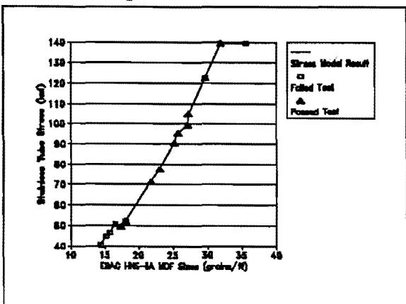
Figure 10 Comparison of Theory and Test Results
