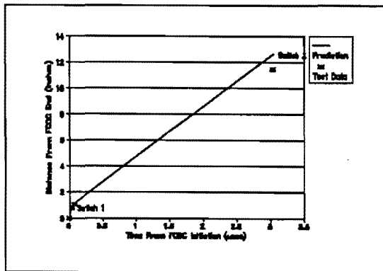
Figure 7 Initiation Test Data
