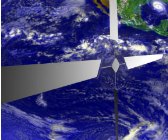
Figure 6. Solar Blade Heliogyro Nanosatellite
