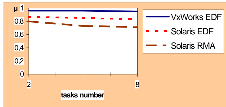
Figure 4 : Evolution of the Utilization Factor in Function of the Number of Tasks
