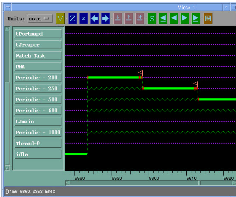
Figure 3 : Java Tasks Scheduled by the VxWorks Kernel
